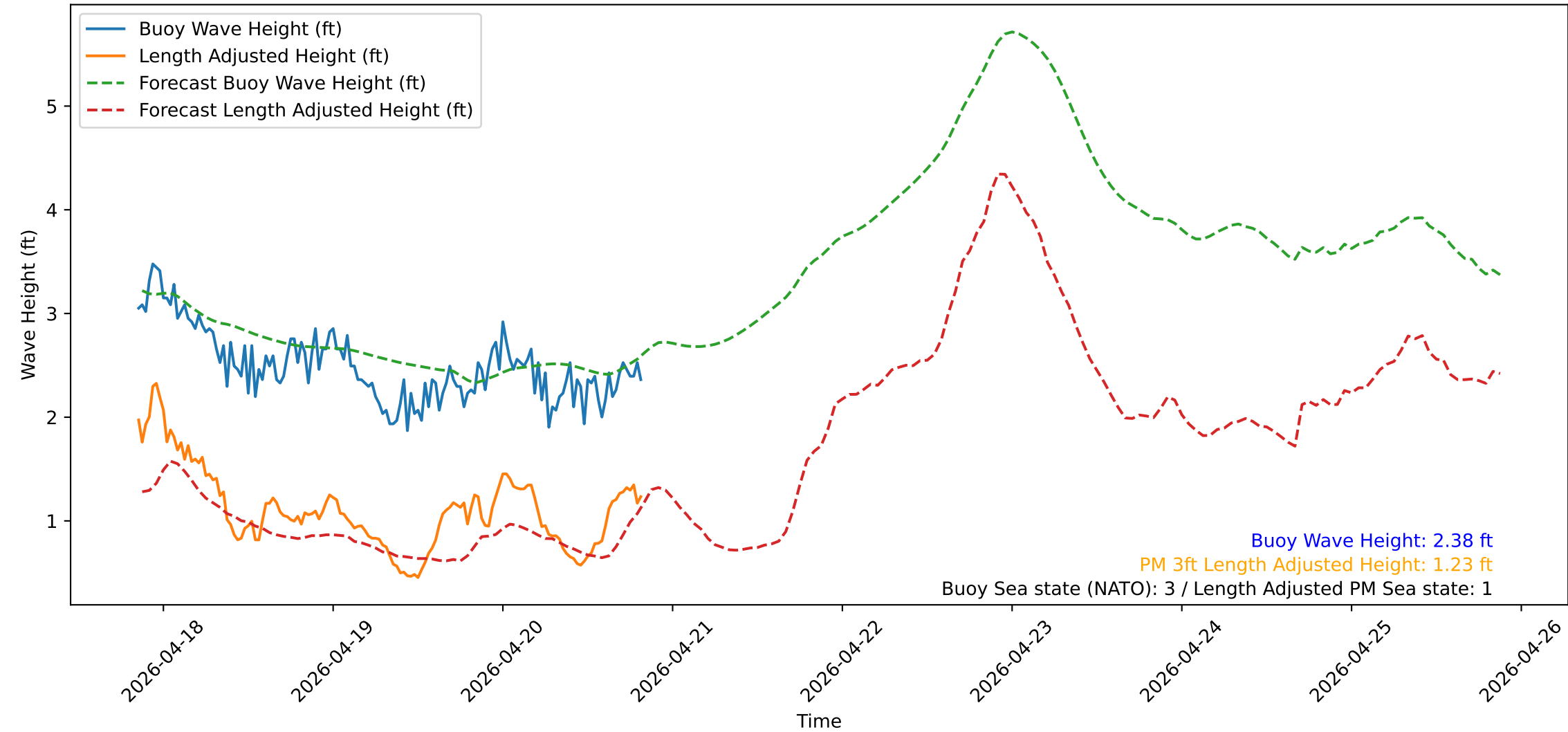
Wave Heights over Time for Green Beach at 2026-04-20 20:31:13
