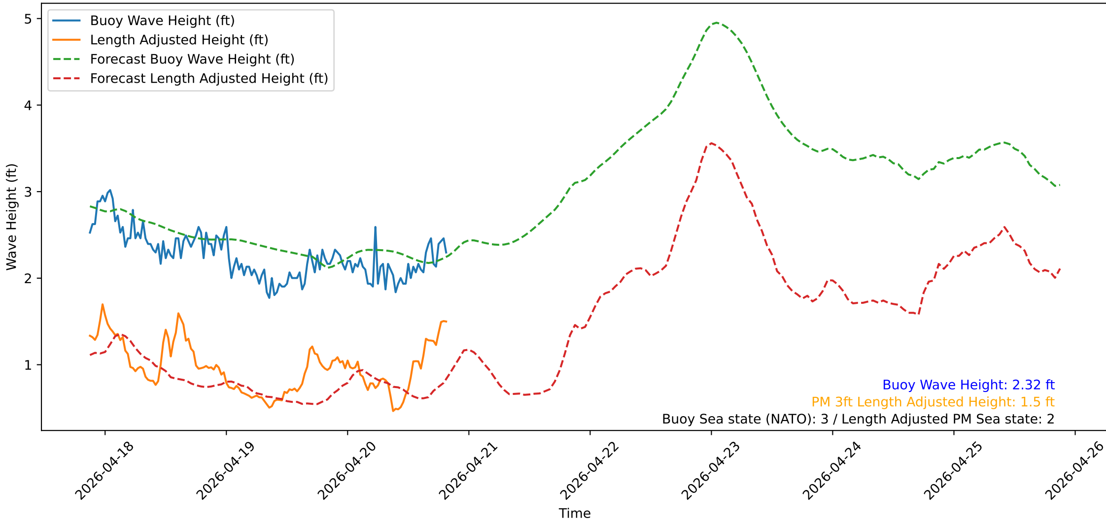
Wave Heights over Time for Red Beach at 2026-04-20 20:30:51
