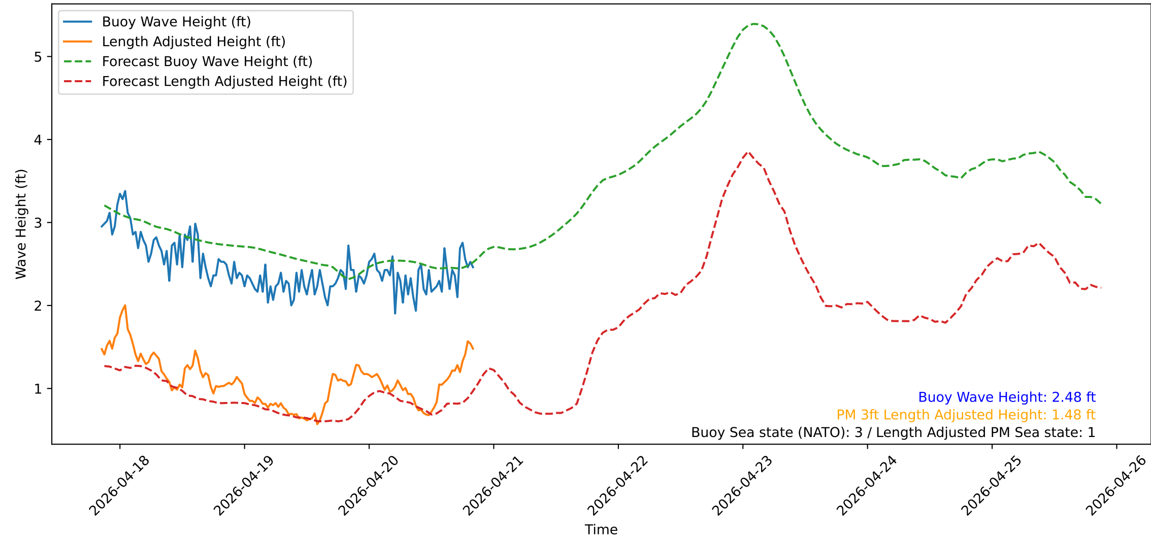
Wave Heights over Time for Oceanside Harbor at 2026-04-20 20:30:32
