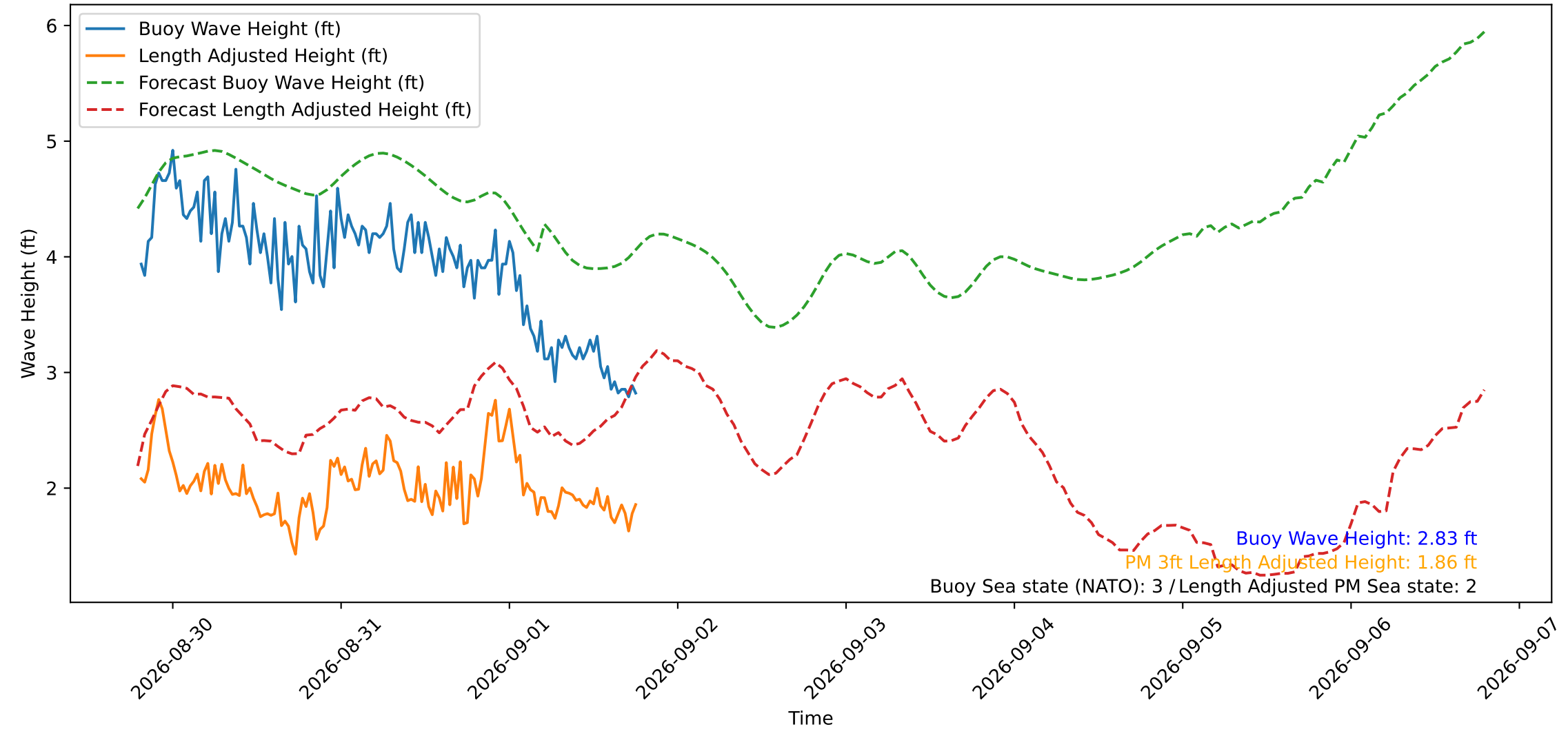
Wave Heights over Time for Green Beach at 2026-09-01 19:01:12
