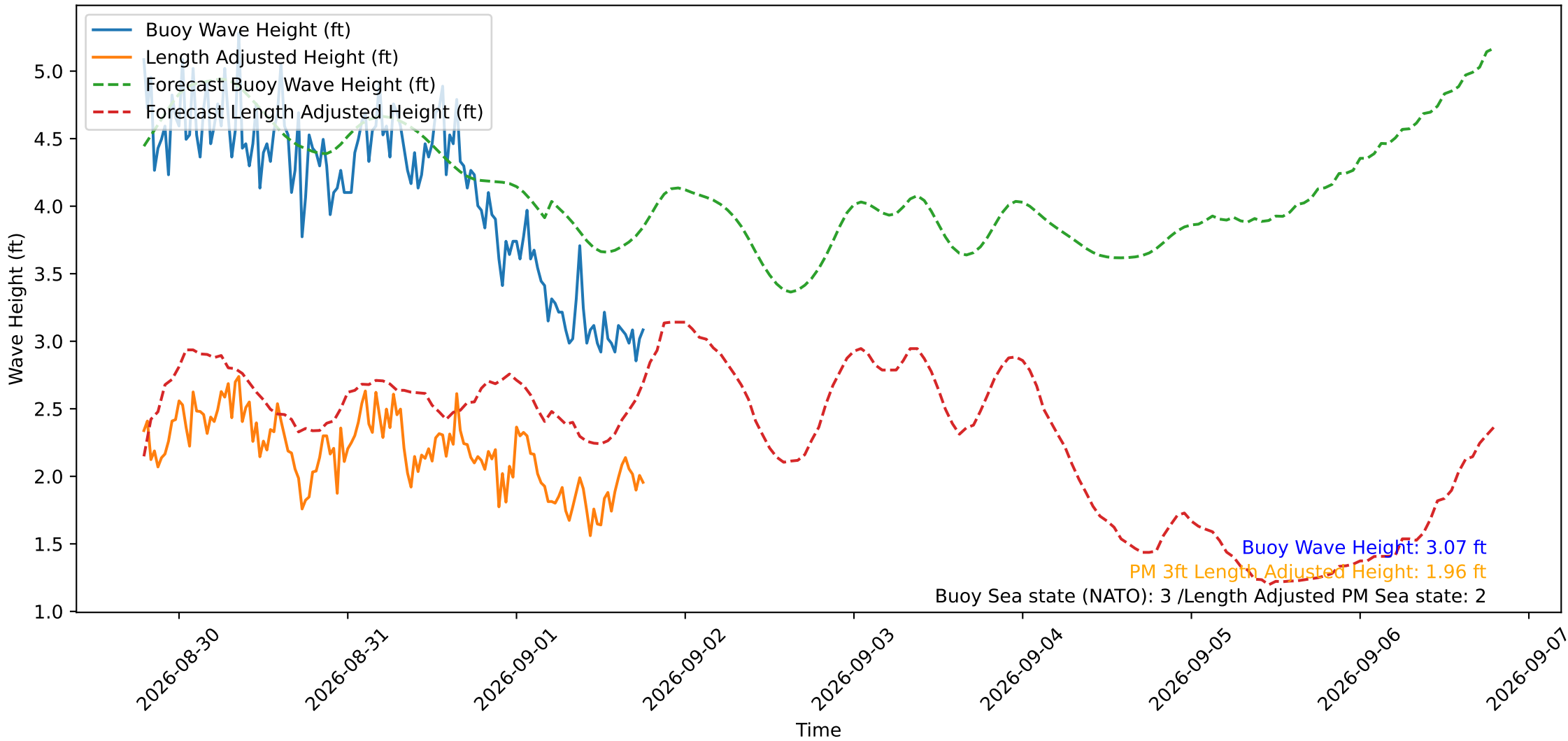
Wave Heights over Time for Oceanside Harbor at 2026-09-01 19:00:30
