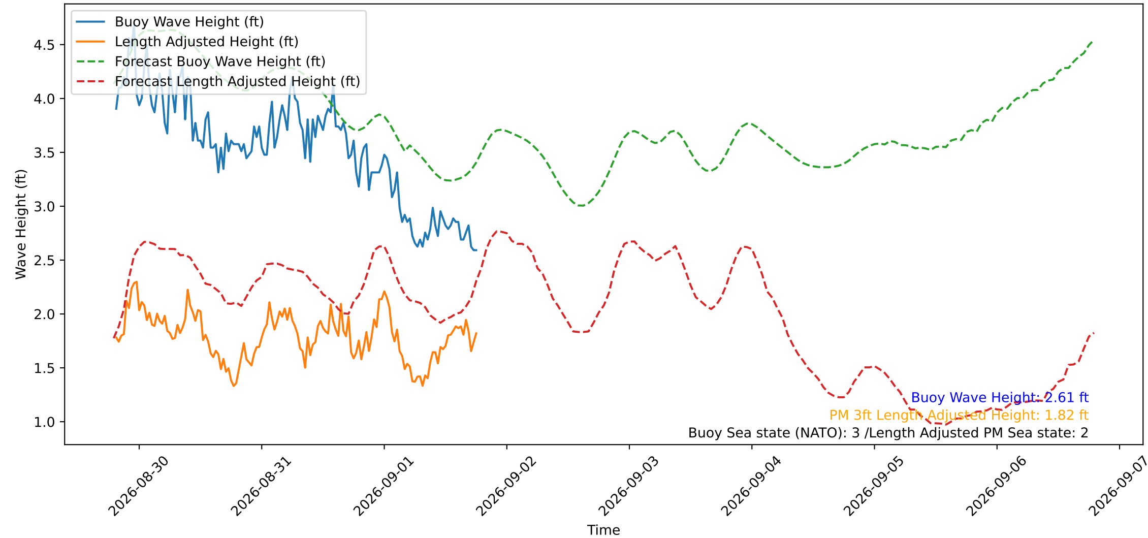
Wave Heights over Time for Red Beach at 2026-09-01 19:00:49
