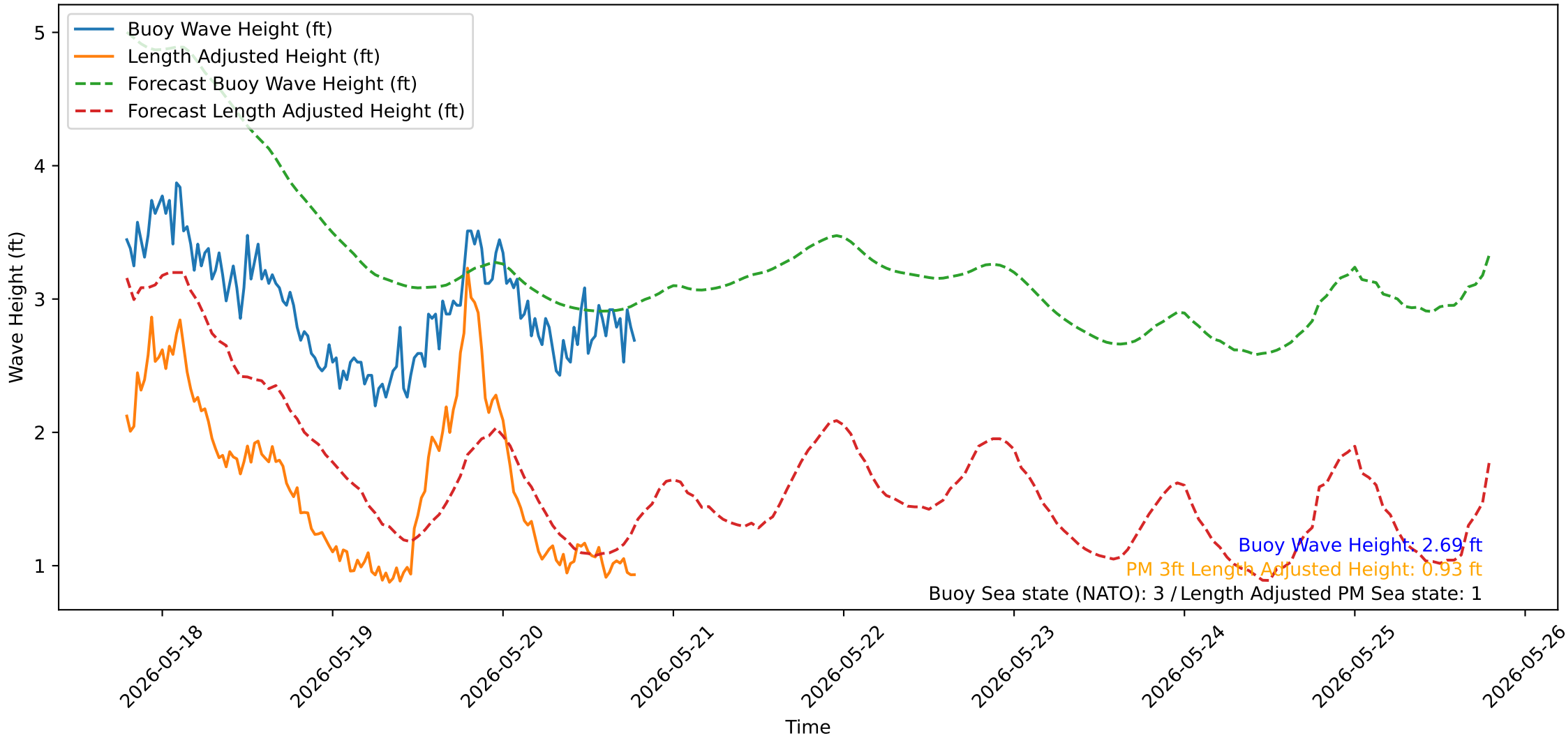
Wave Heights over Time for Oceanside Harbor at 2026-05-20 19:10:31
