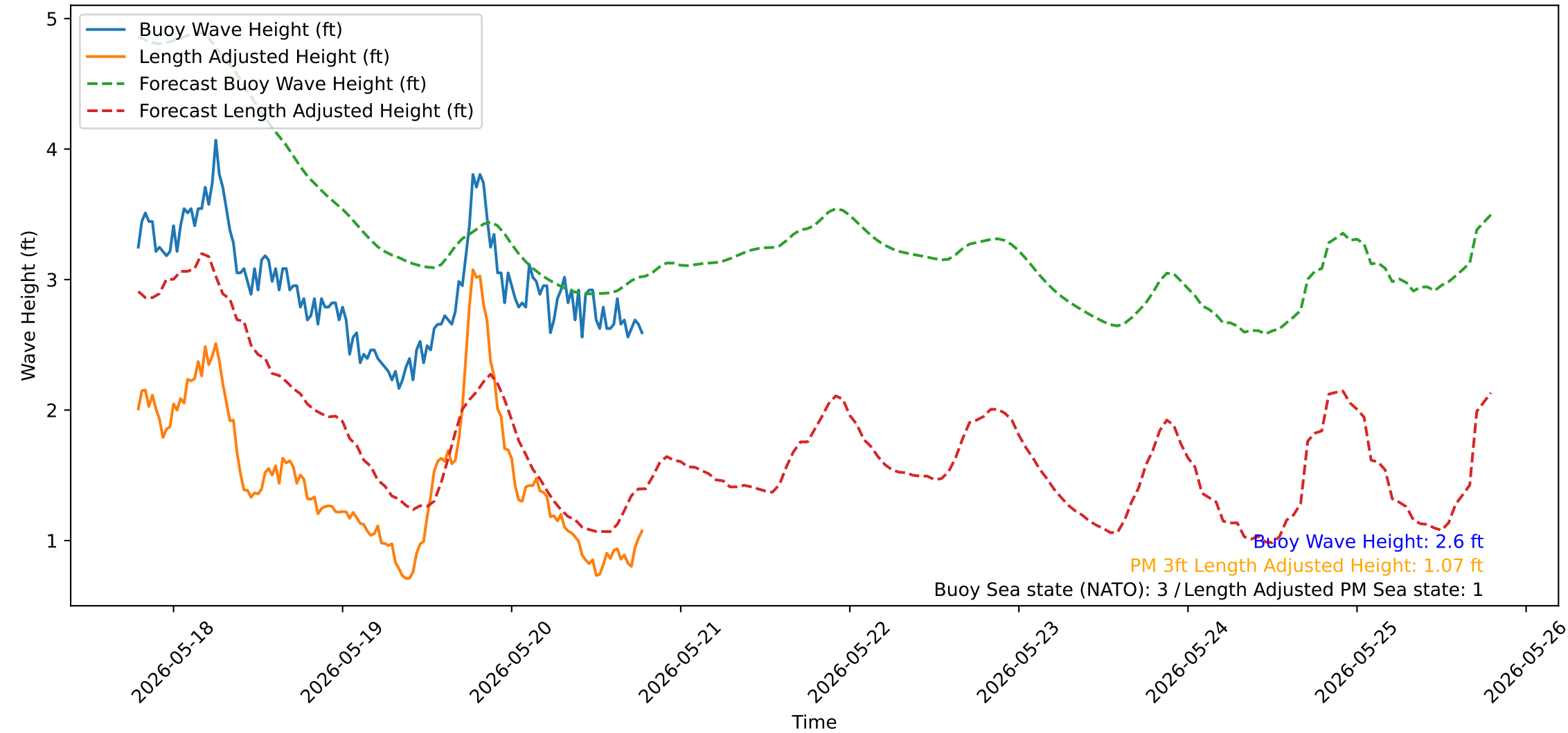
Wave Heights over Time for Green Beach at 2026-05-20 19:11:14
