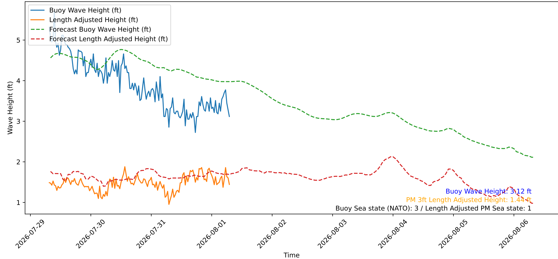
Wave Heights over Time for Oceanside Harbor at 2026-08-01 07:30:27
