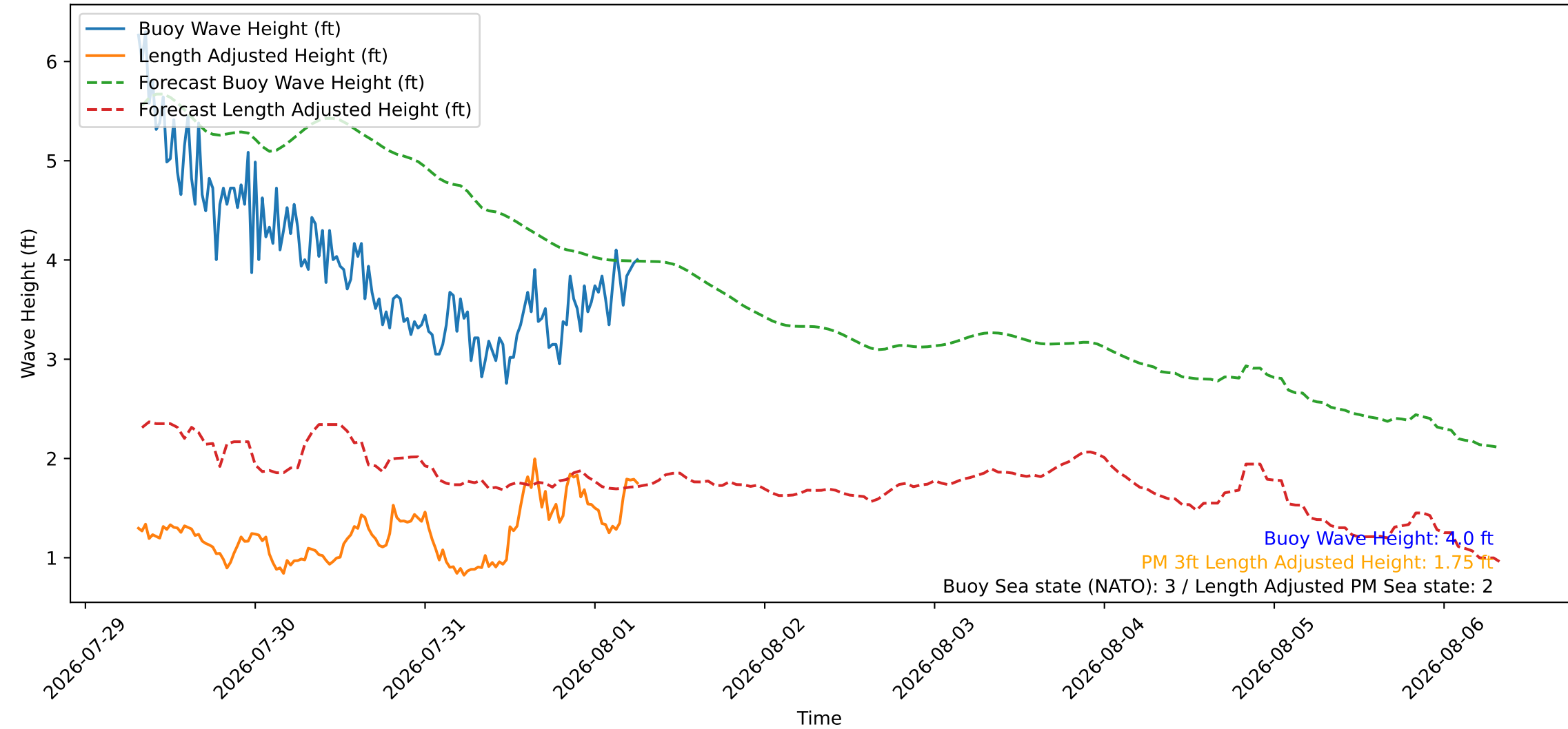
Wave Heights over Time for Green Beach at 2026-08-01 07:31:08
