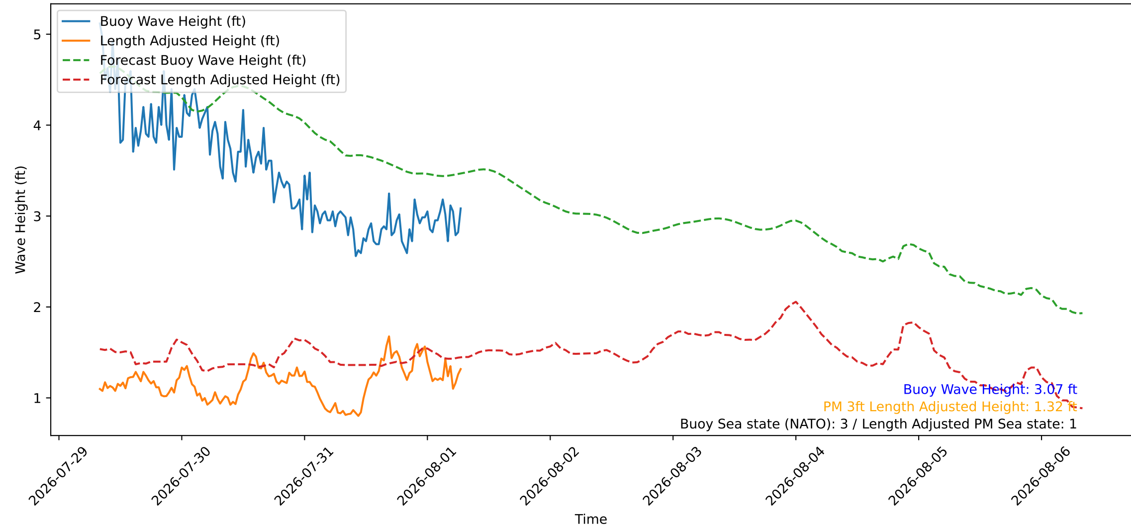
Wave Heights over Time for Red Beach at 2026-08-01 07:30:46
