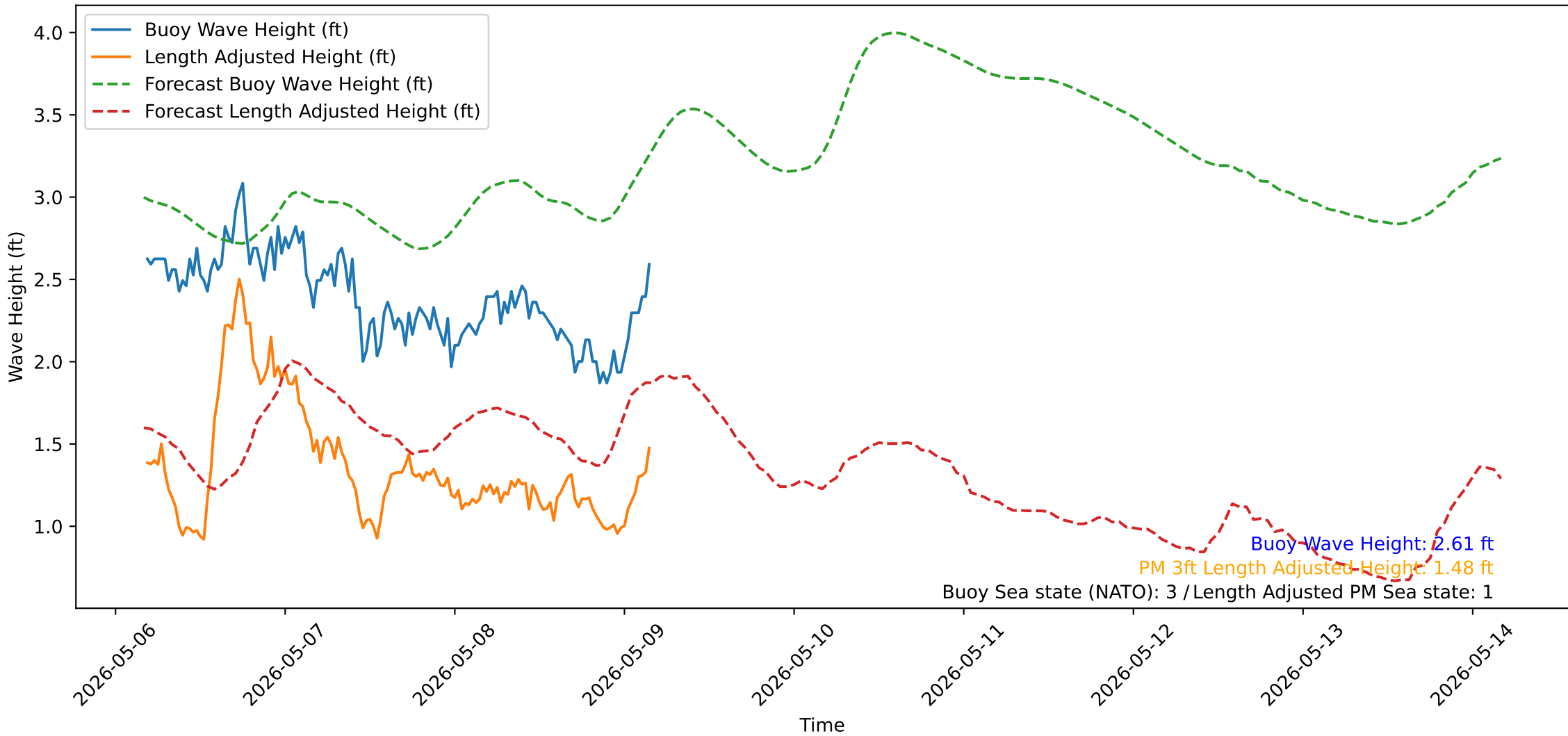
Wave Heights over Time for Oceanside Harbor at 2026-05-09 04:20:31
