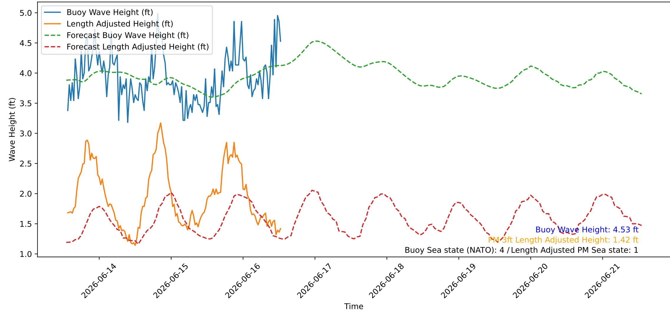
Wave Heights over Time for Oceanside Harbor at 2026-06-16 13:20:26
