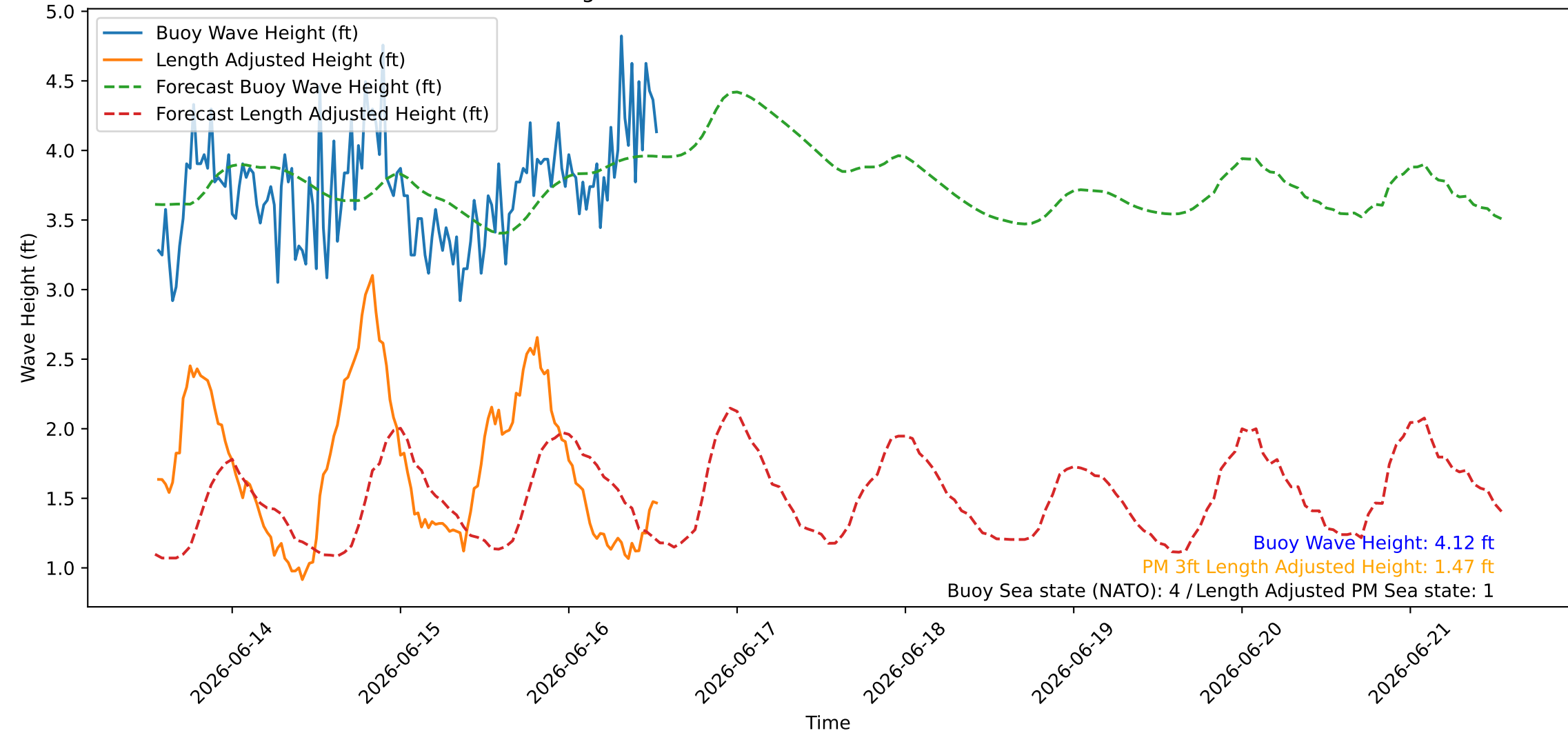
Wave Heights over Time for Red Beach at 2026-06-16 13:20:46
