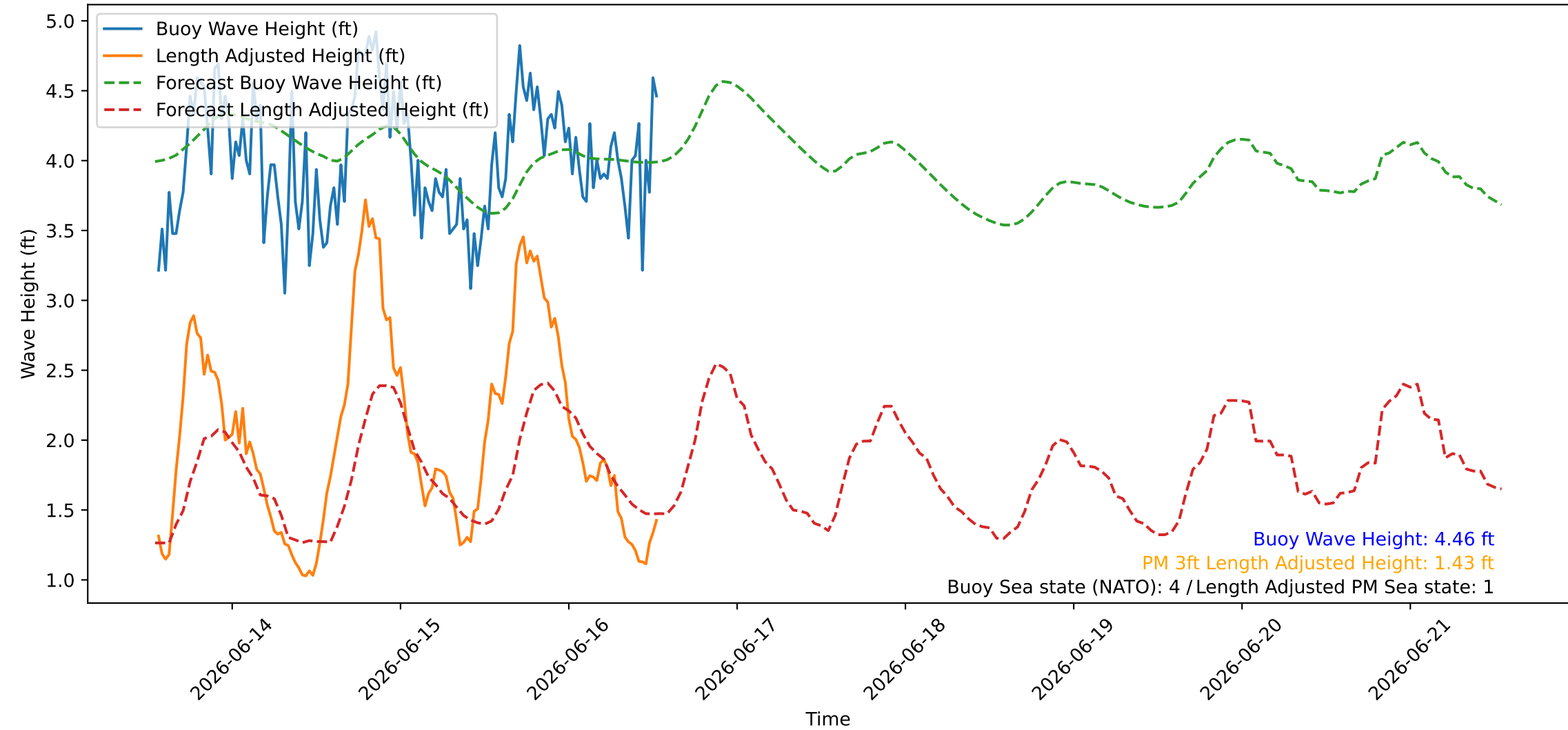
Wave Heights over Time for Green Beach at 2026-06-16 13:21:08
