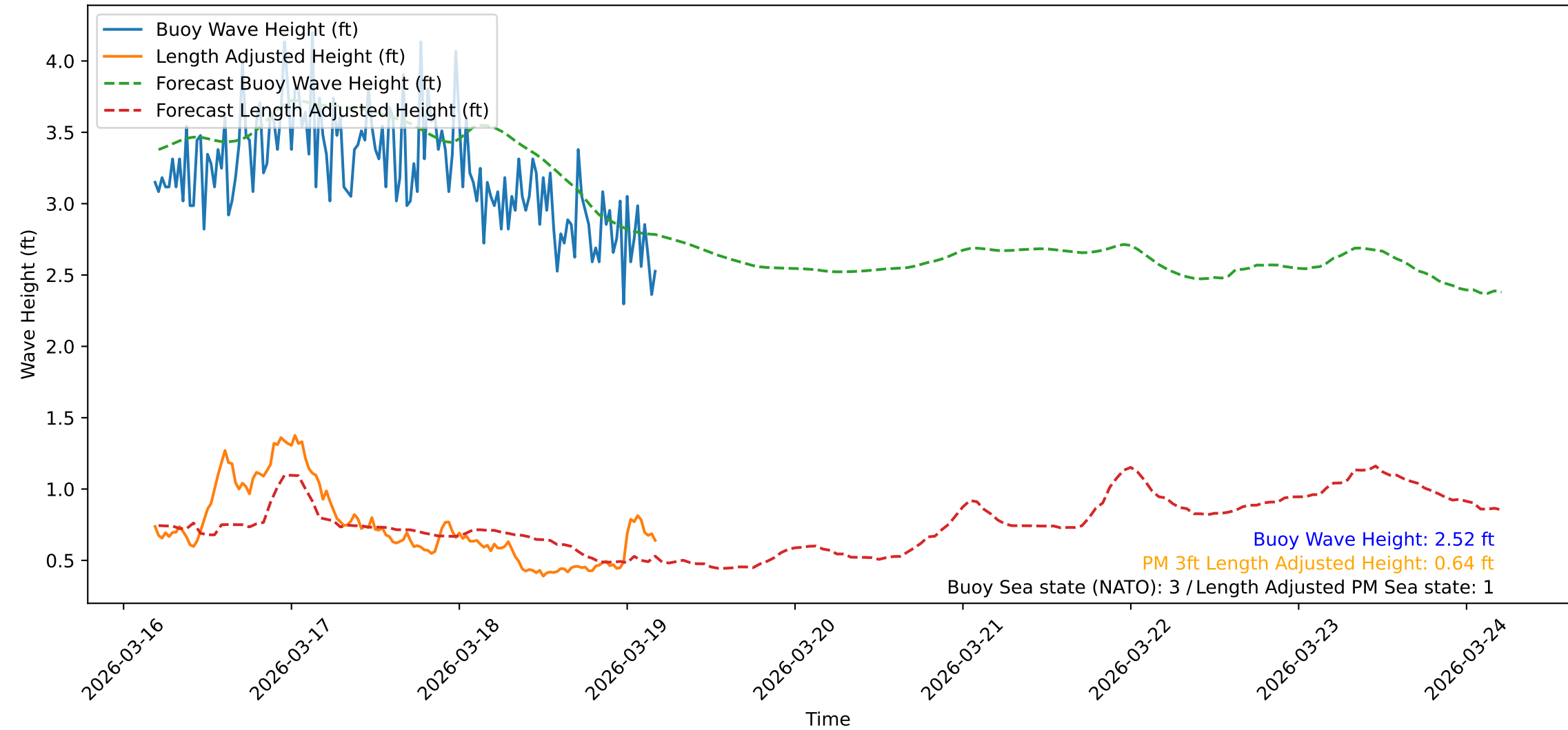
Wave Heights over Time for Green Beach at 2026-03-19 04:41:10
