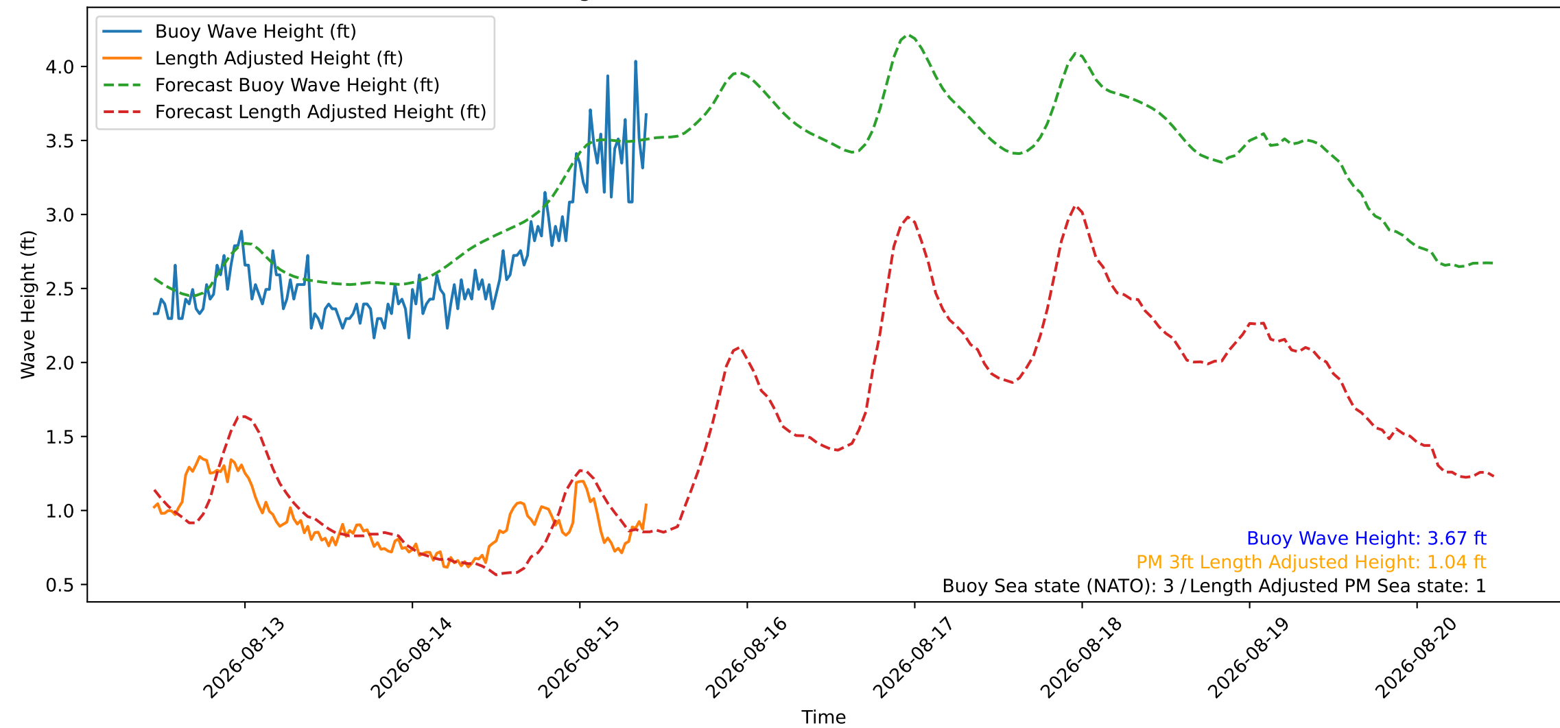
Wave Heights over Time for Red Beach at 2026-08-15 10:30:46
