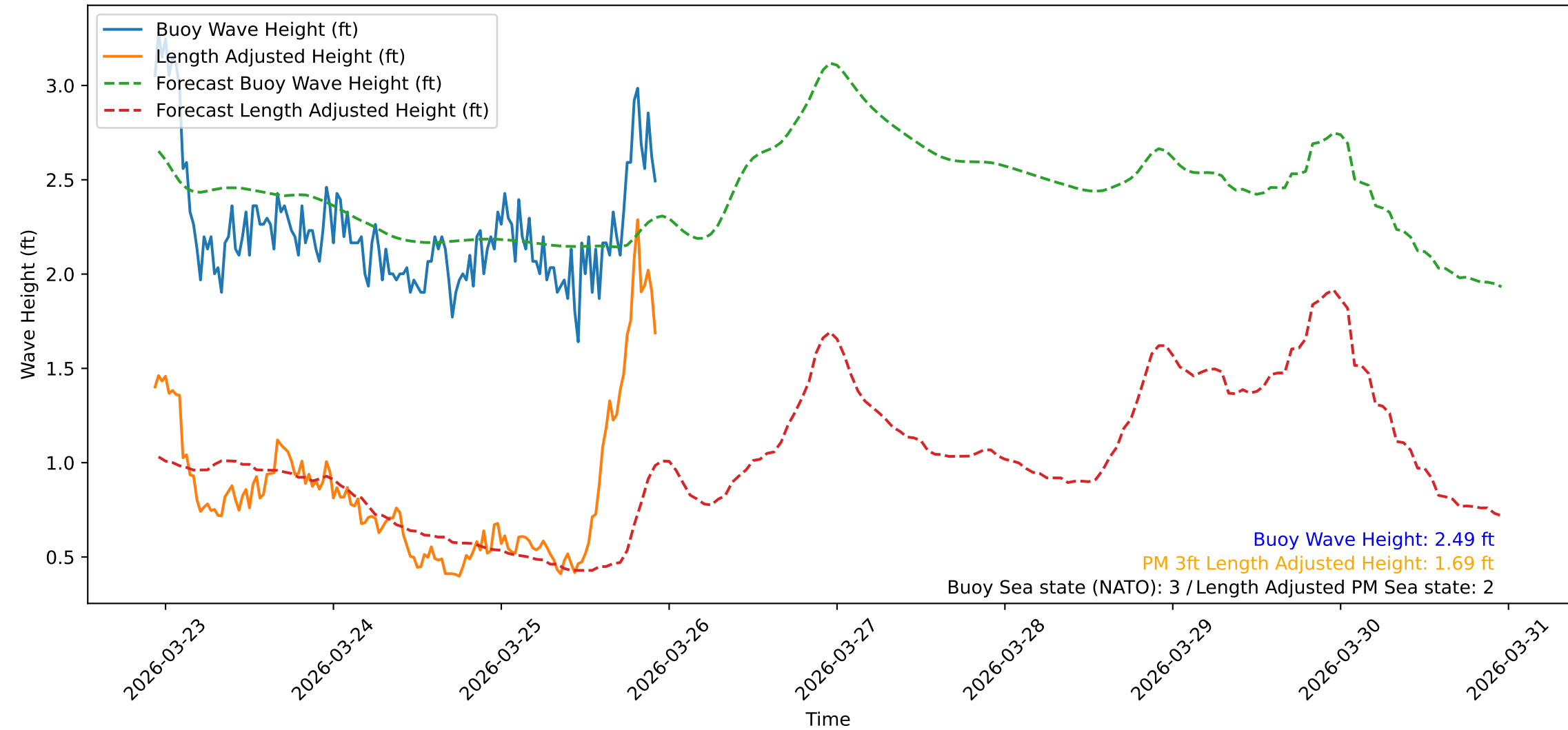
Wave Heights over Time for Green Beach at 2026-03-25 22:41:10
