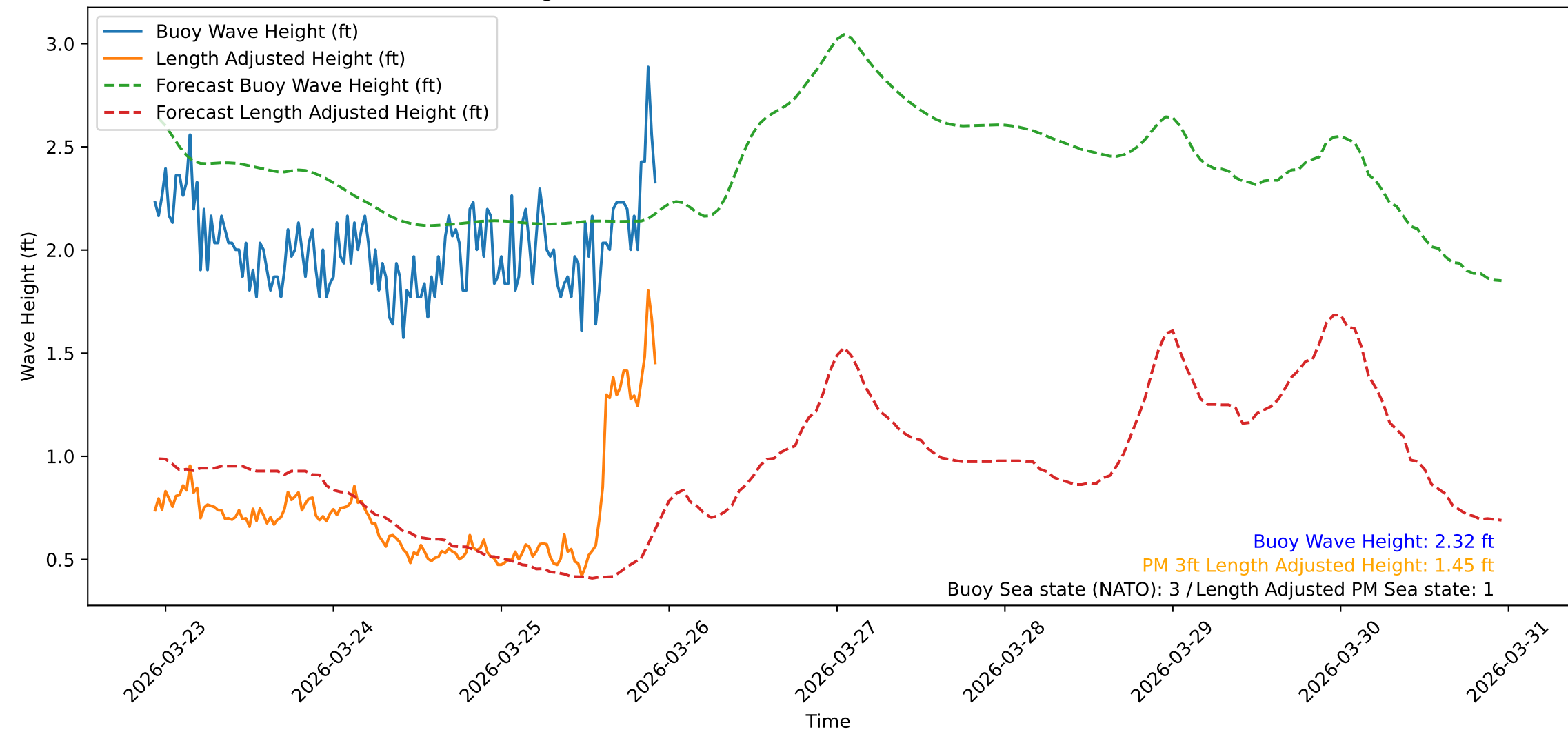
Wave Heights over Time for Oceanside Harbor at 2026-03-25 22:40:32
