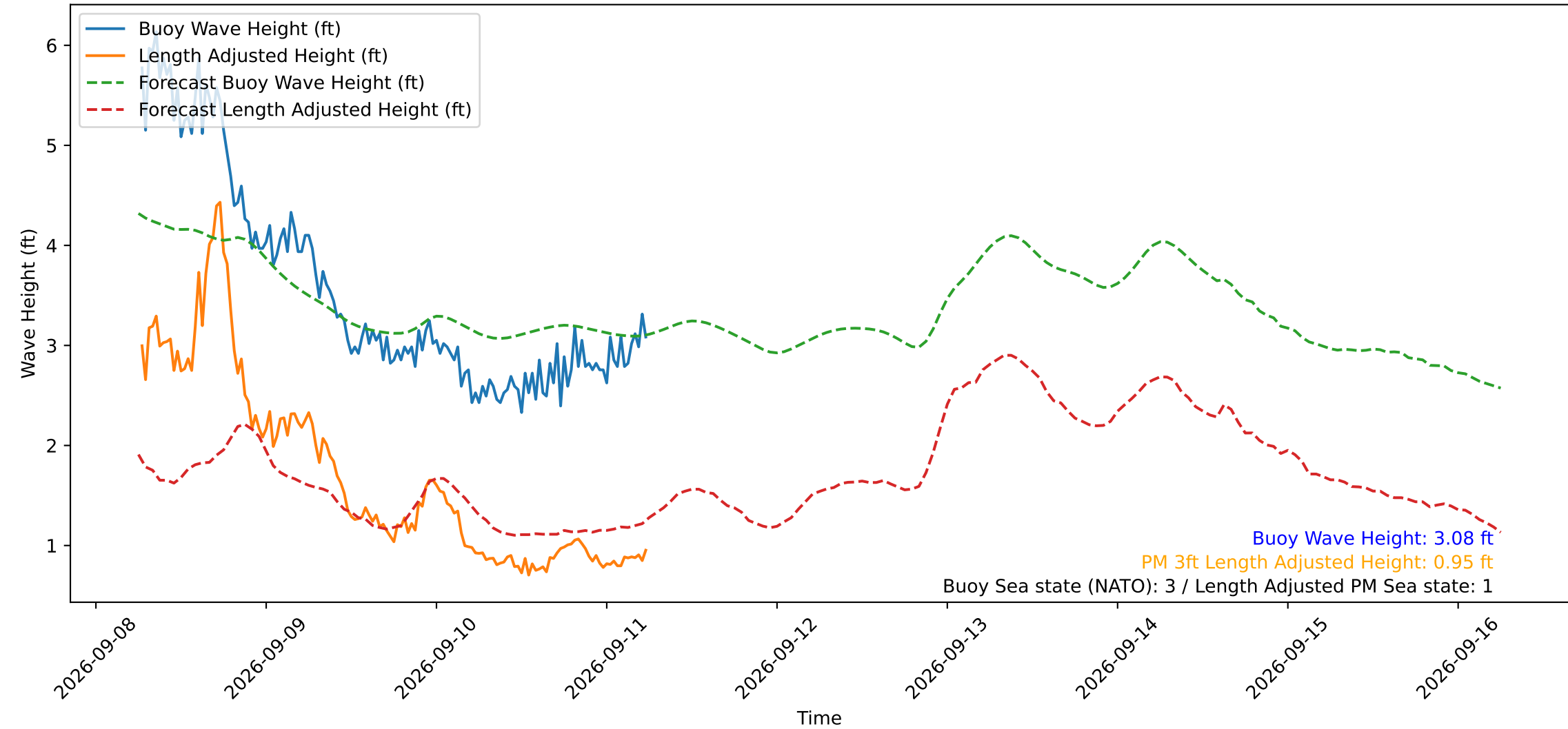
Wave Heights over Time for Red Beach at 2026-09-11 06:10:49
