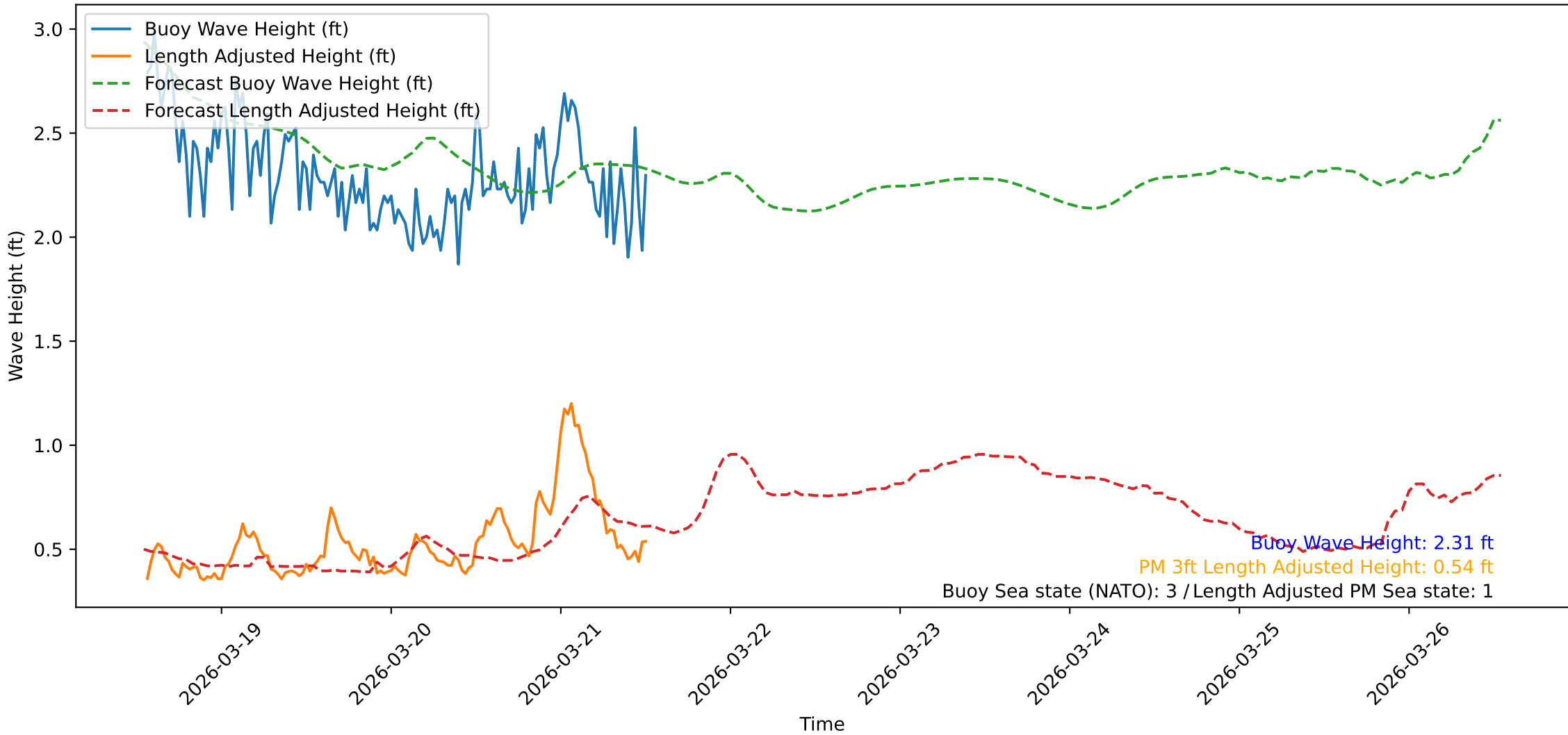
Wave Heights over Time for Red Beach at 2026-03-21 13:00:48
