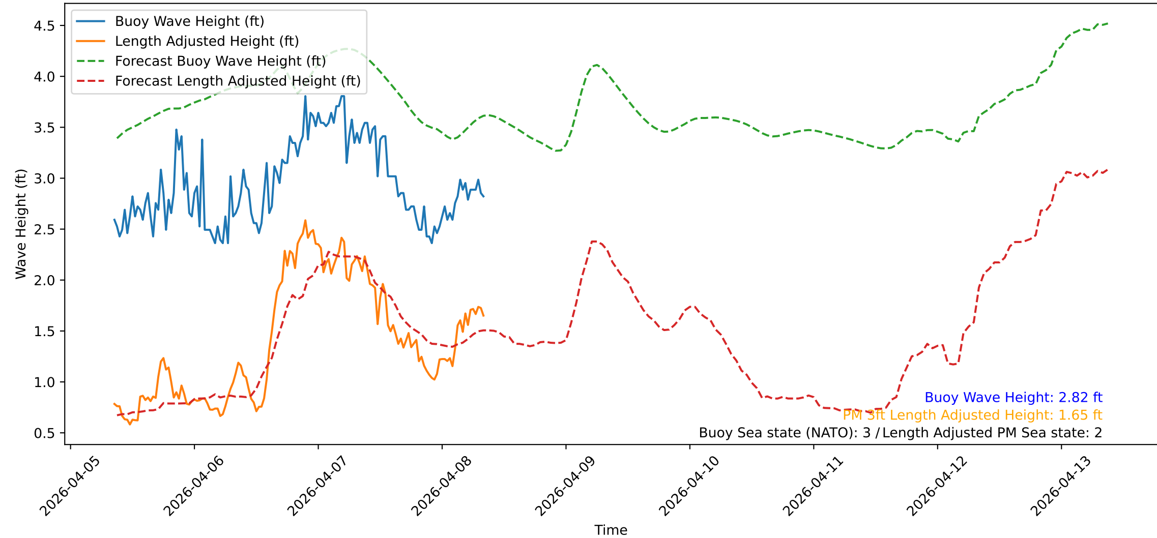
Wave Heights over Time for Green Beach at 2026-04-08 08:41:10
