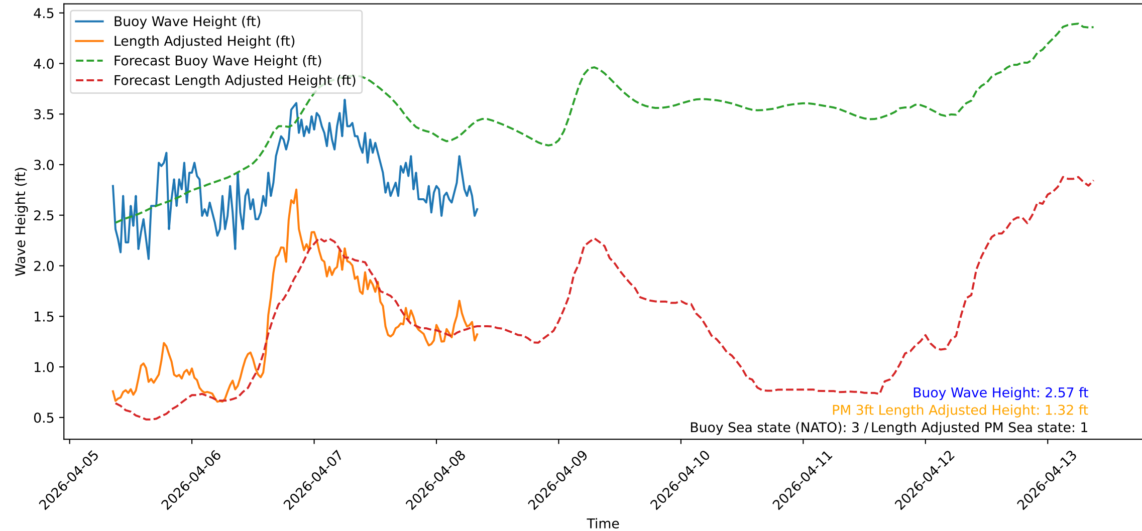
Wave Heights over Time for Oceanside Harbor at 2026-04-08 08:40:31
