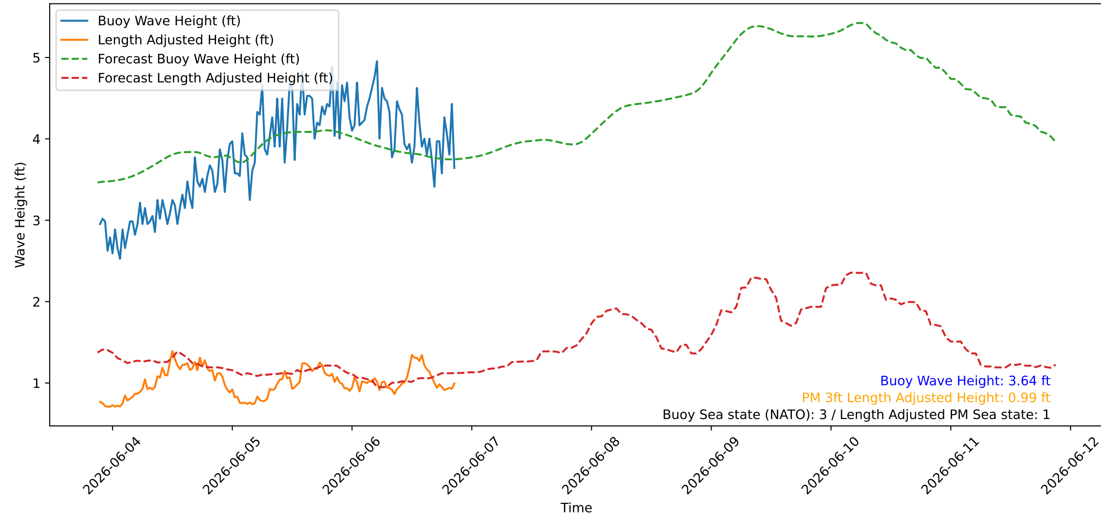
Wave Heights over Time for Red Beach at 2026-06-06 21:10:47
