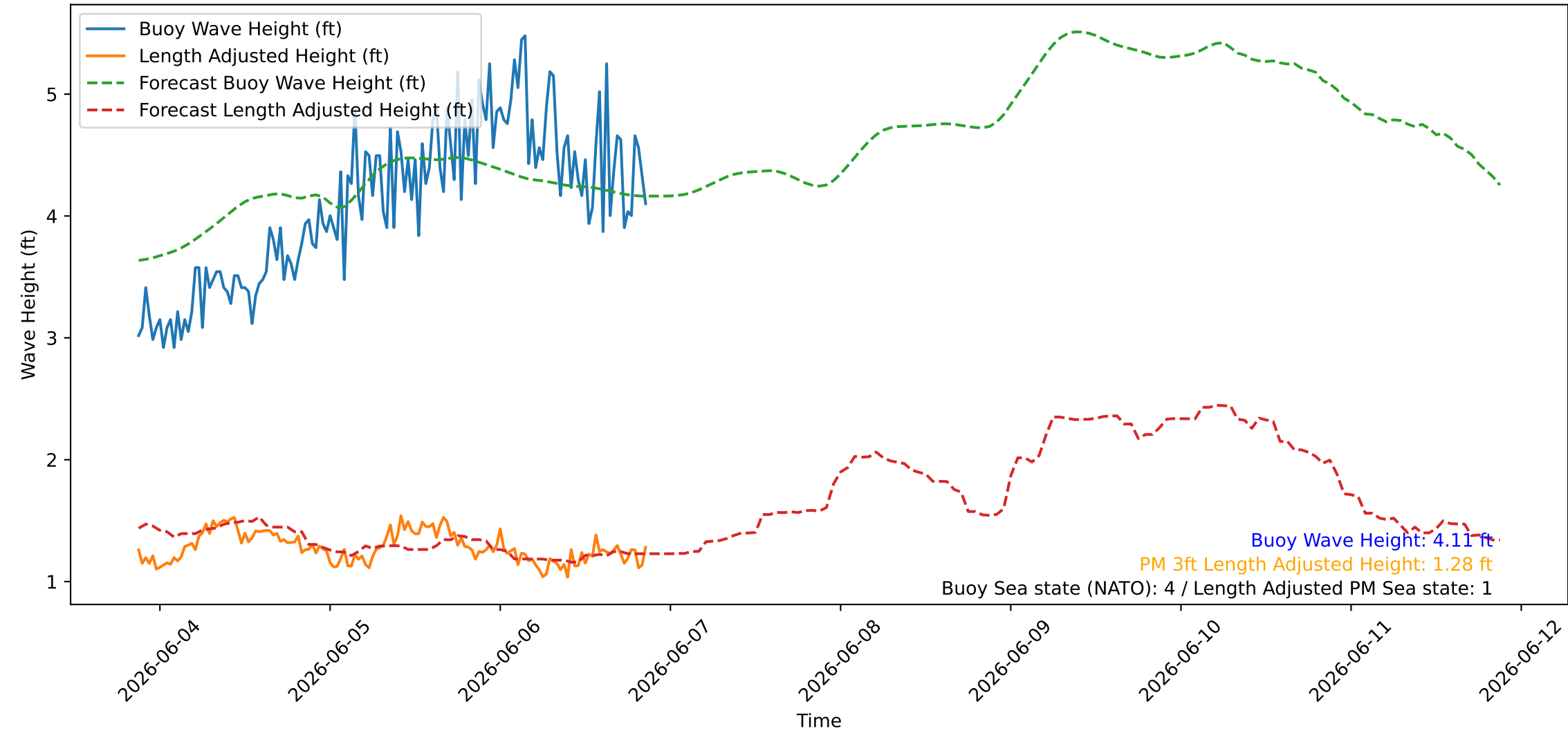
Wave Heights over Time for Oceanside Harbor at 2026-06-06 21:10:27
