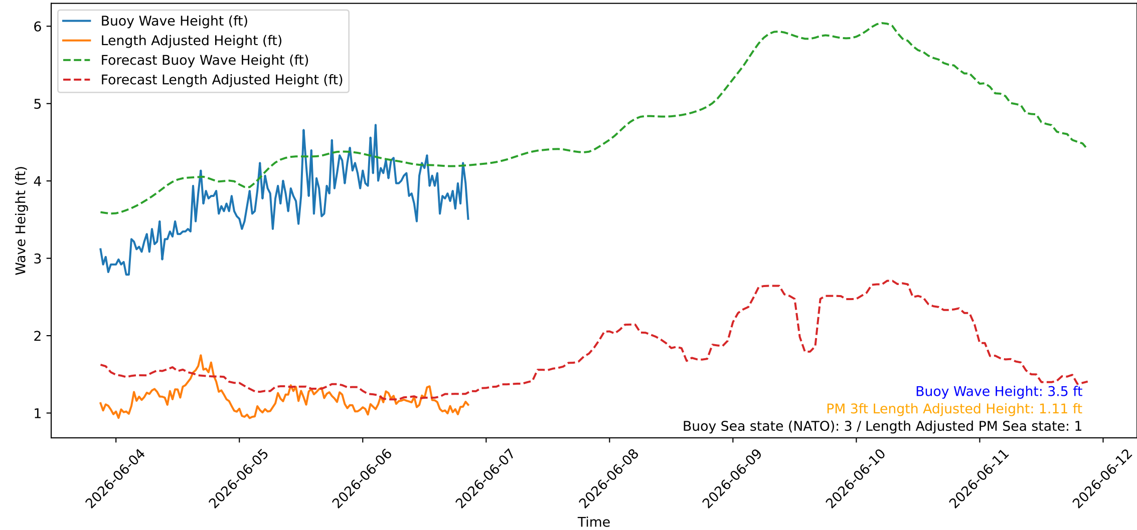
Wave Heights over Time for Green Beach at 2026-06-06 21:11:09
