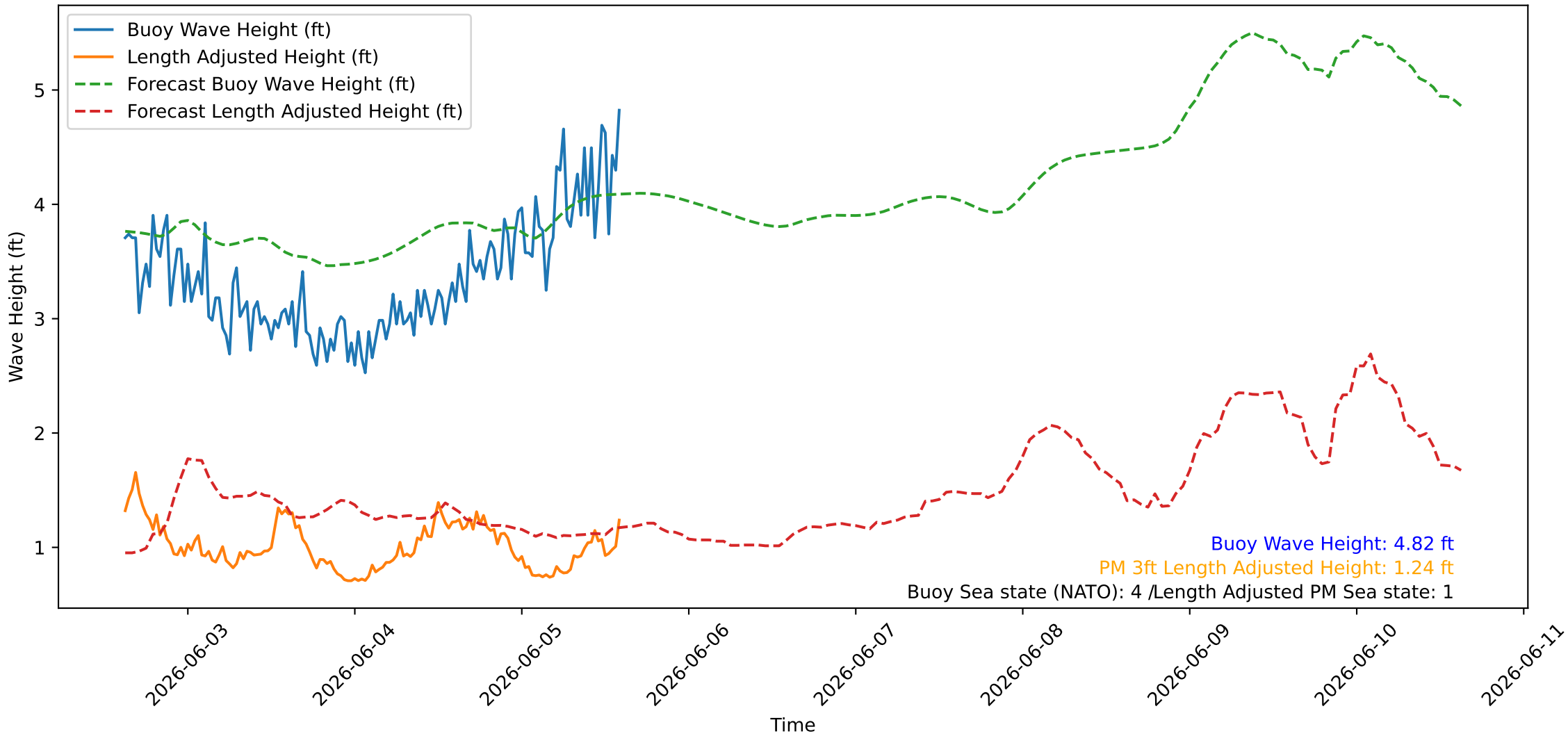
Wave Heights over Time for Red Beach at 2026-06-05 14:50:46
