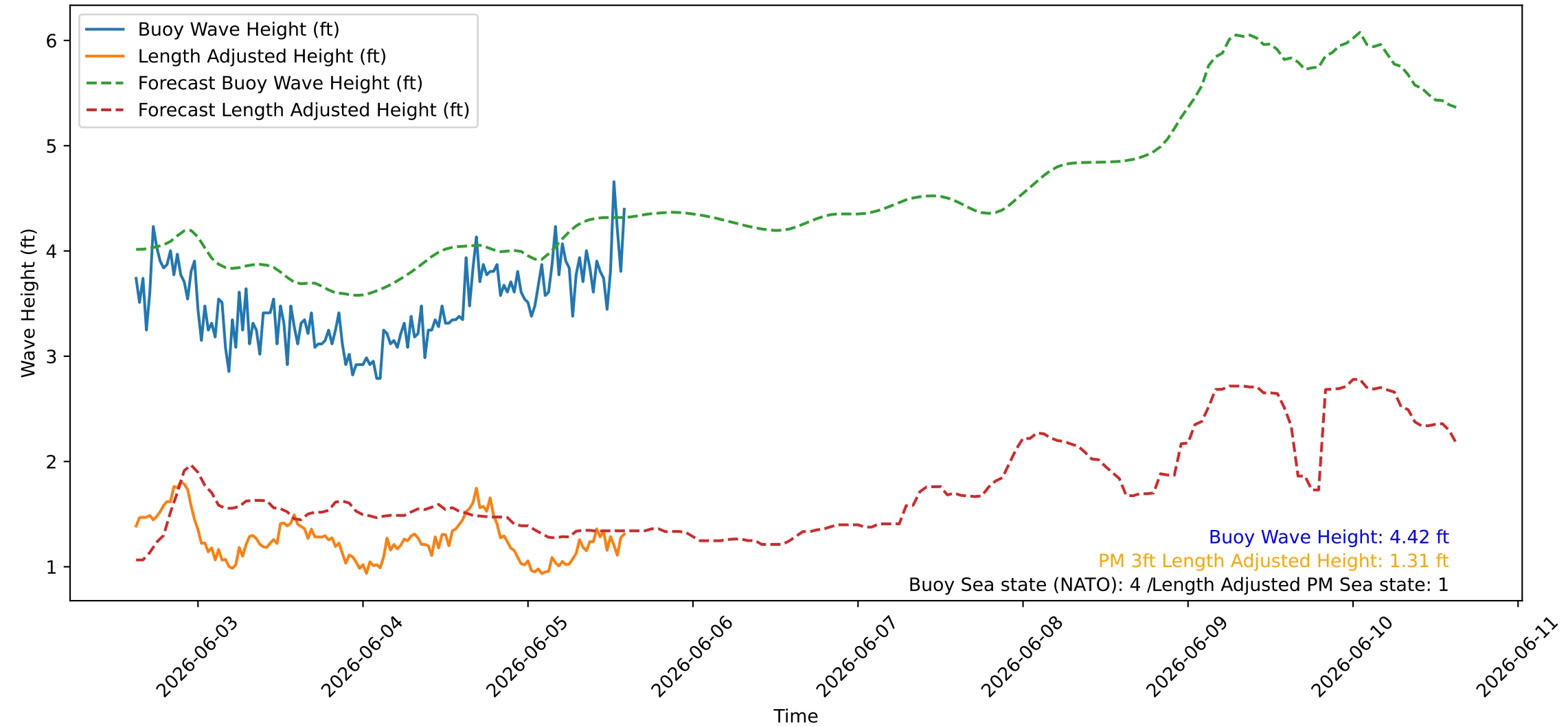
Wave Heights over Time for Green Beach at 2026-06-05 14:51:10
