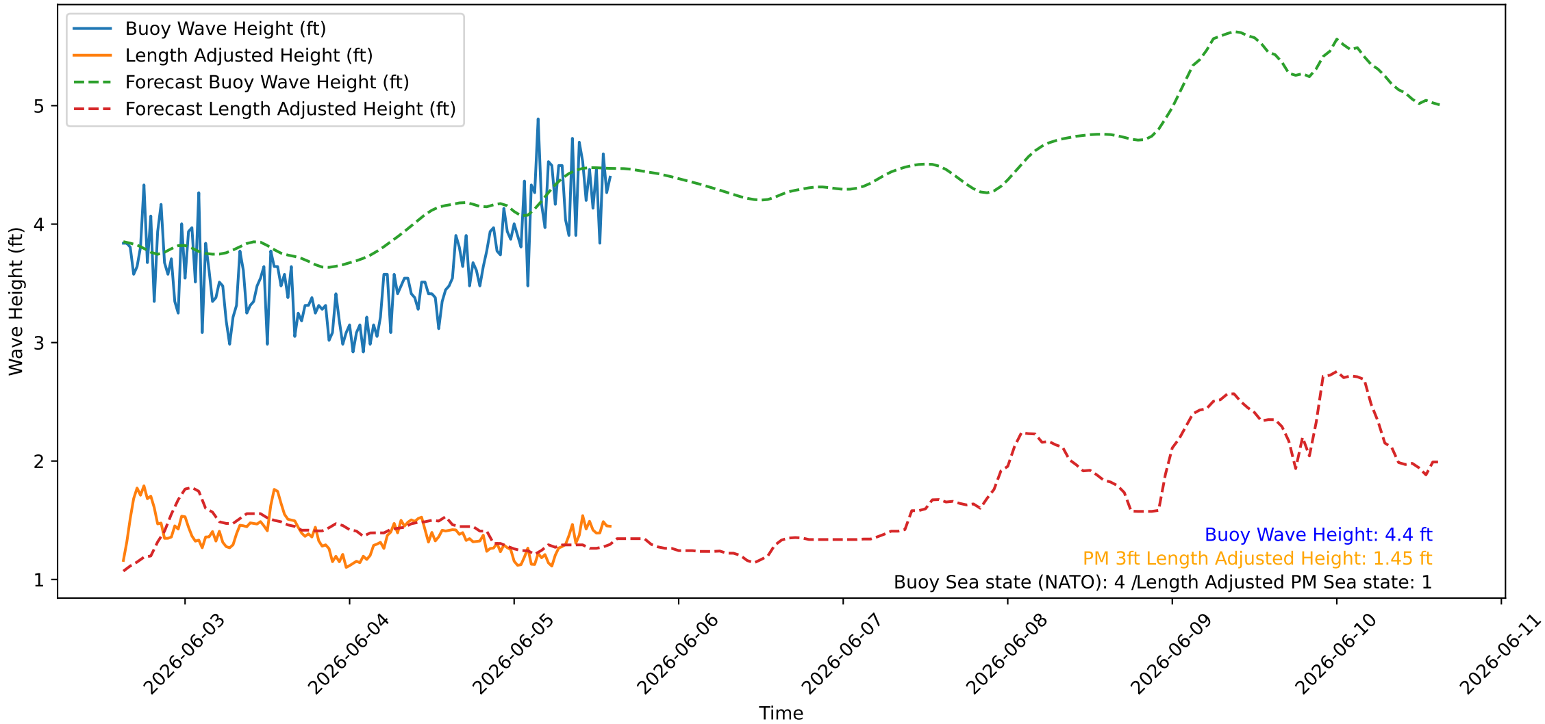
Wave Heights over Time for Oceanside Harbor at 2026-06-05 14:50:25
