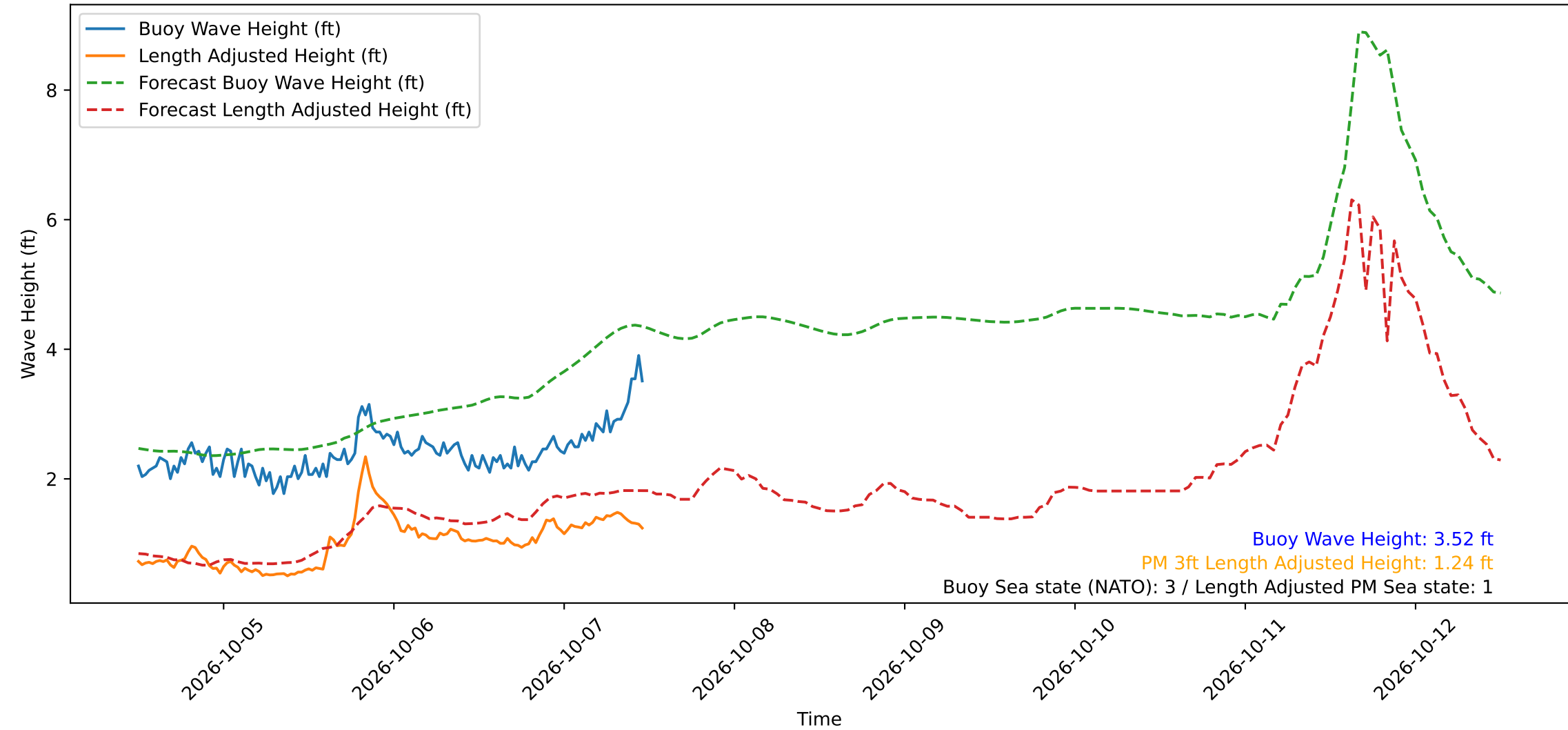
Wave Heights over Time for Green Beach at 2026-10-07 11:41:13
