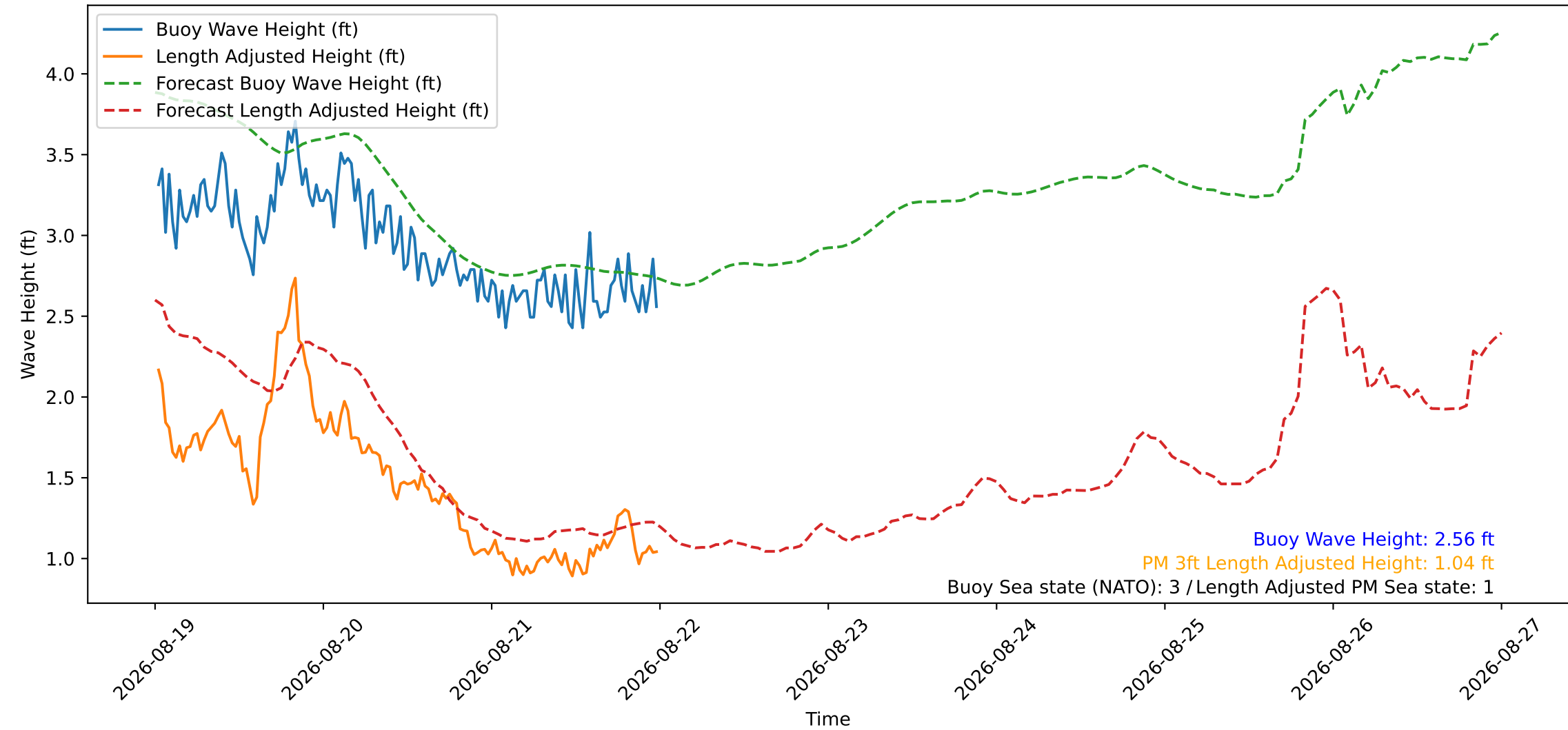
Wave Heights over Time for Green Beach at 2026-08-22 00:11:12
