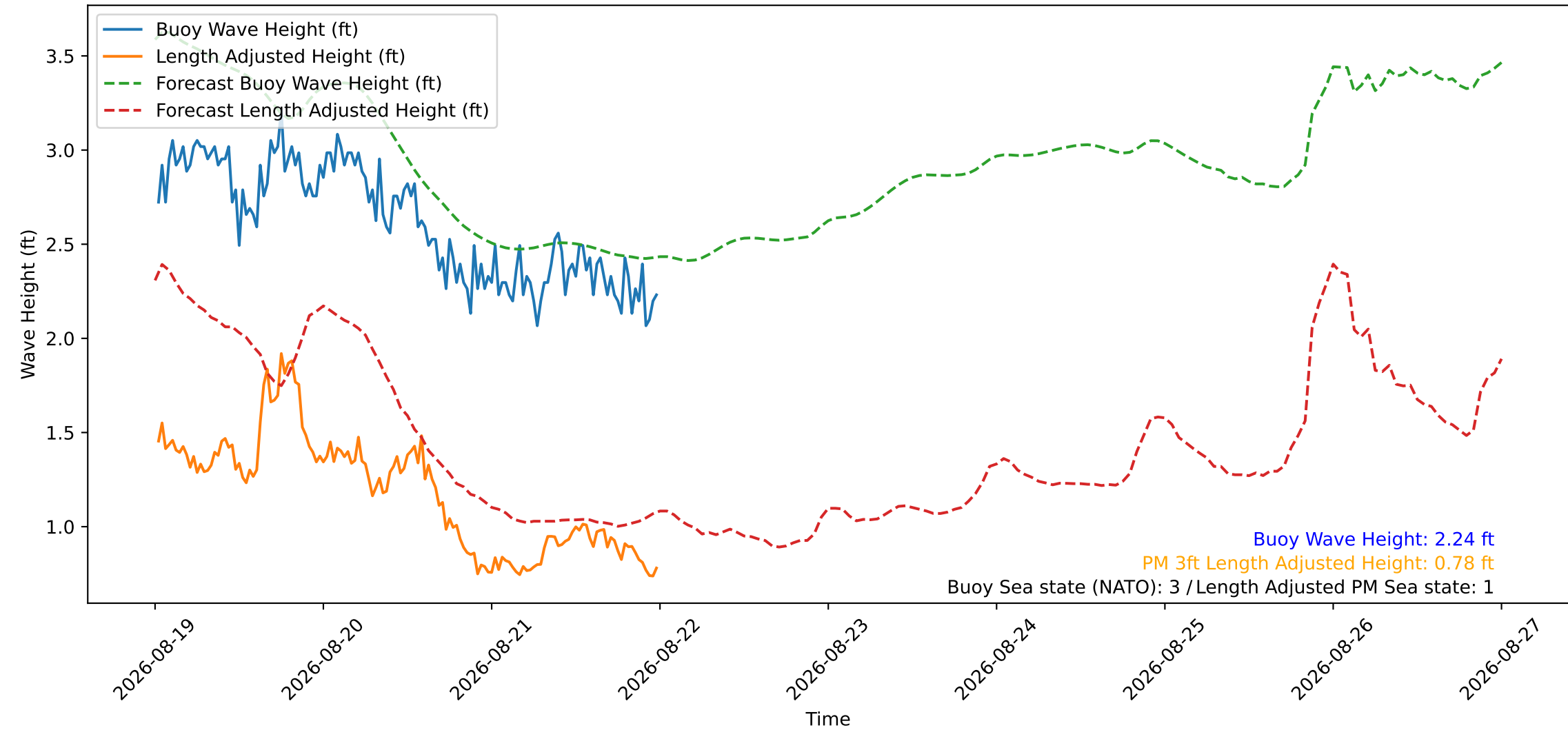
Wave Heights over Time for Red Beach at 2026-08-22 00:10:50
