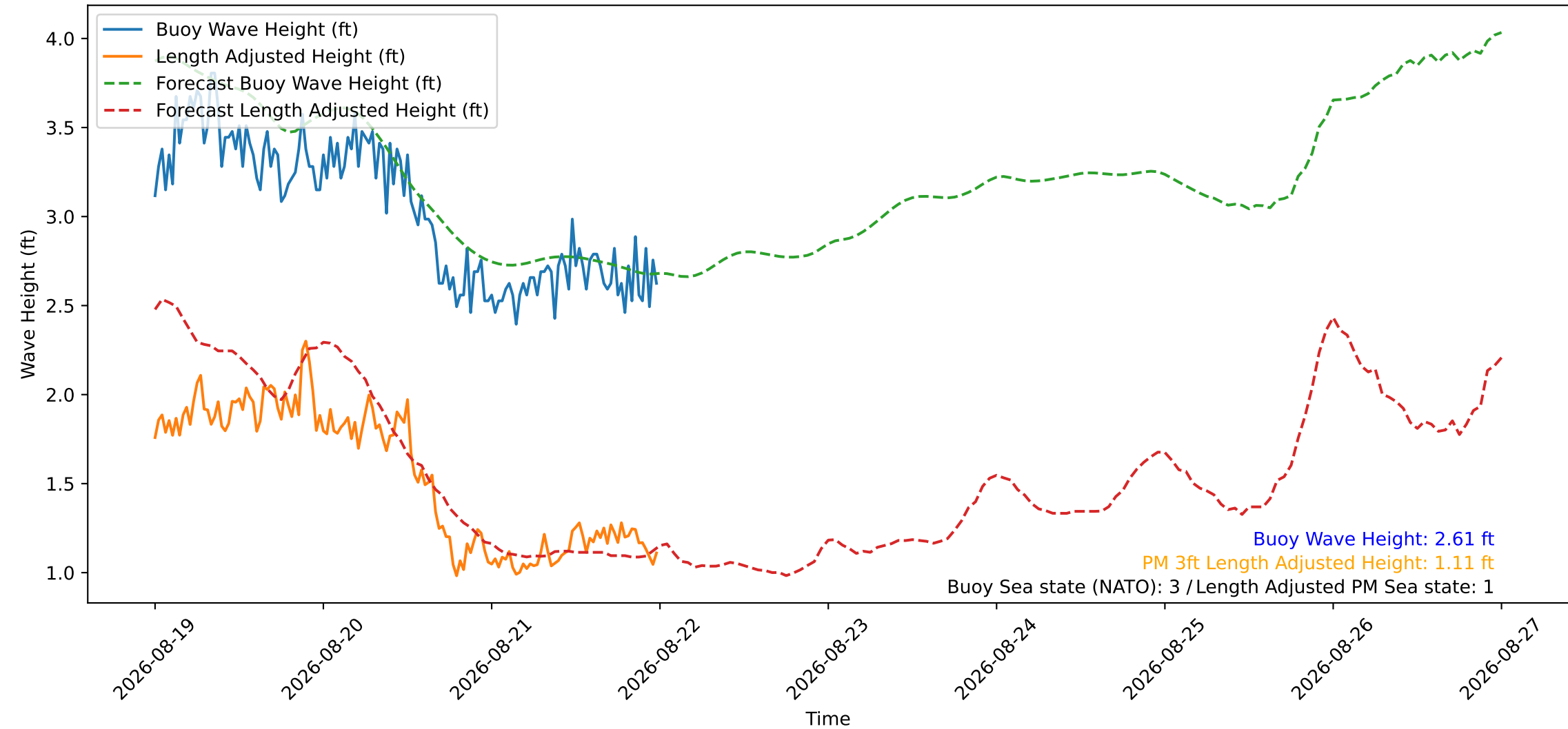
Wave Heights over Time for Oceanside Harbor at 2026-08-22 00:10:30
