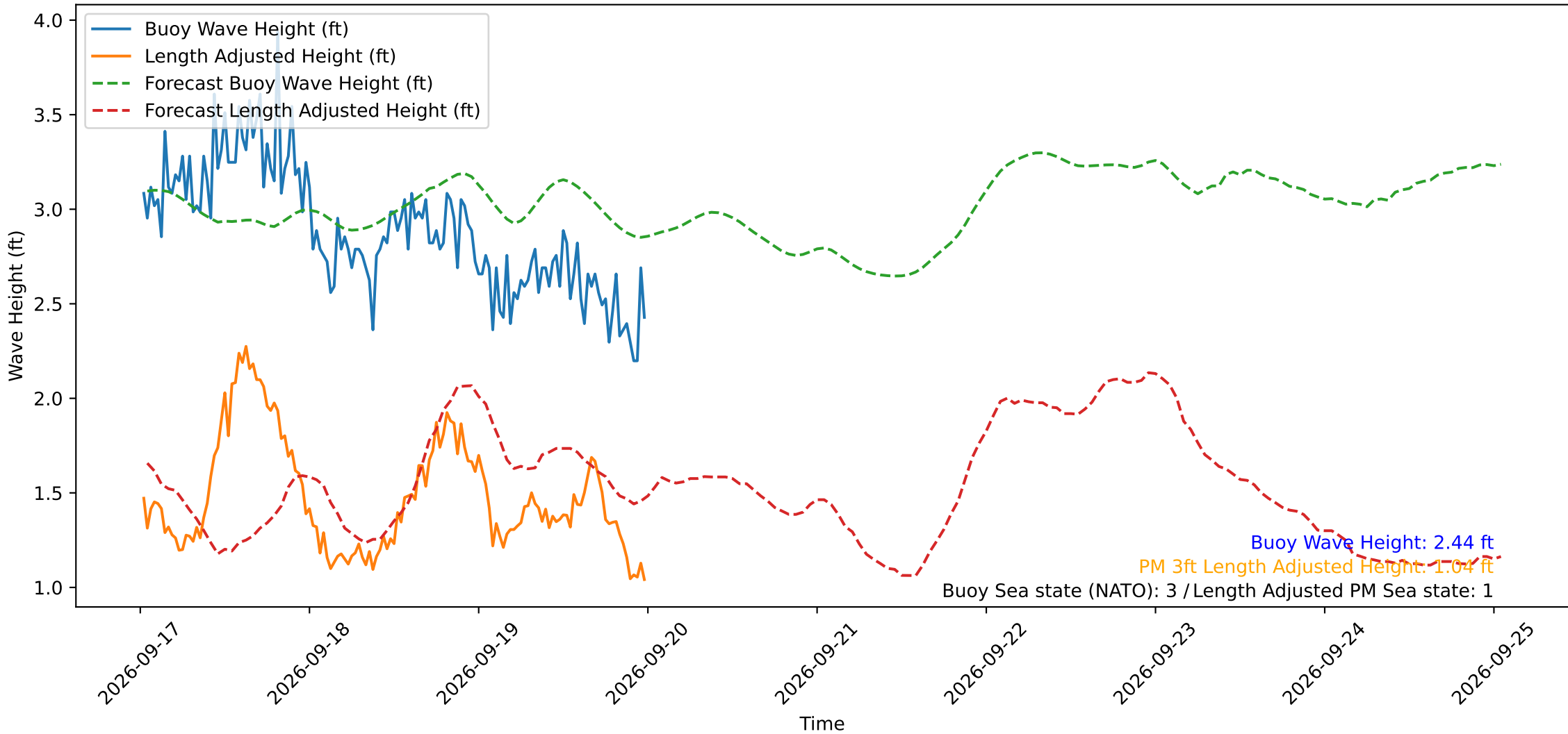
Wave Heights over Time for Oceanside Harbor at 2026-09-20 00:30:29
