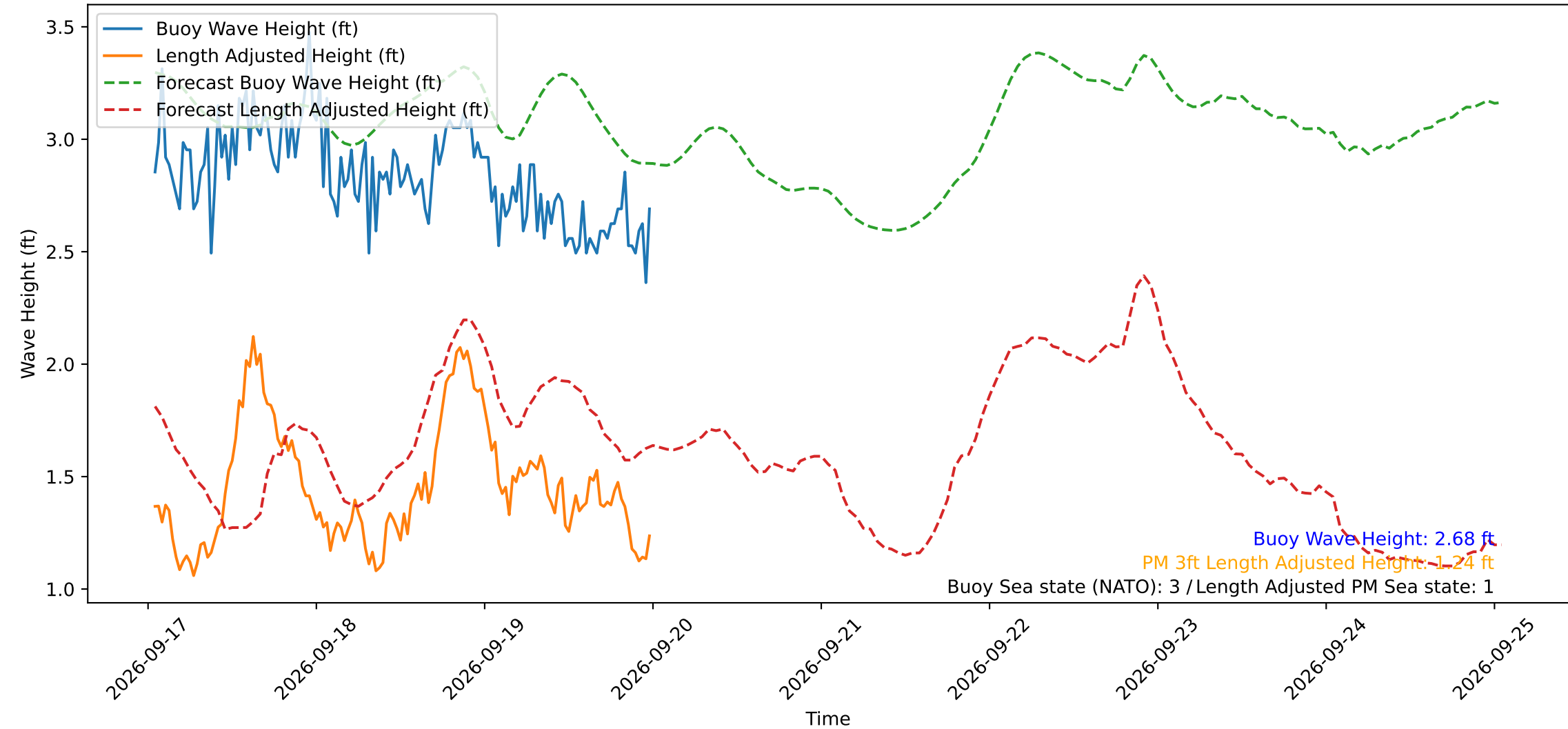
Wave Heights over Time for Green Beach at 2026-09-20 00:31:11
