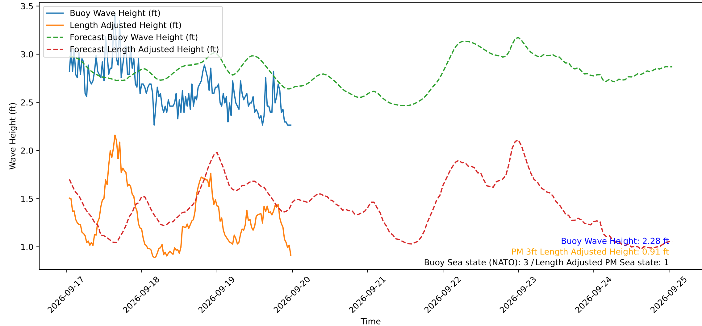
Wave Heights over Time for Red Beach at 2026-09-20 00:30:49
