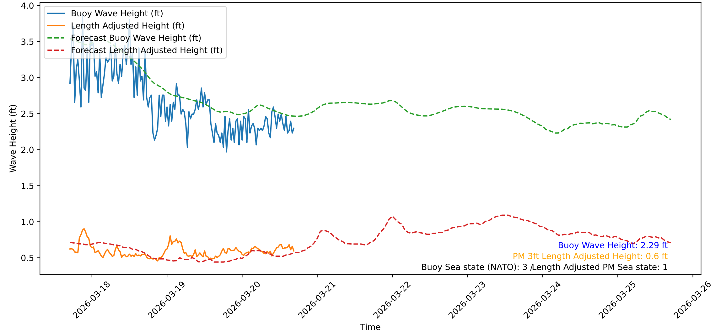
Wave Heights over Time for Oceanside Harbor at 2026-03-20 17:10:32
