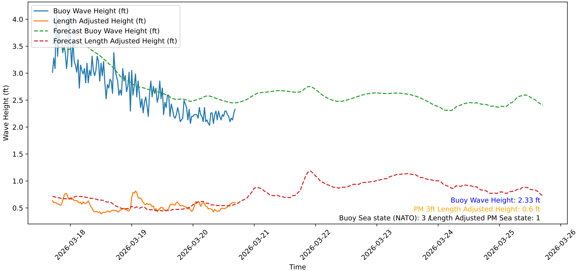
Wave Heights over Time for Green Beach at 2026-03-20 17:11:11
