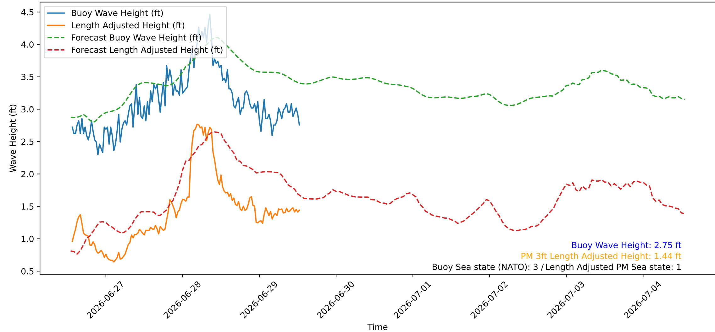
Wave Heights over Time for Red Beach at 2026-06-29 13:10:44
