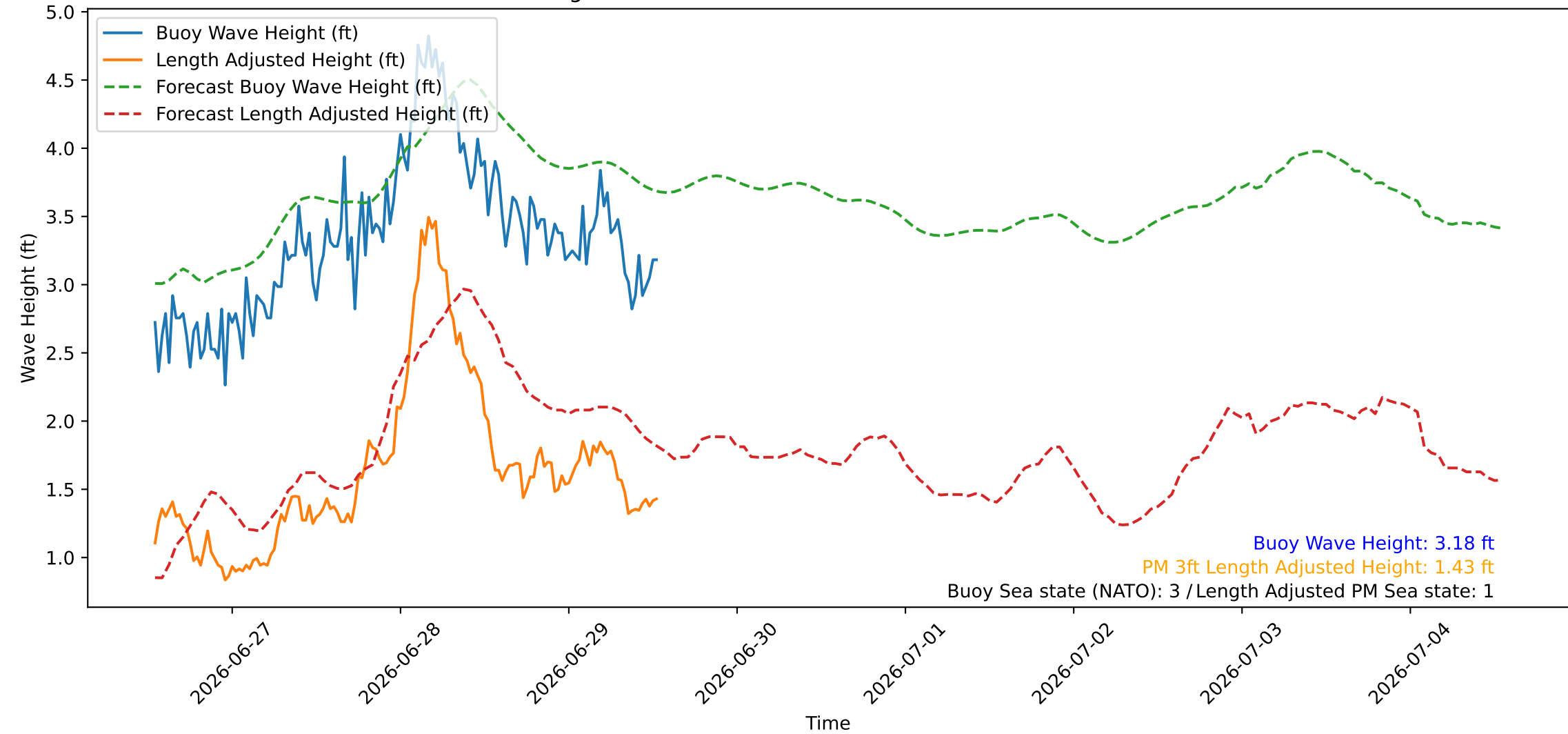
Wave Heights over Time for Green Beach at 2026-06-29 13:11:07
