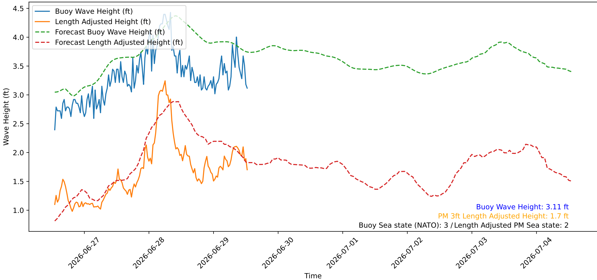
Wave Heights over Time for Oceanside Harbor at 2026-06-29 13:10:25
