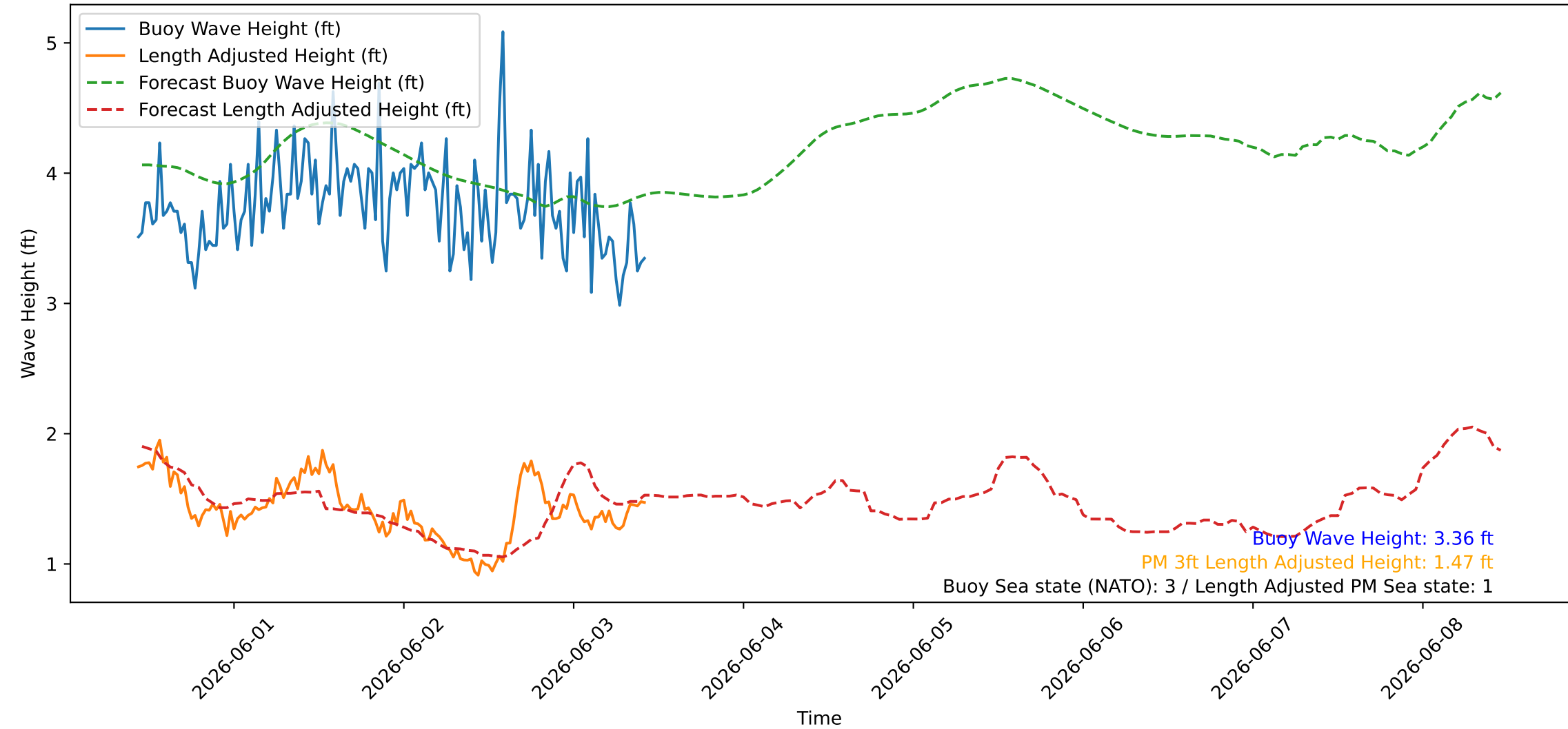
Wave Heights over Time for Oceanside Harbor at 2026-06-03 10:40:26
