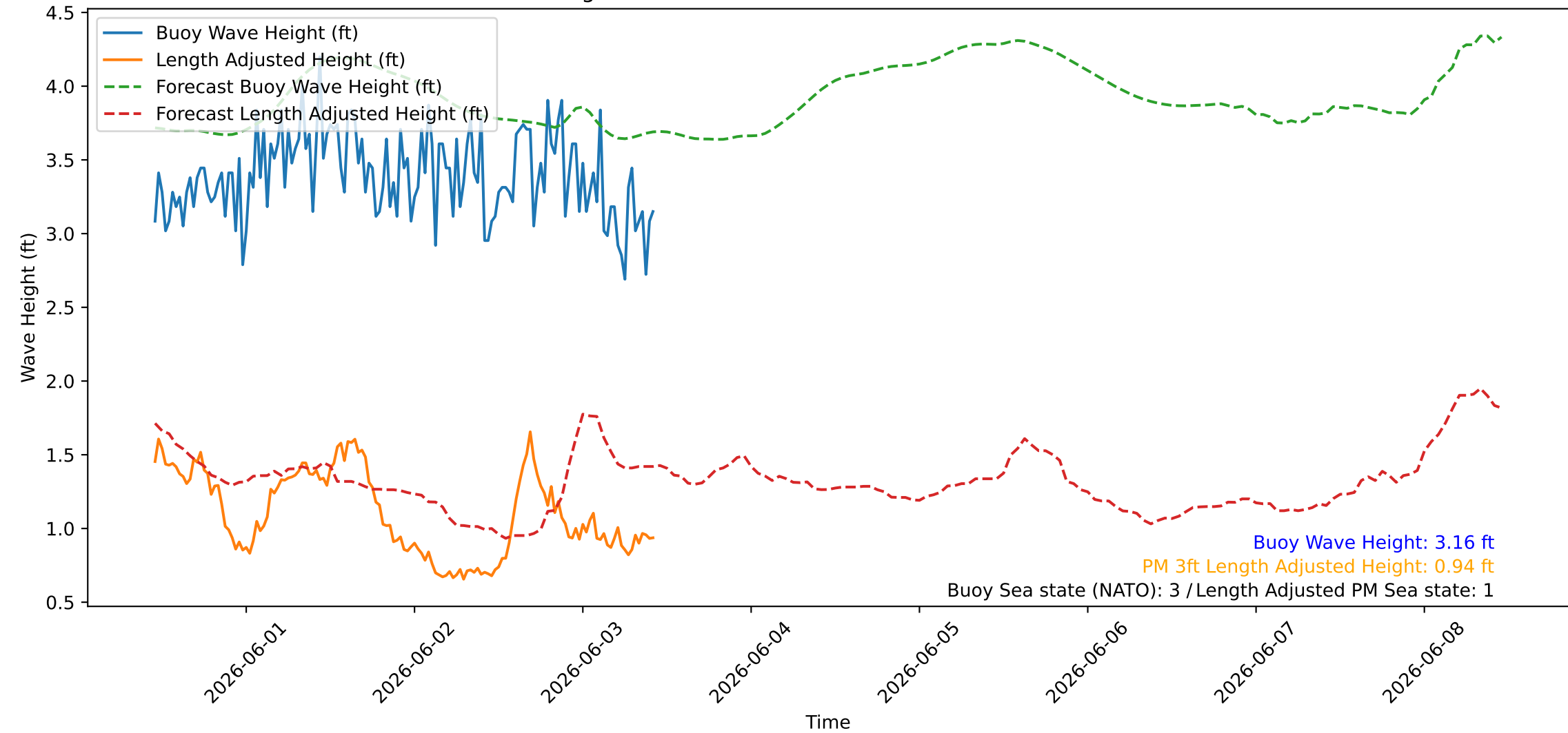
Wave Heights over Time for Red Beach at 2026-06-03 10:40:45
