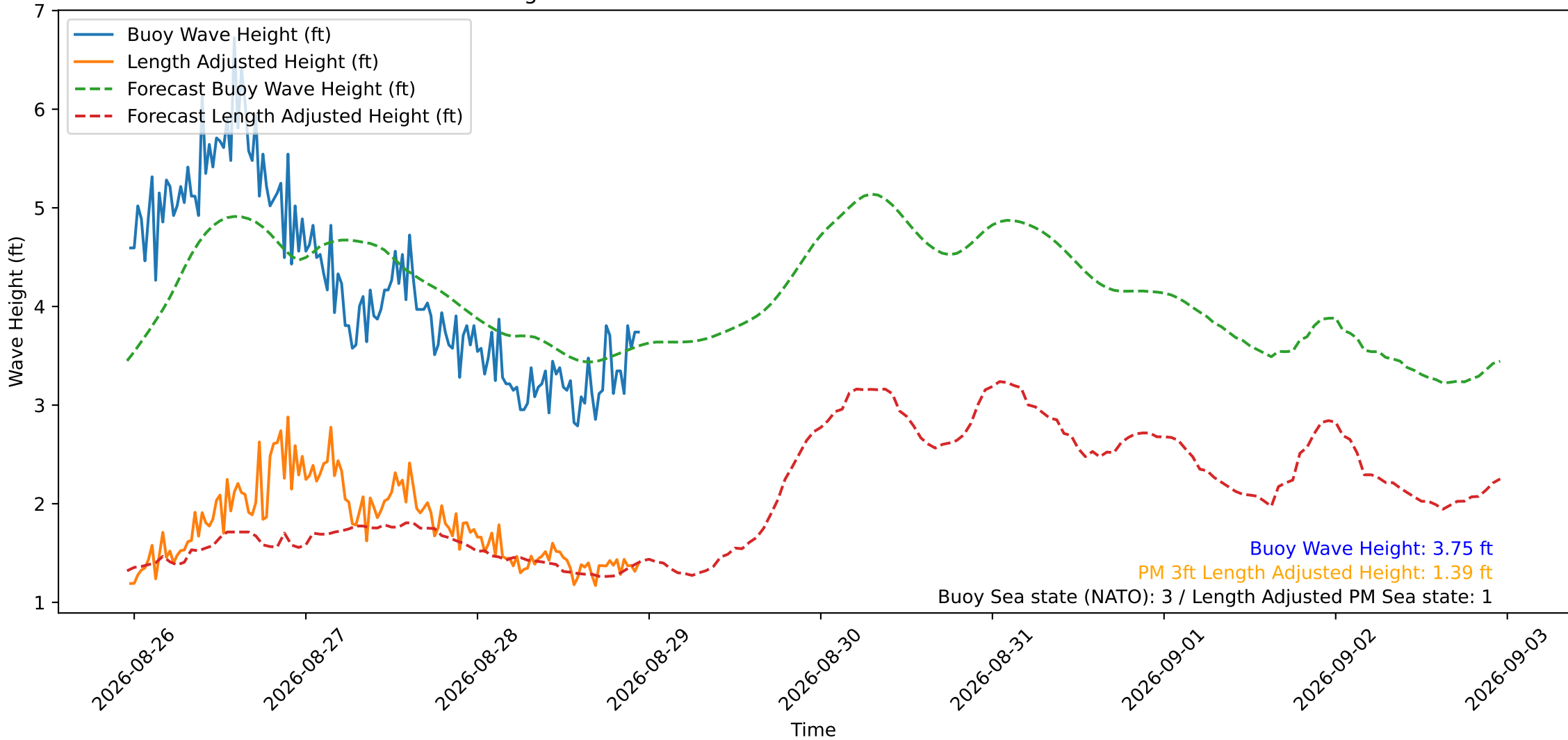
Wave Heights over Time for Oceanside Harbor at 2026-08-28 23:20:29
