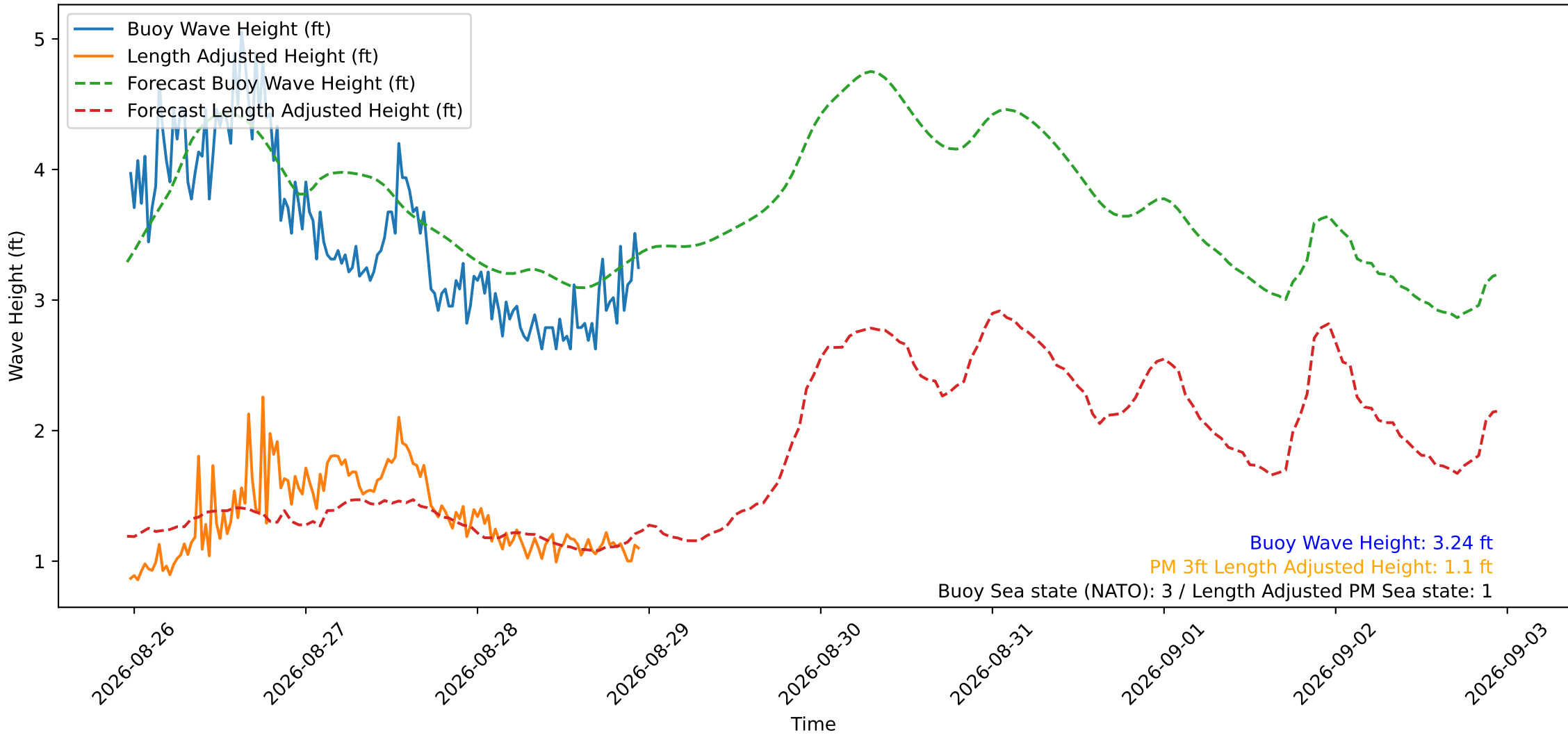
Wave Heights over Time for Red Beach at 2026-08-28 23:20:50
