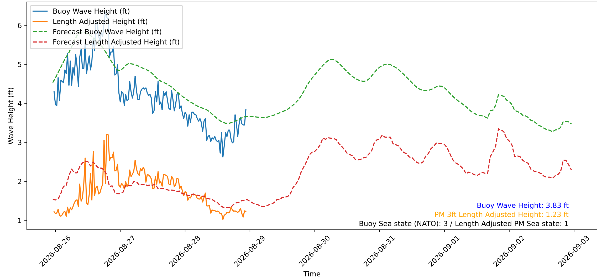
Wave Heights over Time for Green Beach at 2026-08-28 23:21:14
