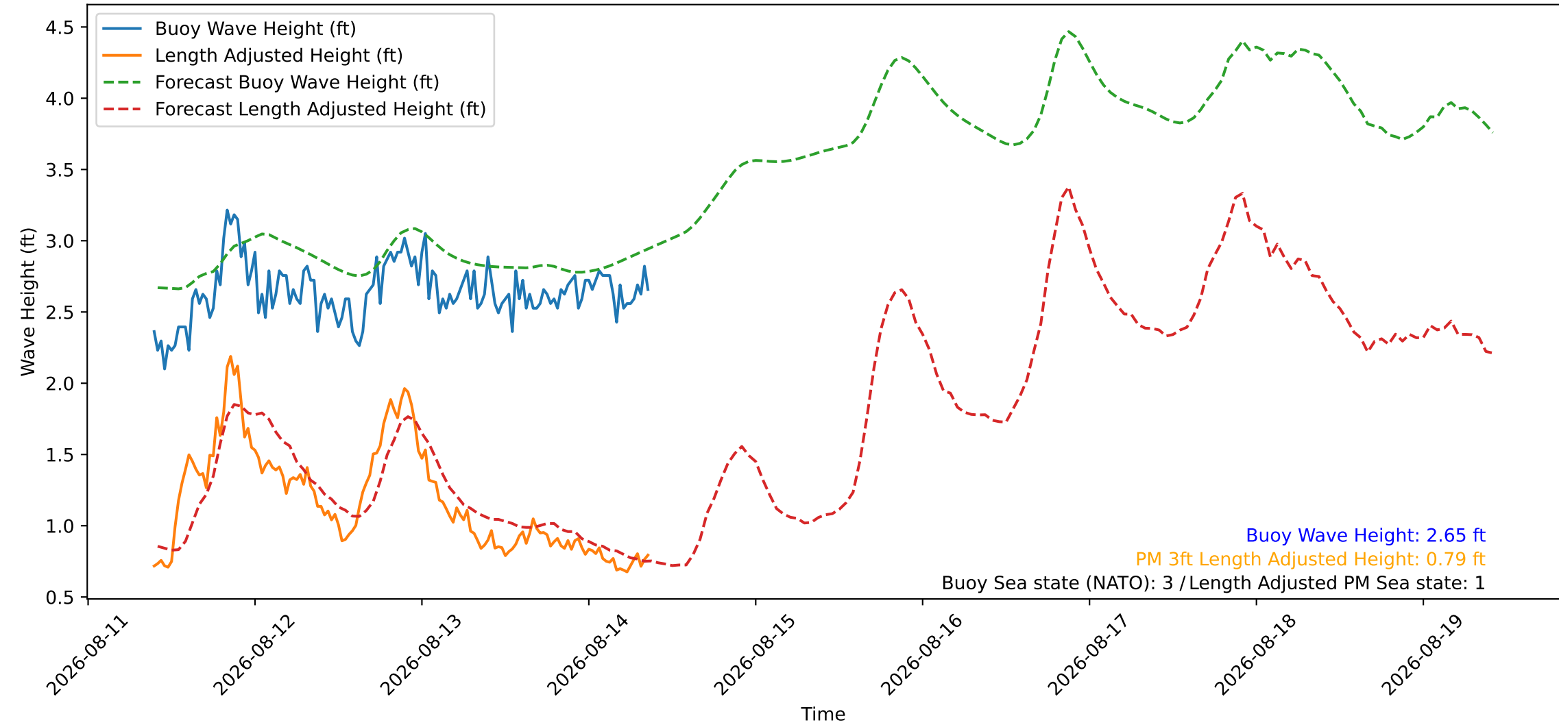
Wave Heights over Time for Green Beach at 2026-08-14 09:31:08
