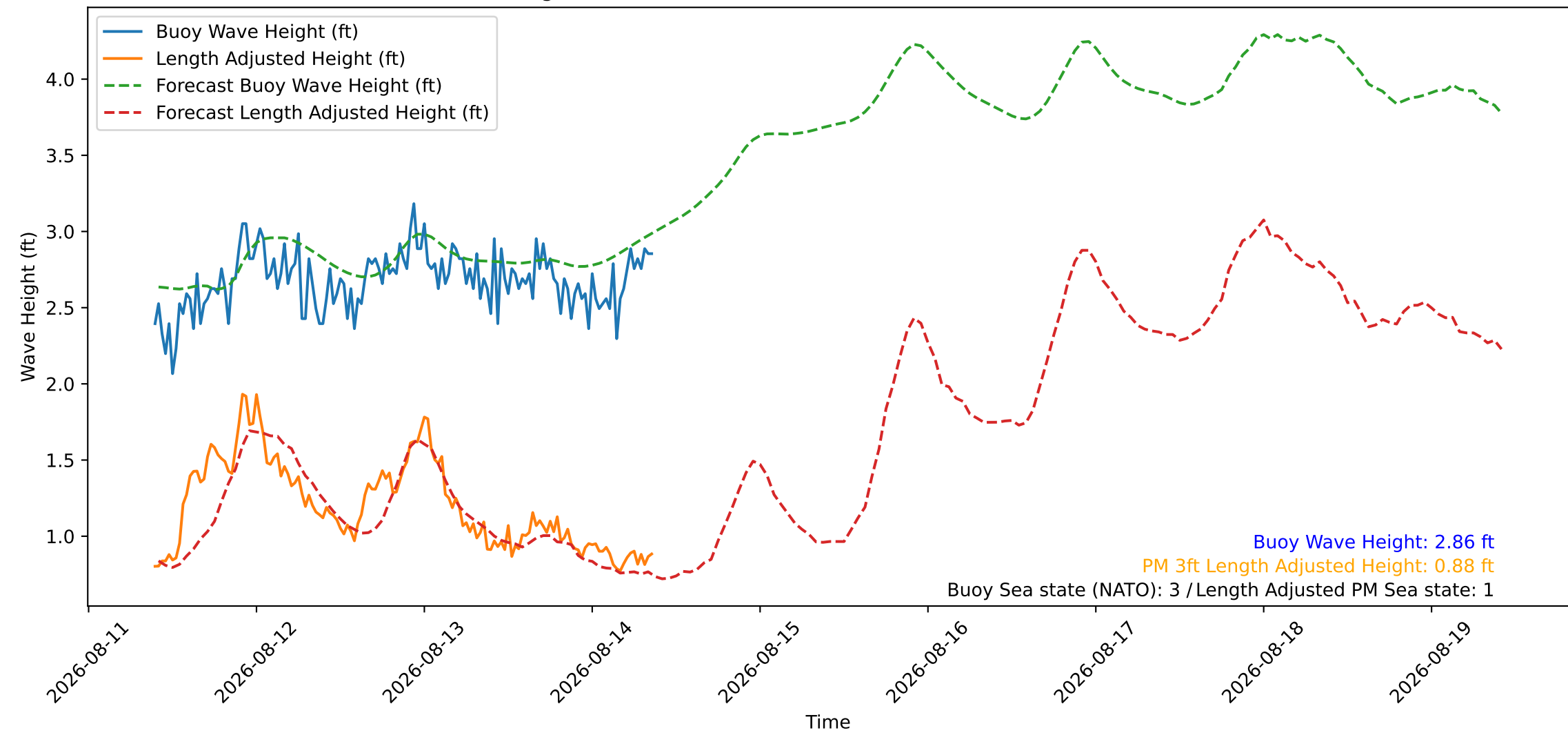
Wave Heights over Time for Oceanside Harbor at 2026-08-14 09:30:26
