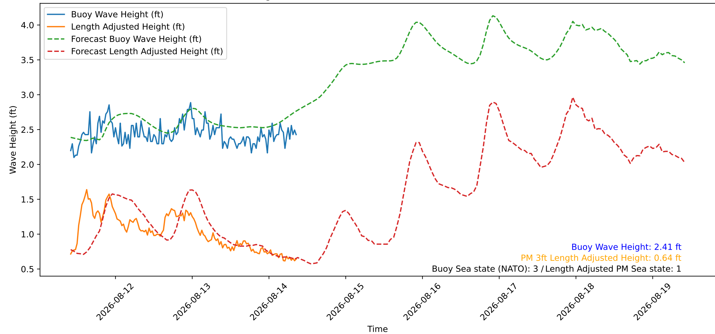
Wave Heights over Time for Red Beach at 2026-08-14 09:30:46
