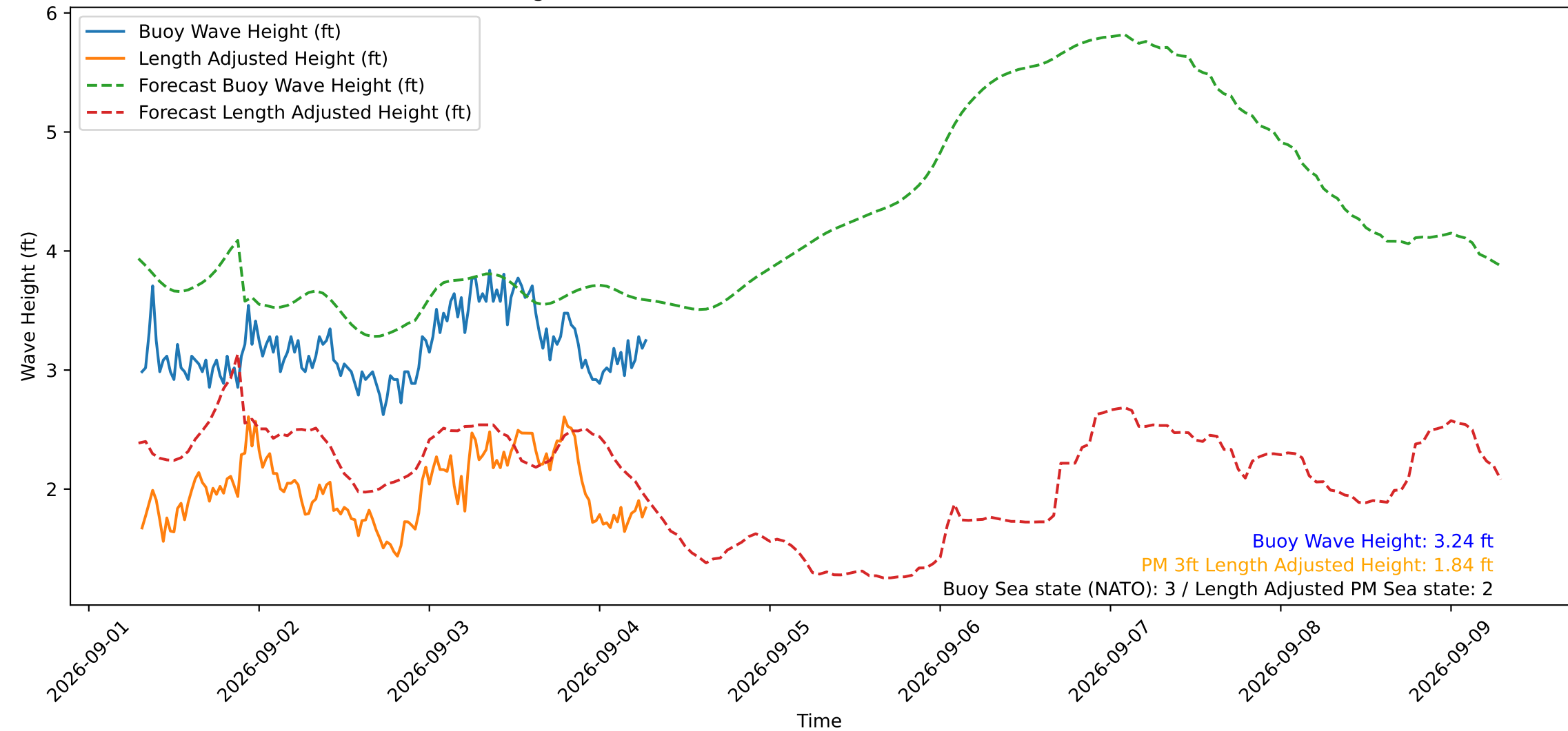
Wave Heights over Time for Oceanside Harbor at 2026-09-04 07:20:30
