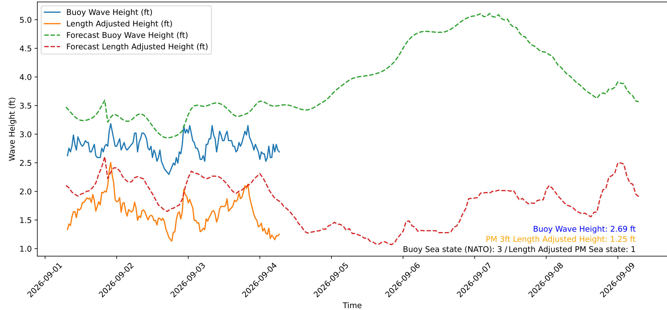
Wave Heights over Time for Red Beach at 2026-09-04 07:20:50
