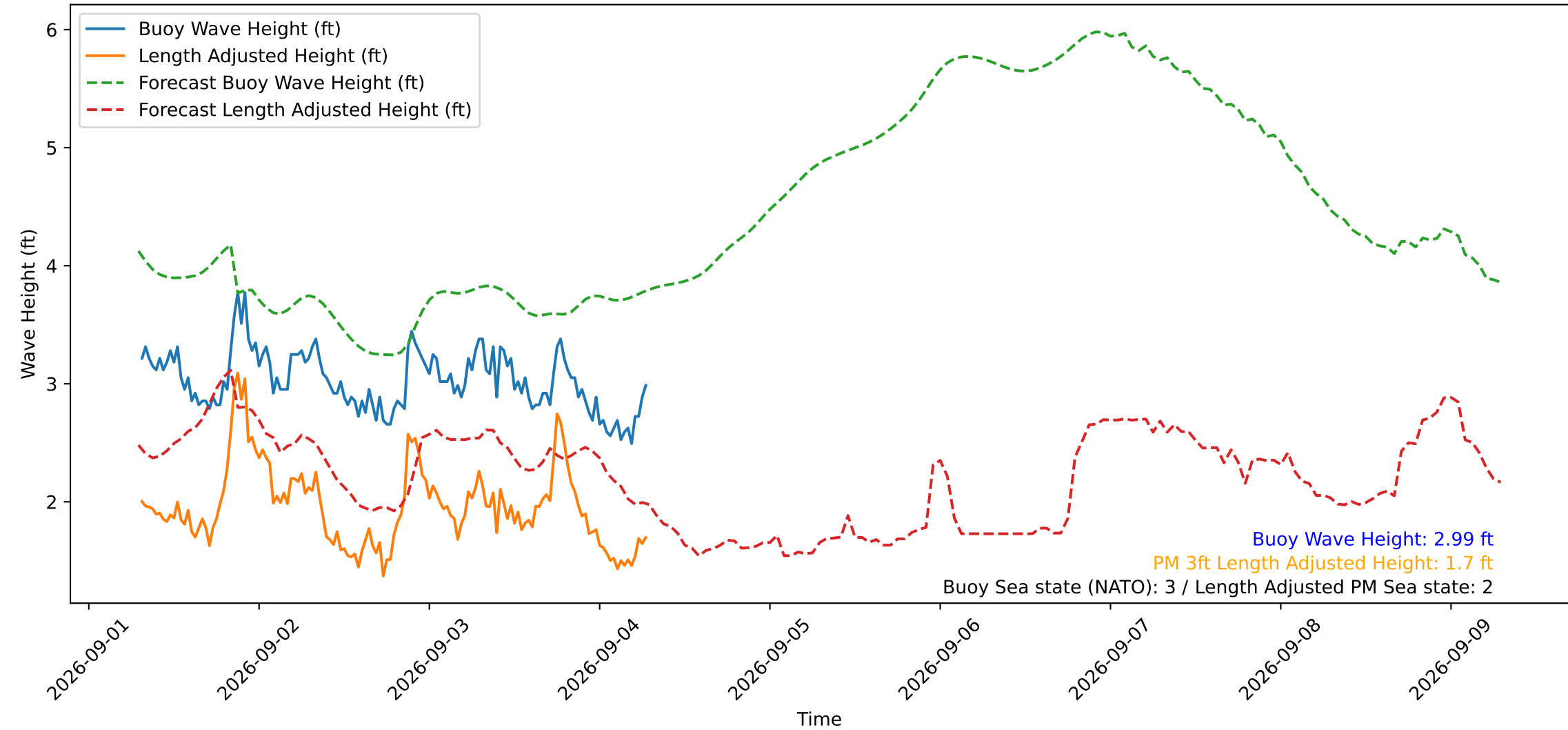
Wave Heights over Time for Green Beach at 2026-09-04 07:21:15
