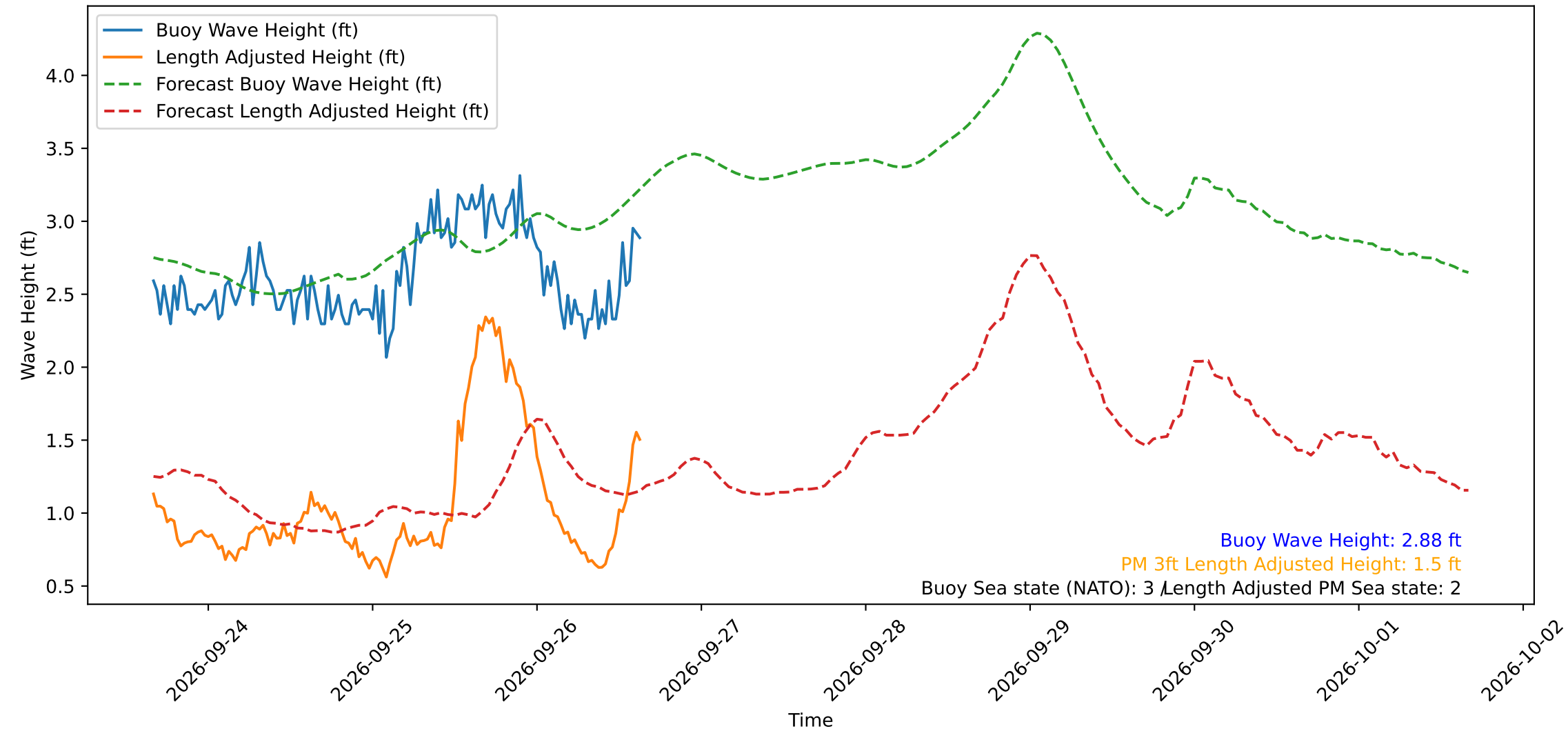
Wave Heights over Time for Red Beach at 2026-09-26 15:50:50
