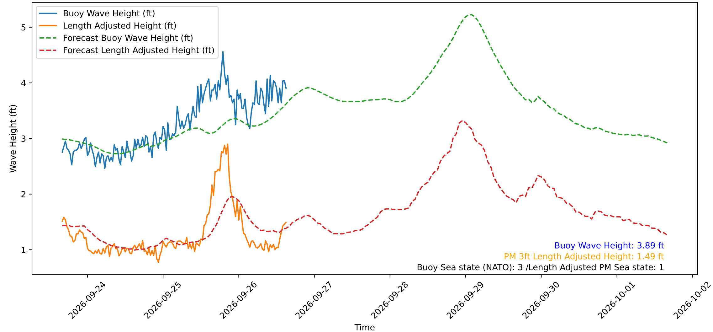
Wave Heights over Time for Green Beach at 2026-09-26 15:51:14
