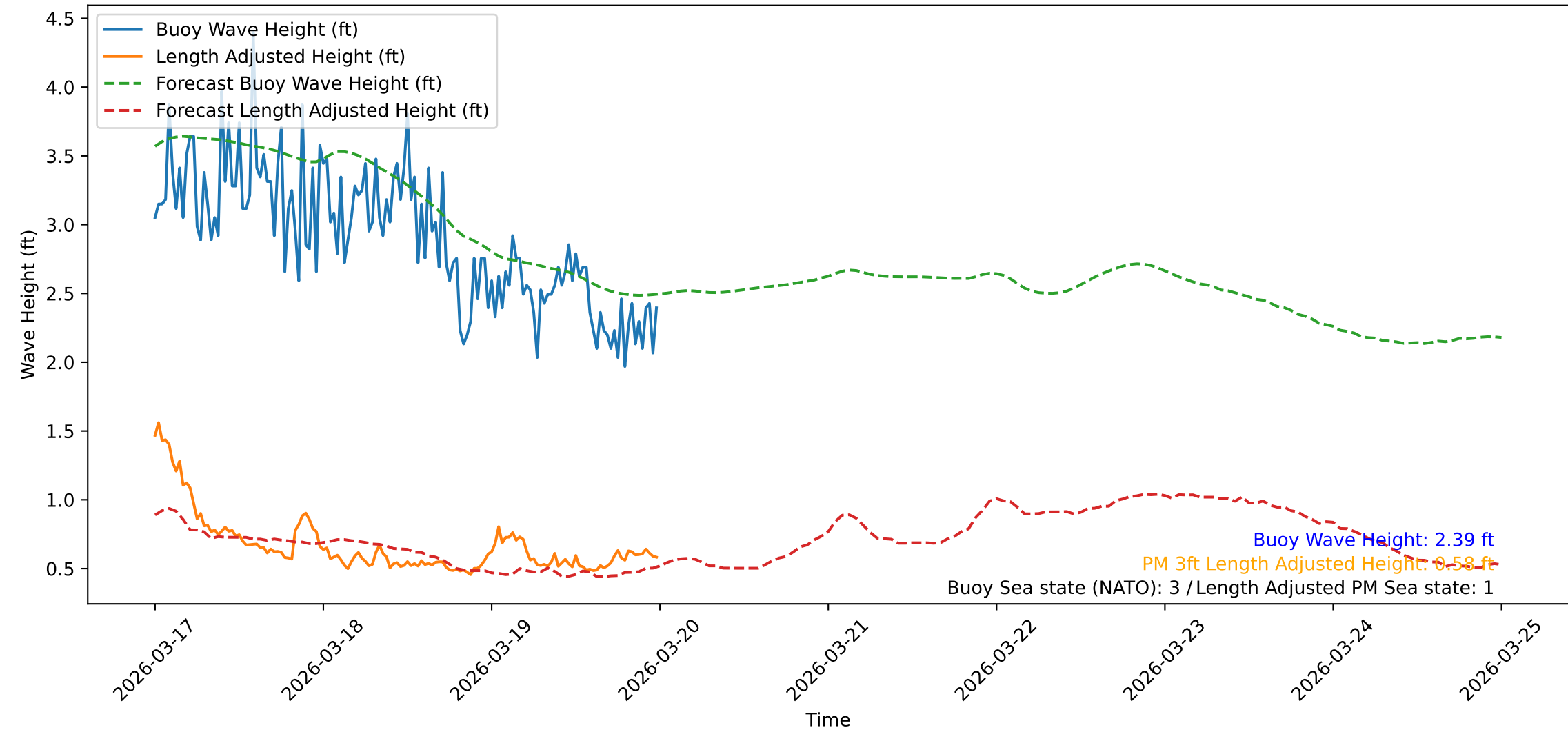
Wave Heights over Time for Oceanside Harbor at 2026-03-20 00:00:31
