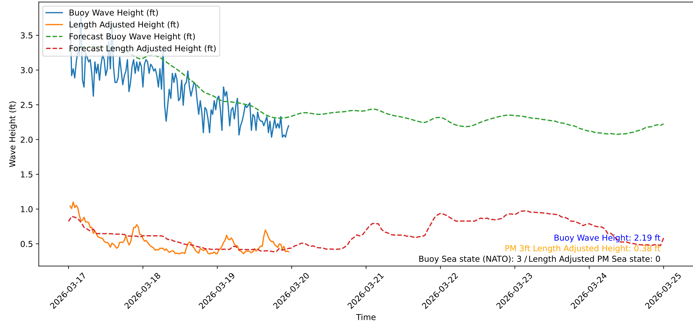
Wave Heights over Time for Red Beach at 2026-03-20 00:00:47
