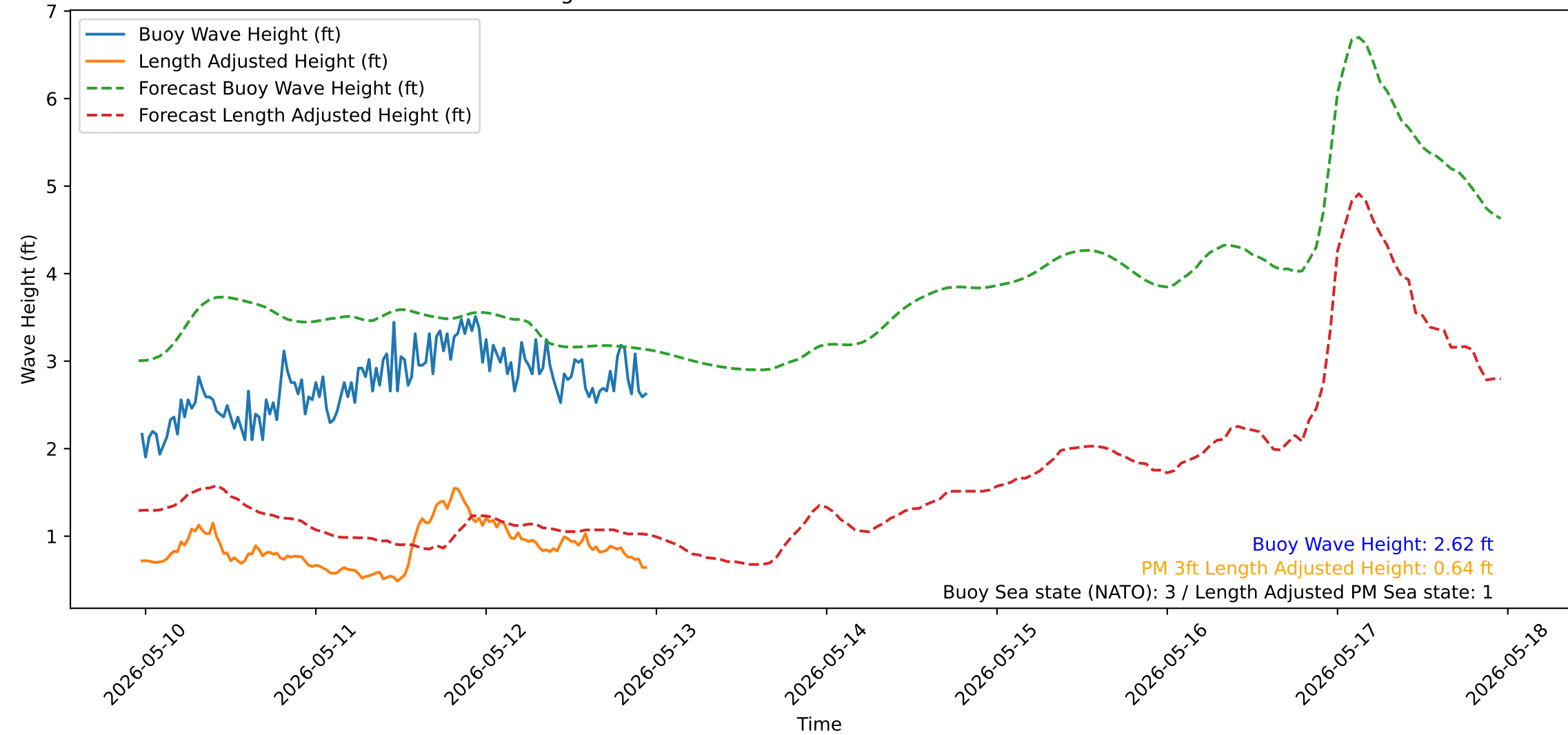
Wave Heights over Time for Green Beach at 2026-05-12 23:21:14
