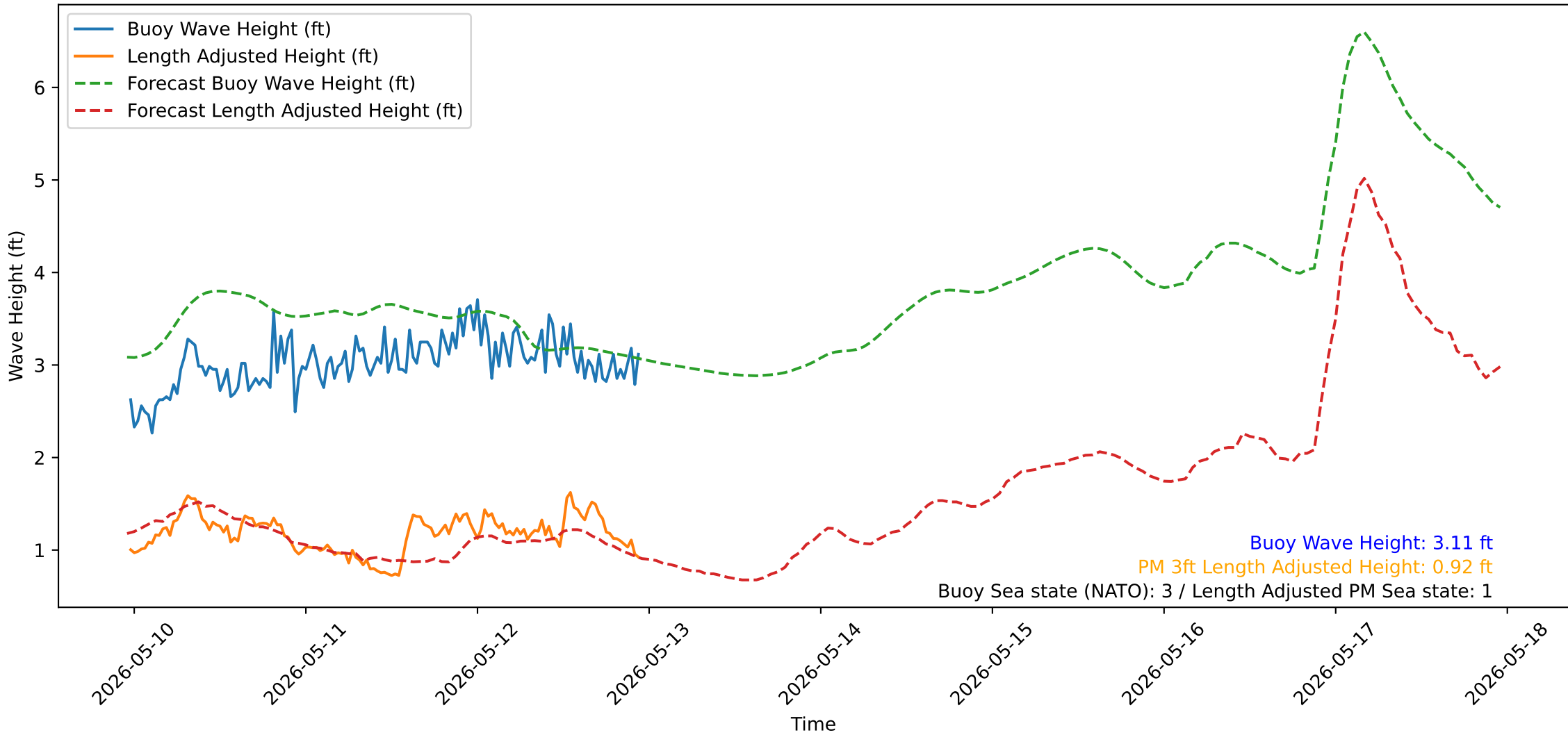
Wave Heights over Time for Oceanside Harbor at 2026-05-12 23:20:32
