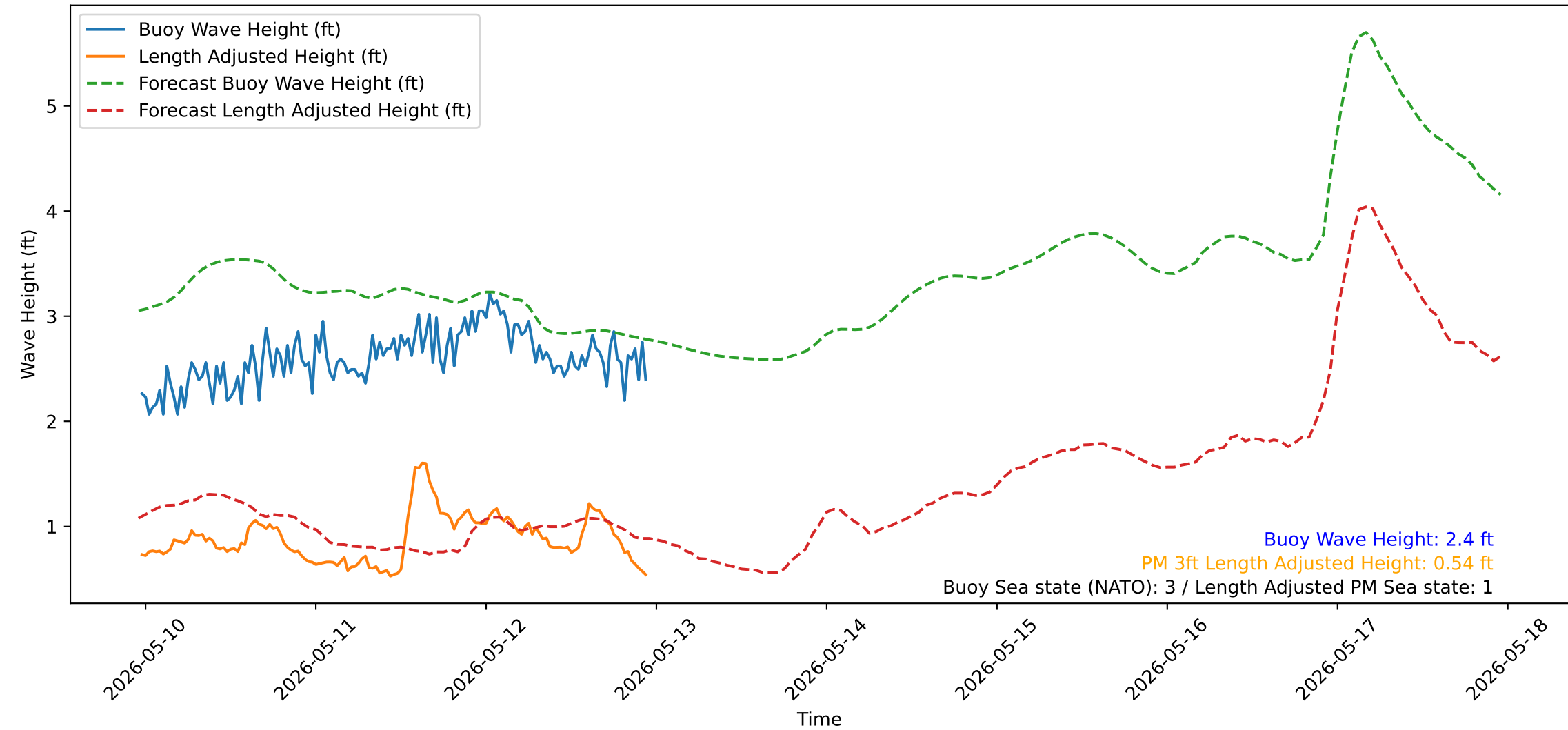
Wave Heights over Time for Red Beach at 2026-05-12 23:20:52
