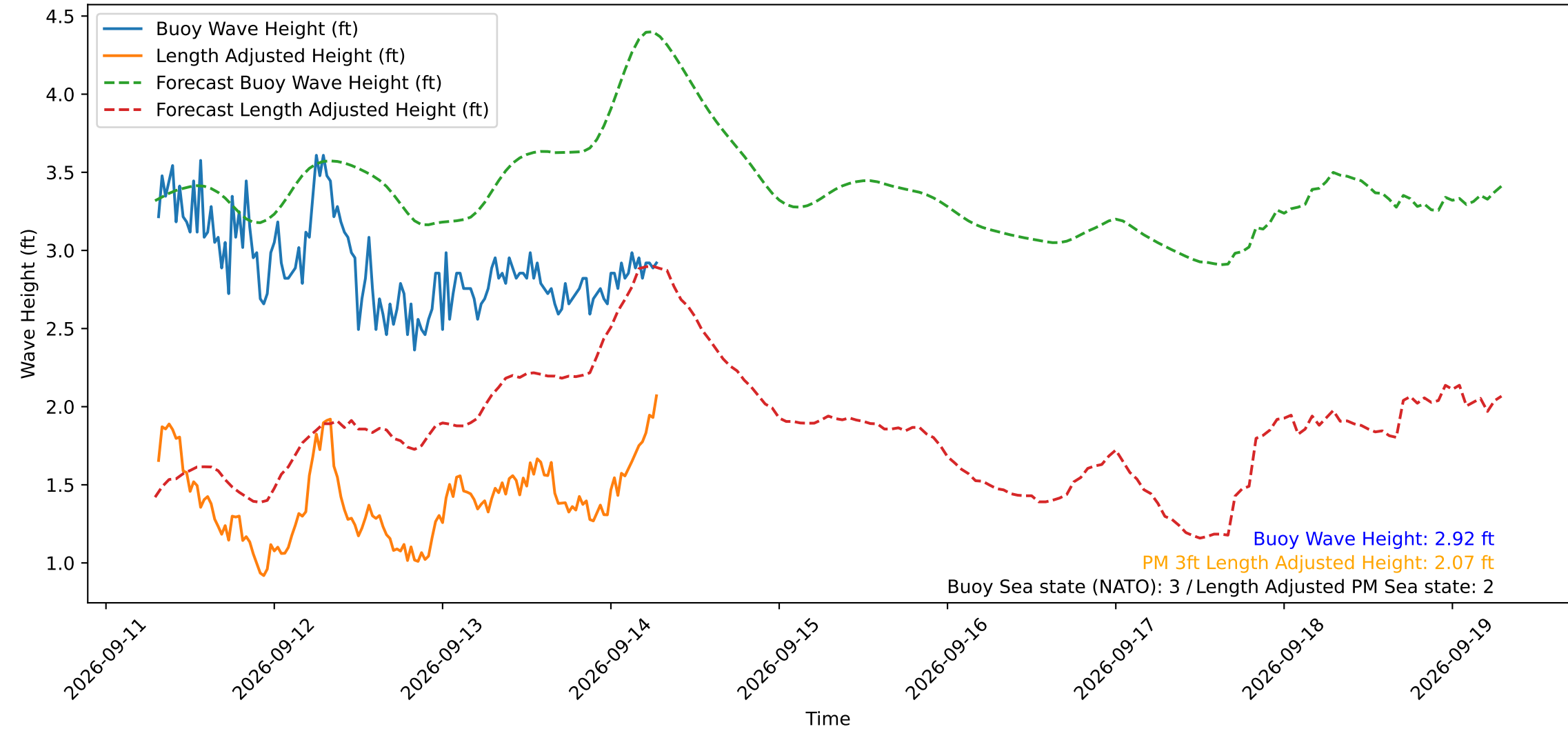
Wave Heights over Time for Green Beach at 2026-09-14 07:21:14
