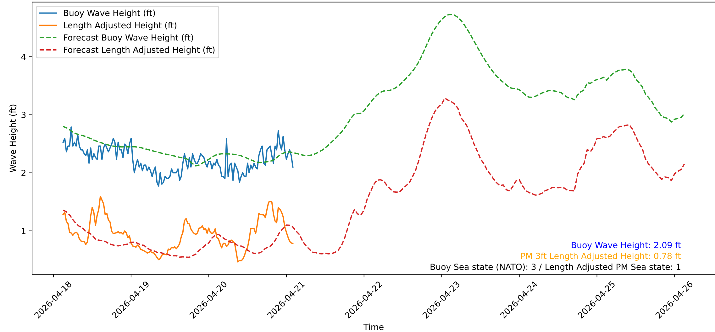
Wave Heights over Time for Red Beach at 2026-04-21 02:40:51
