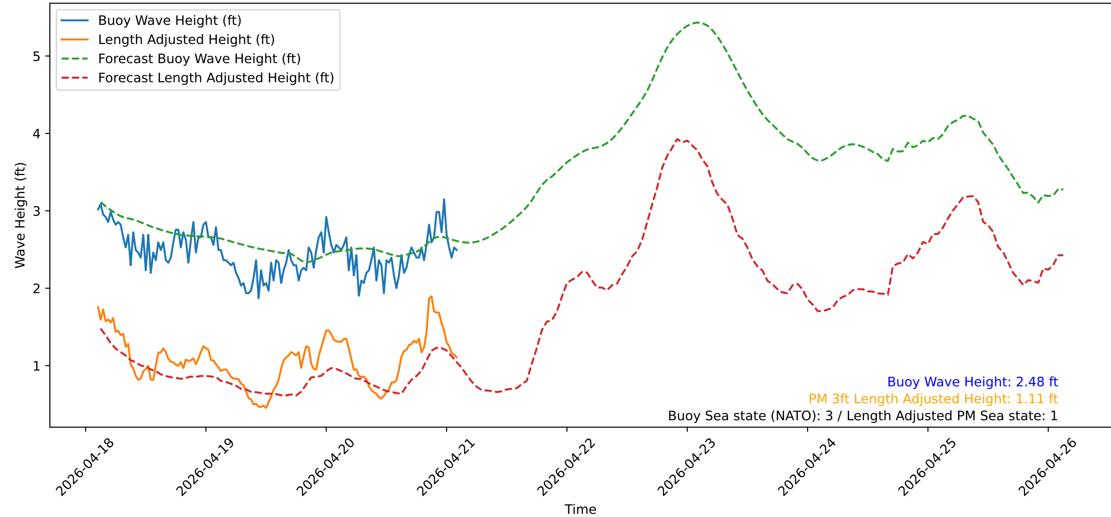
Wave Heights over Time for Green Beach at 2026-04-21 02:41:13
