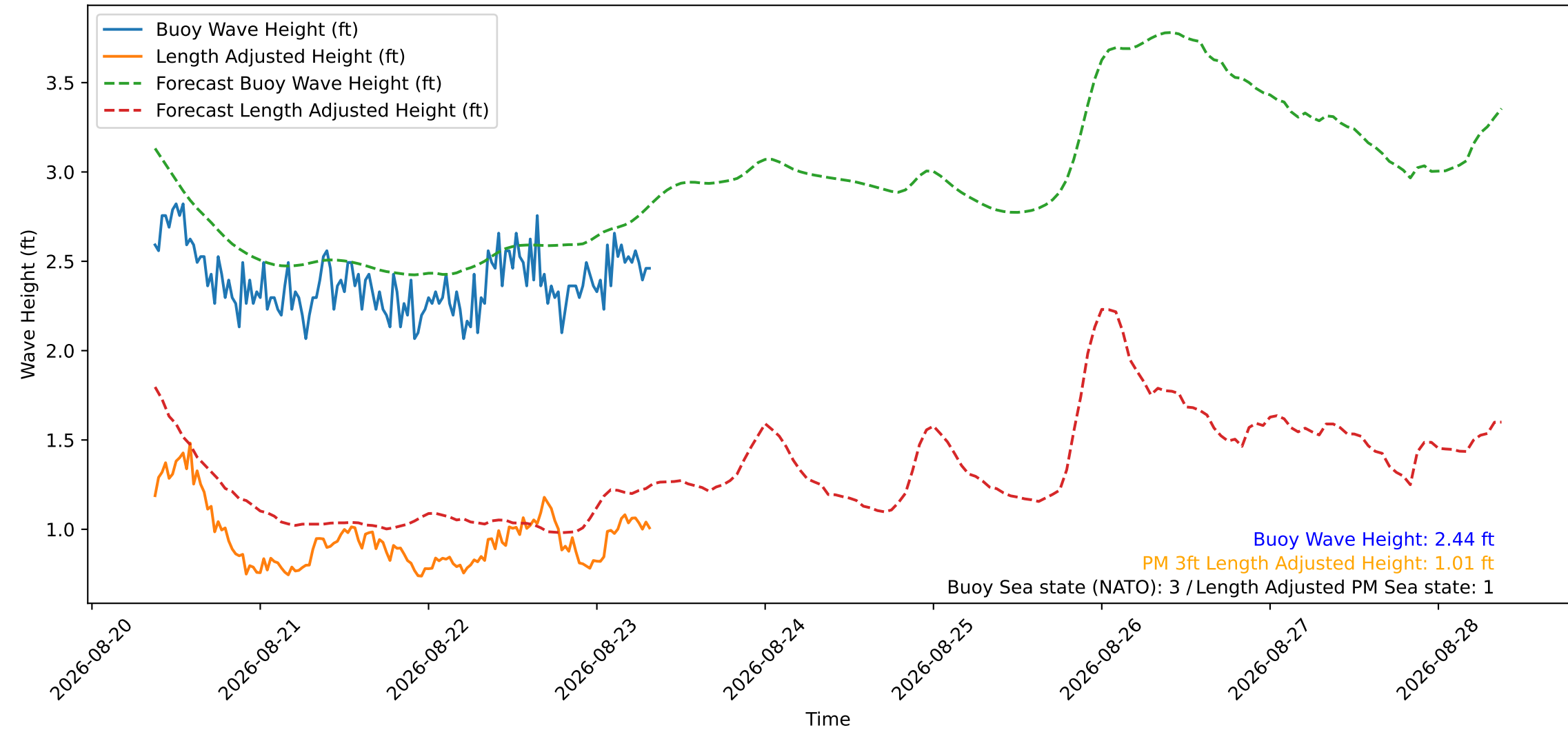
Wave Heights over Time for Red Beach at 2026-08-23 08:30:49
