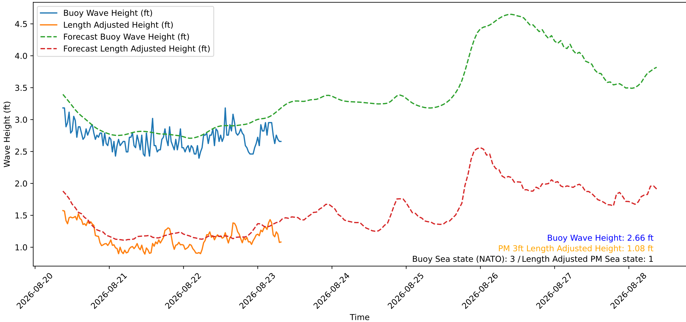
Wave Heights over Time for Green Beach at 2026-08-23 08:31:12
