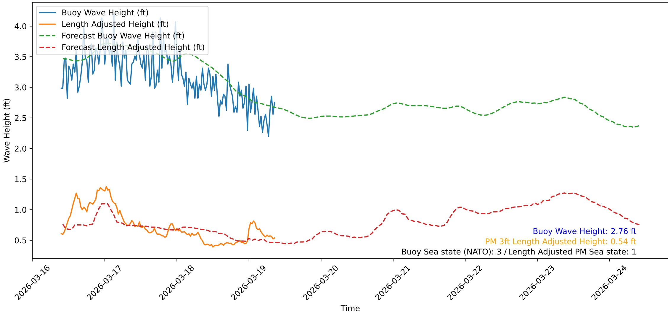
Wave Heights over Time for Green Beach at 2026-03-19 09:31:10
