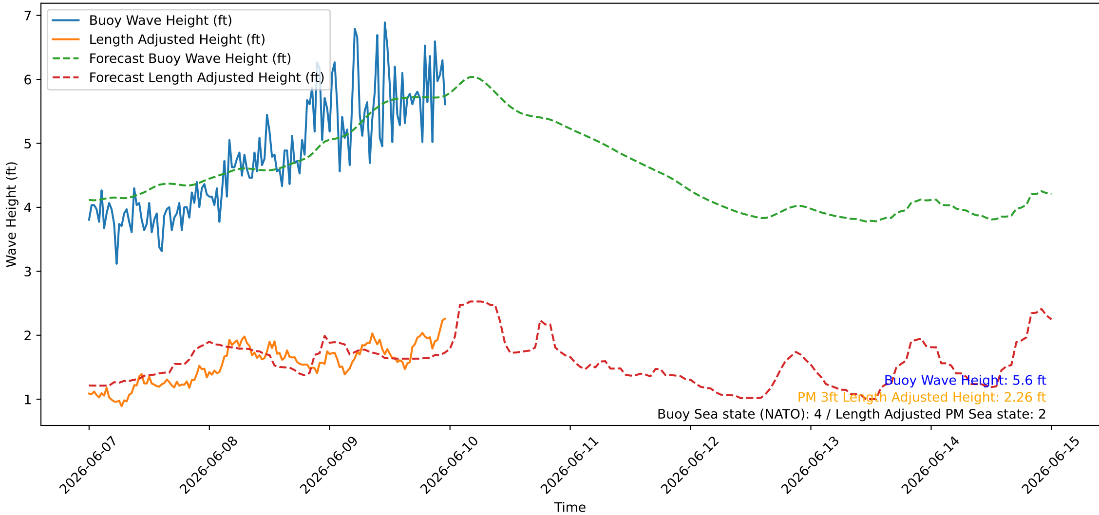
Wave Heights over Time for Green Beach at 2026-06-09 23:51:10
