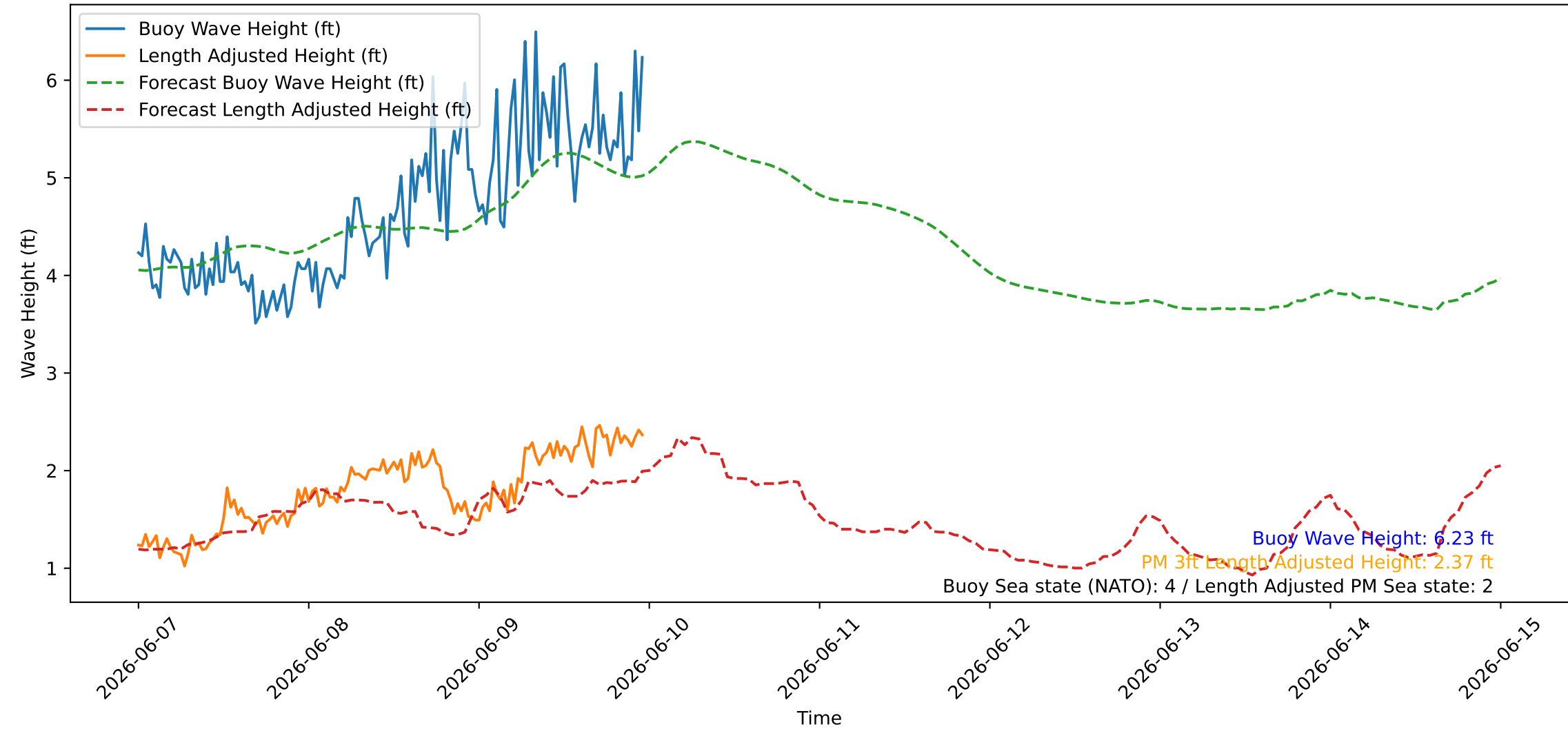
Wave Heights over Time for Oceanside Harbor at 2026-06-09 23:50:26
