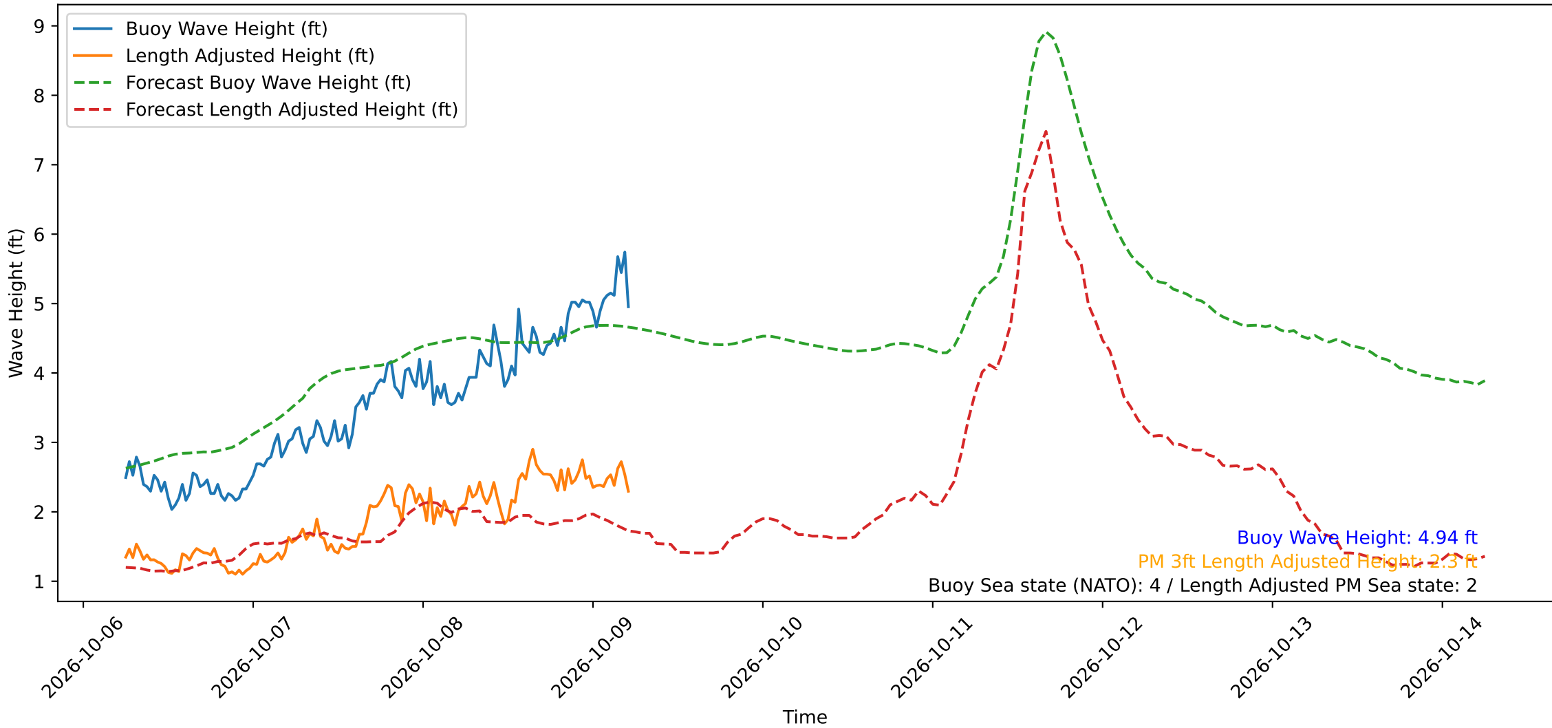
Wave Heights over Time for Oceanside Harbor at 2026-10-09 05:50:30
