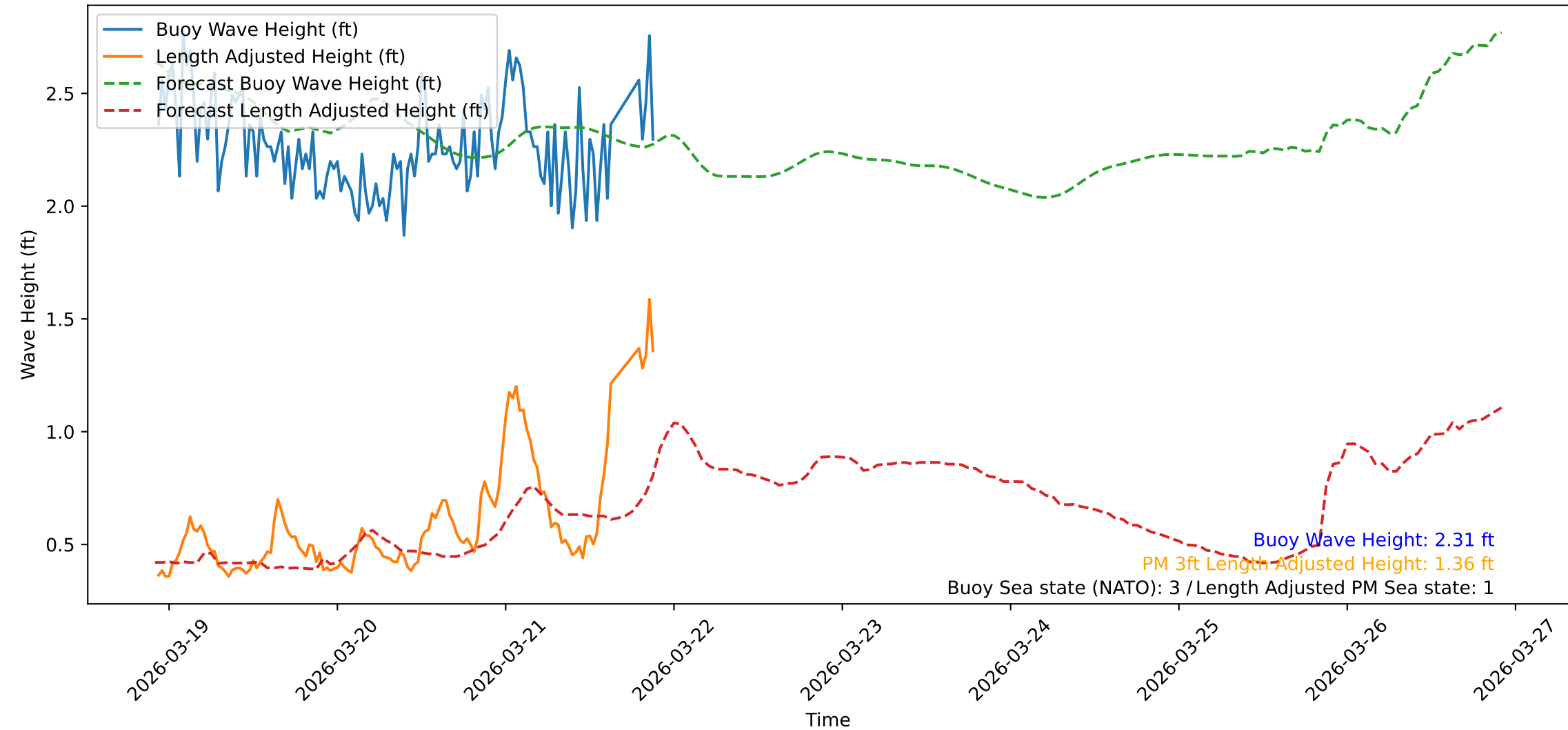
Wave Heights over Time for Red Beach at 2026-03-21 22:00:46
