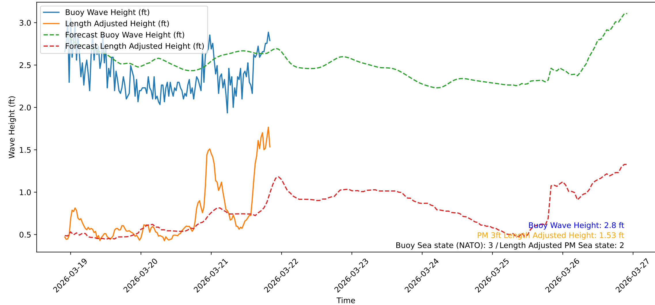
Wave Heights over Time for Green Beach at 2026-03-21 22:01:09
