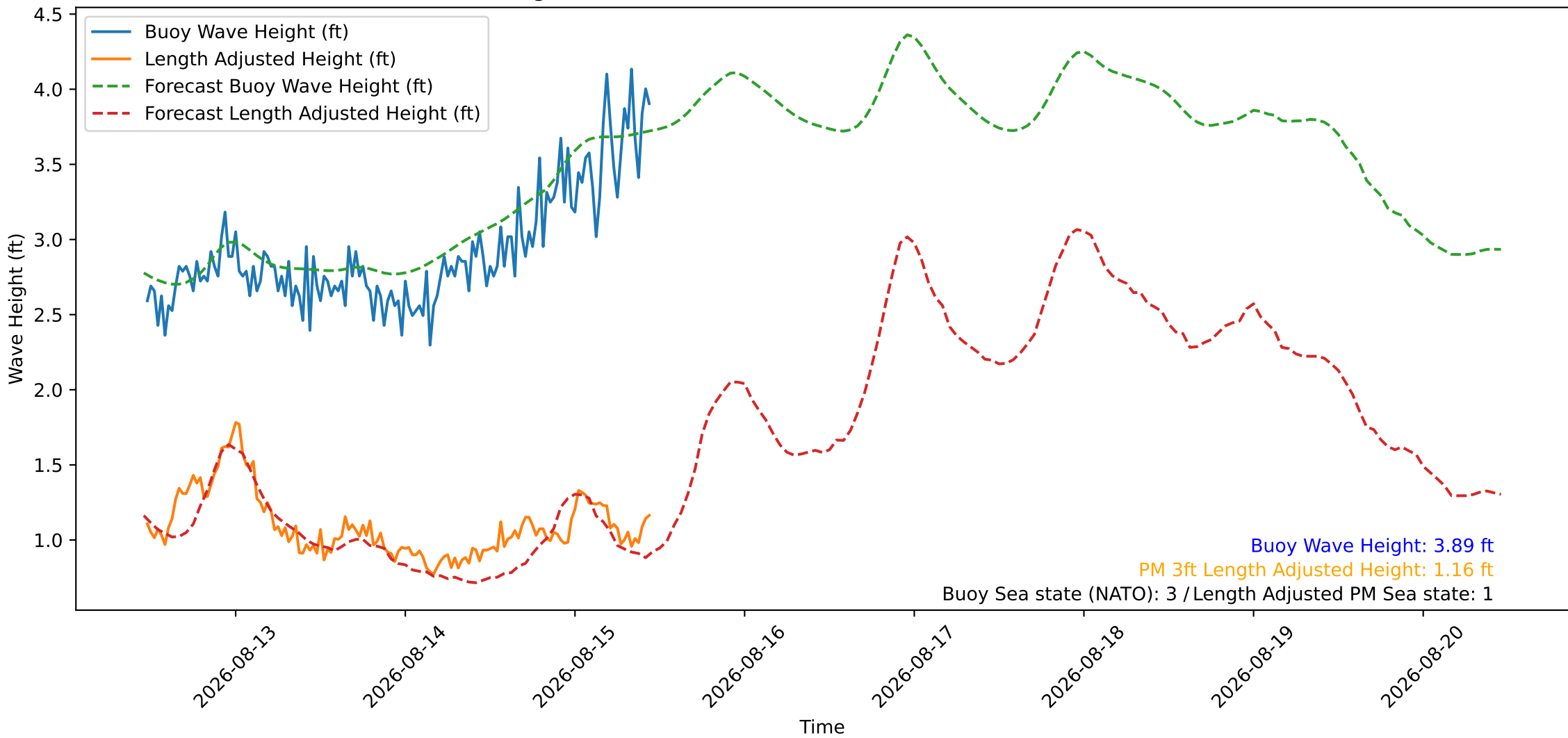
Wave Heights over Time for Oceanside Harbor at 2026-08-15 11:20:26
