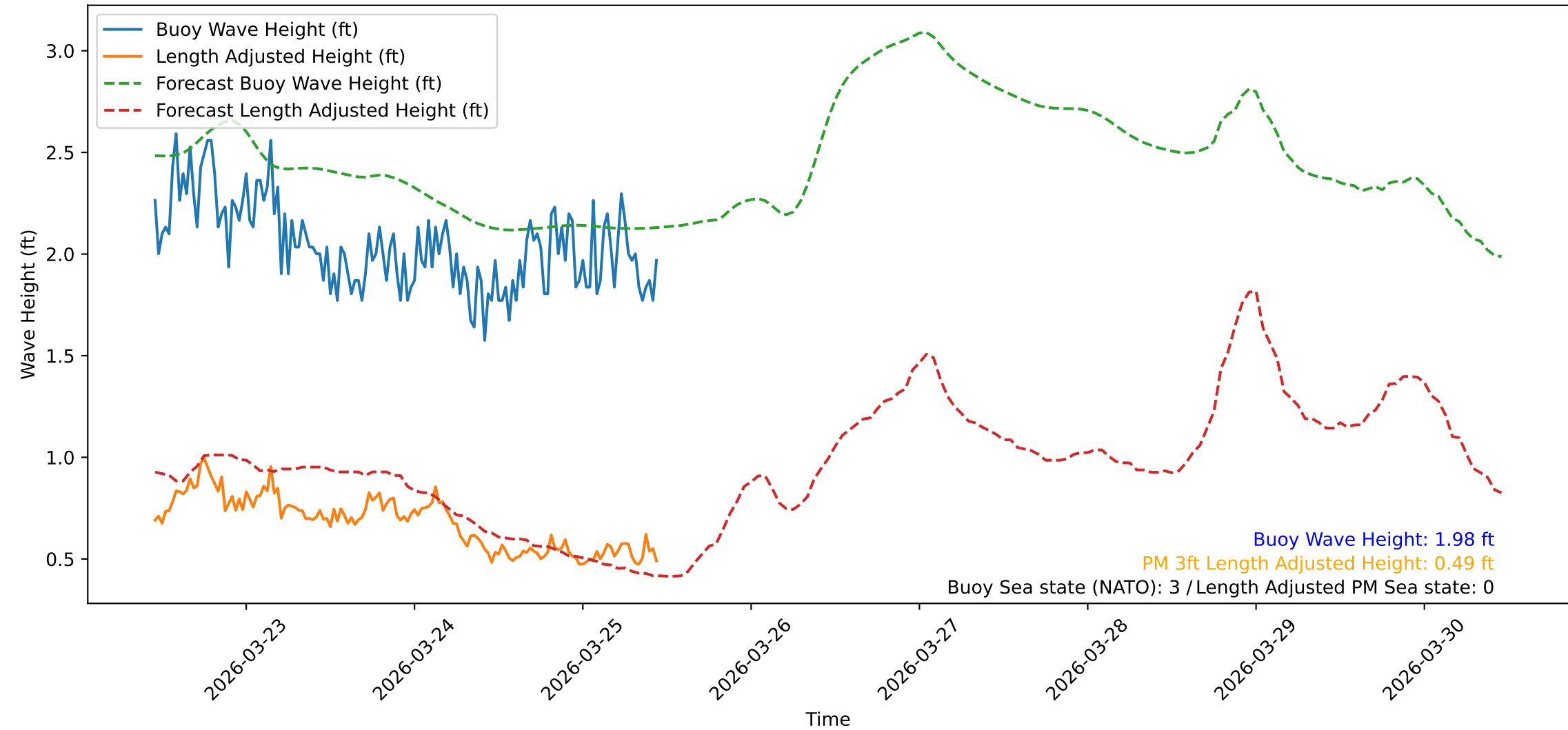
Wave Heights over Time for Oceanside Harbor at 2026-03-25 11:00:31
