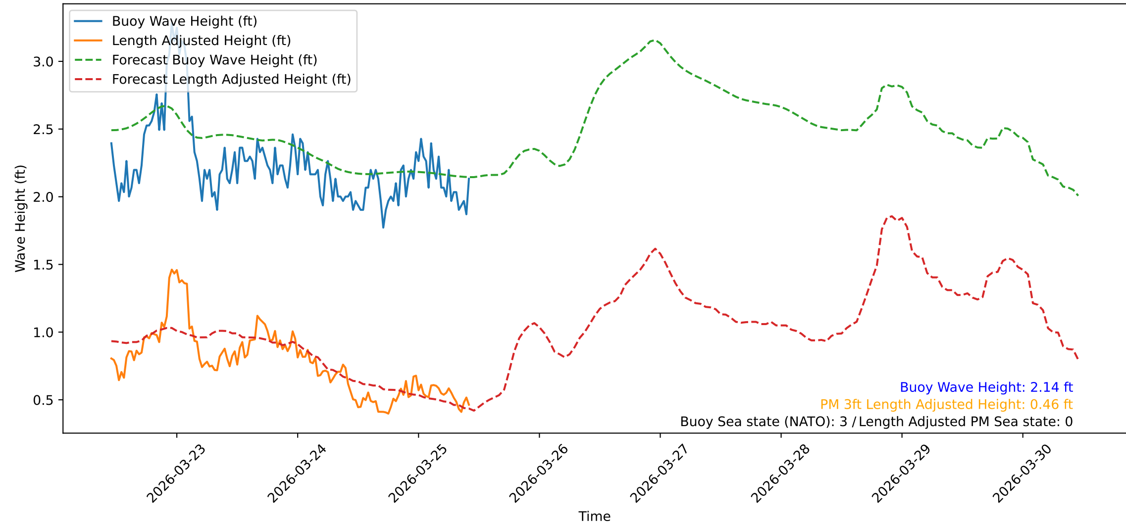
Wave Heights over Time for Green Beach at 2026-03-25 11:01:09
