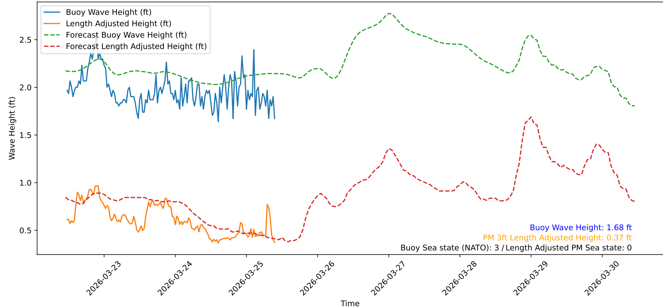
Wave Heights over Time for Red Beach at 2026-03-25 11:00:47
