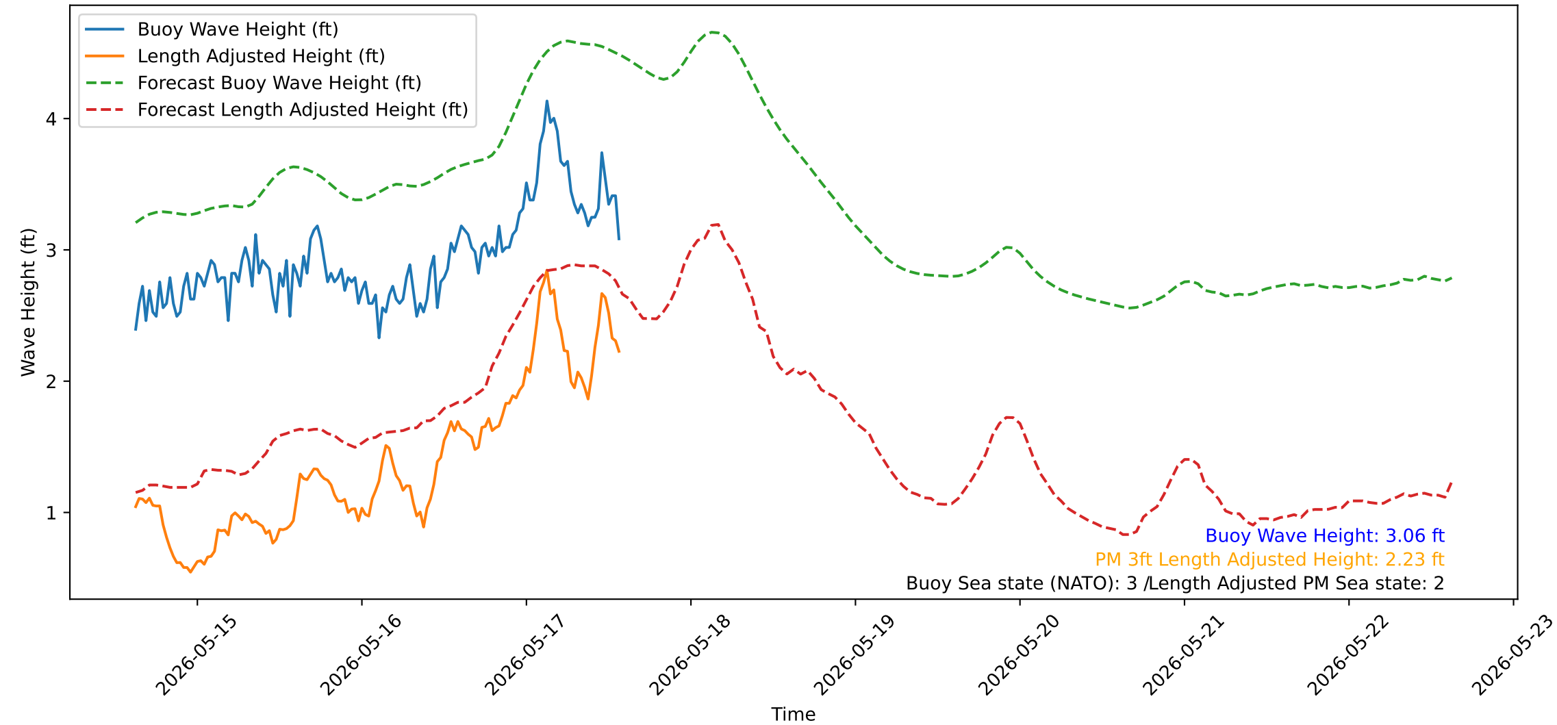
Wave Heights over Time for Red Beach at 2026-05-17 14:40:51
