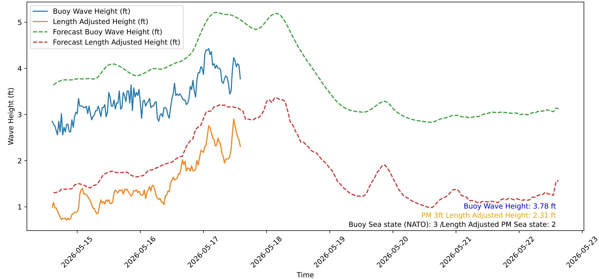
Wave Heights over Time for Green Beach at 2026-05-17 14:41:14
