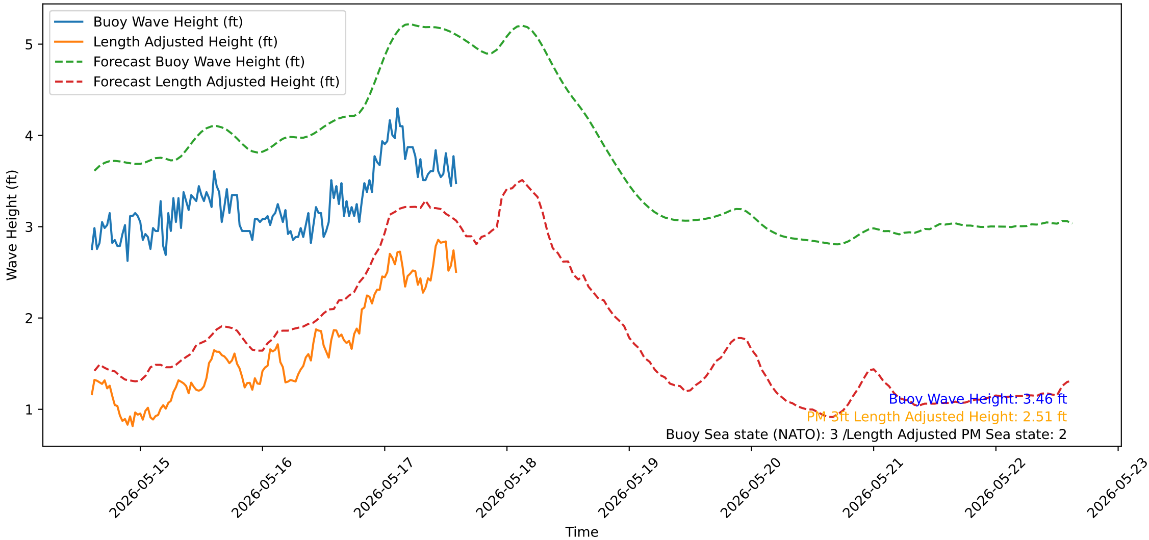
Wave Heights over Time for Oceanside Harbor at 2026-05-17 14:40:32
