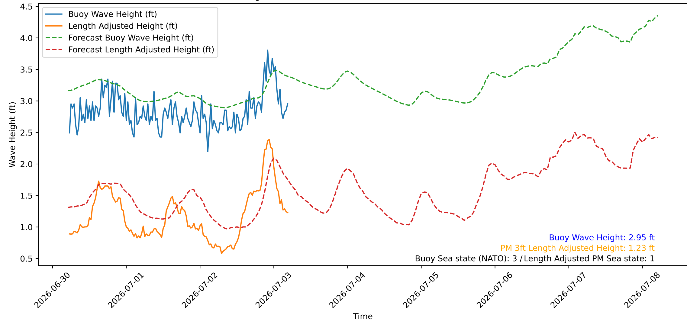
Wave Heights over Time for Red Beach at 2026-07-03 05:10:45
