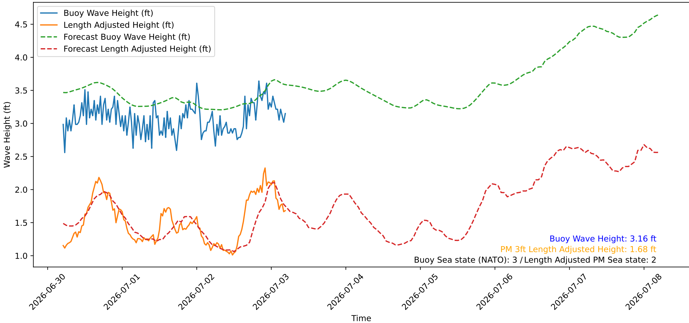
Wave Heights over Time for Oceanside Harbor at 2026-07-03 05:10:26
