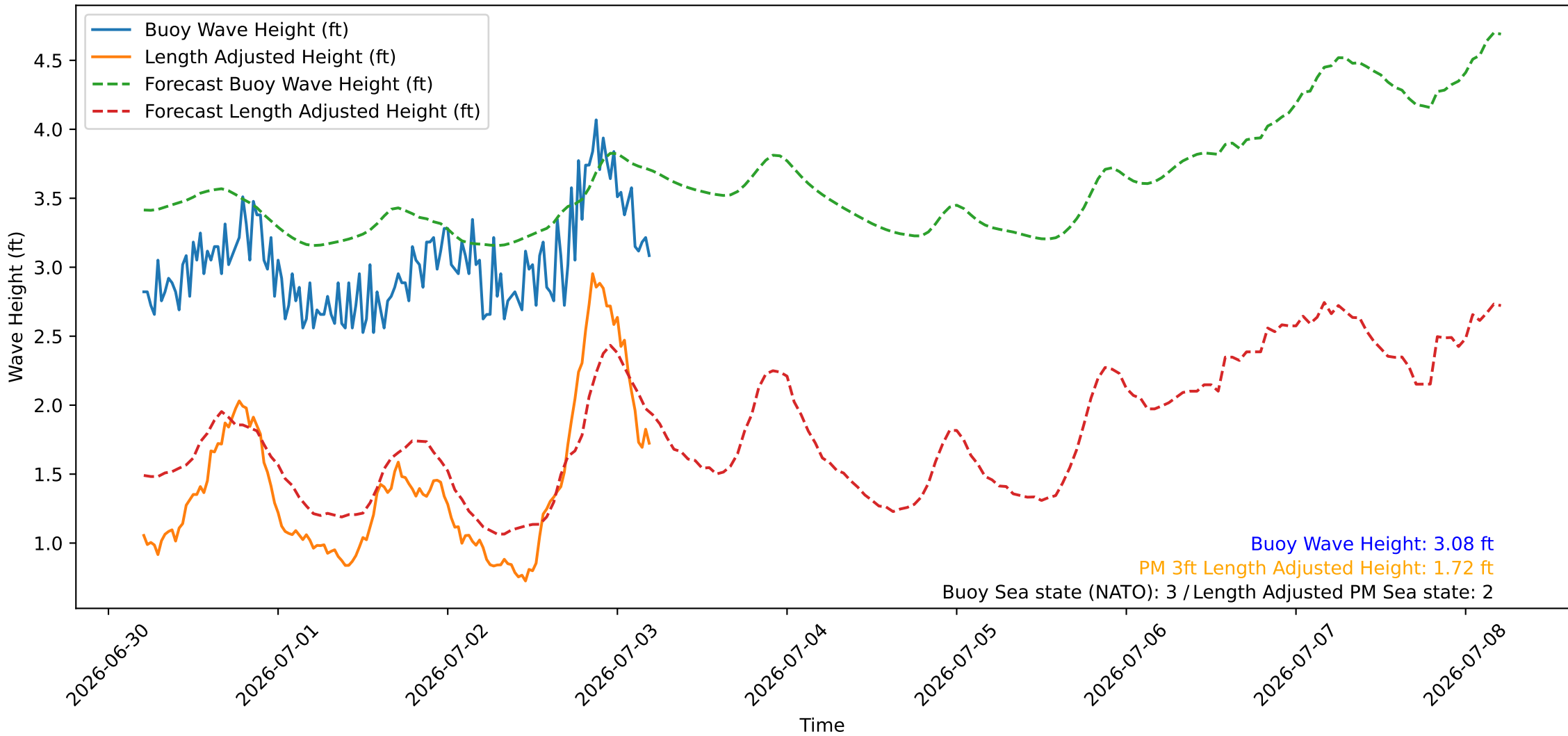
Wave Heights over Time for Green Beach at 2026-07-03 05:11:07
