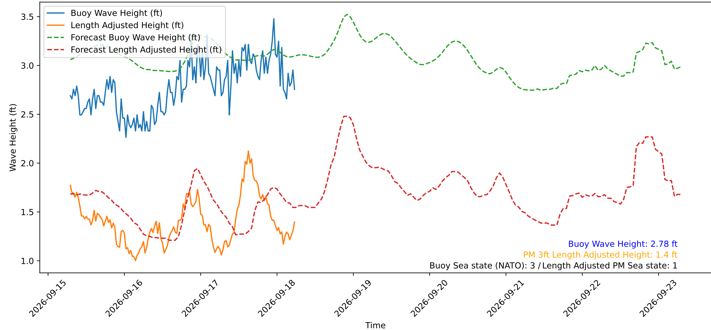
Wave Heights over Time for Green Beach at 2026-09-18 06:31:12
