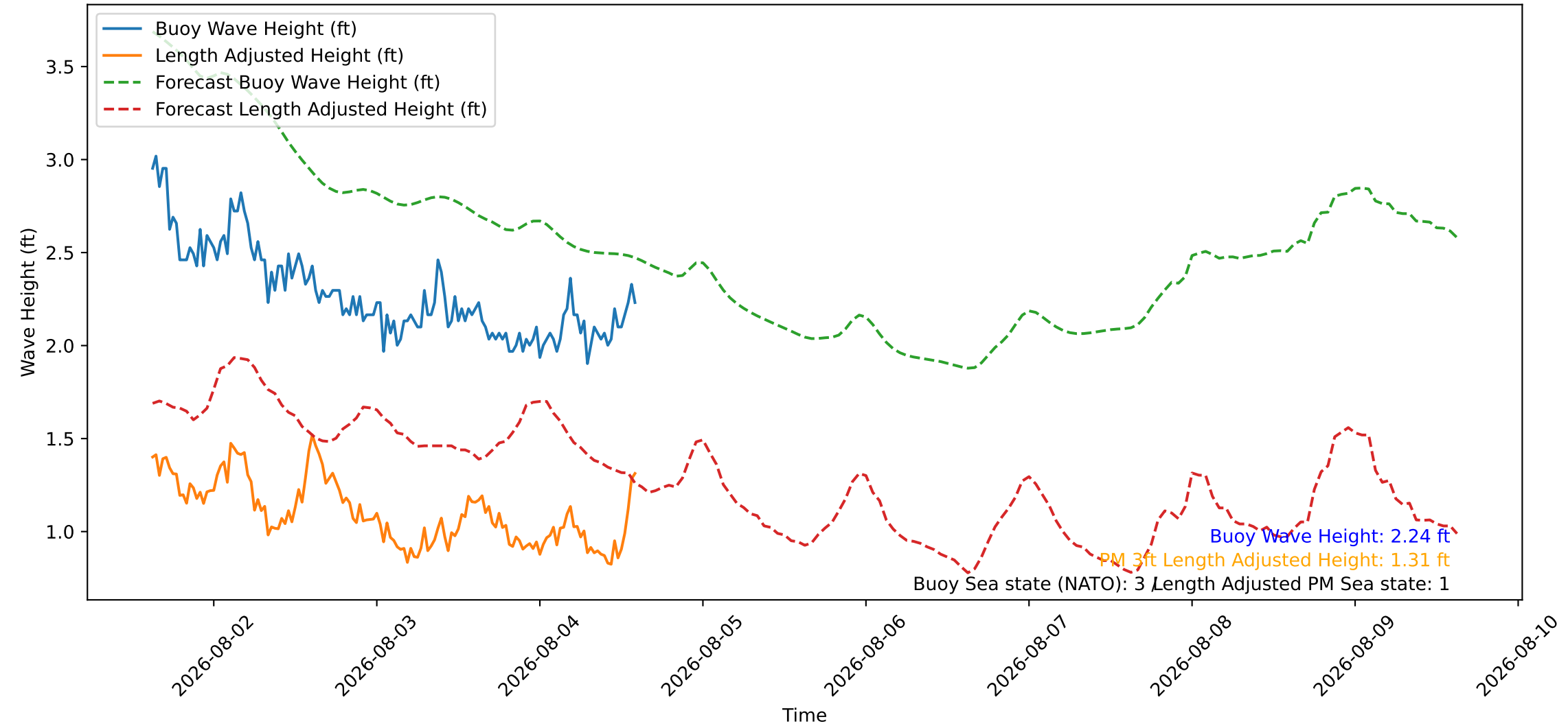
Wave Heights over Time for Red Beach at 2026-08-04 14:50:47
