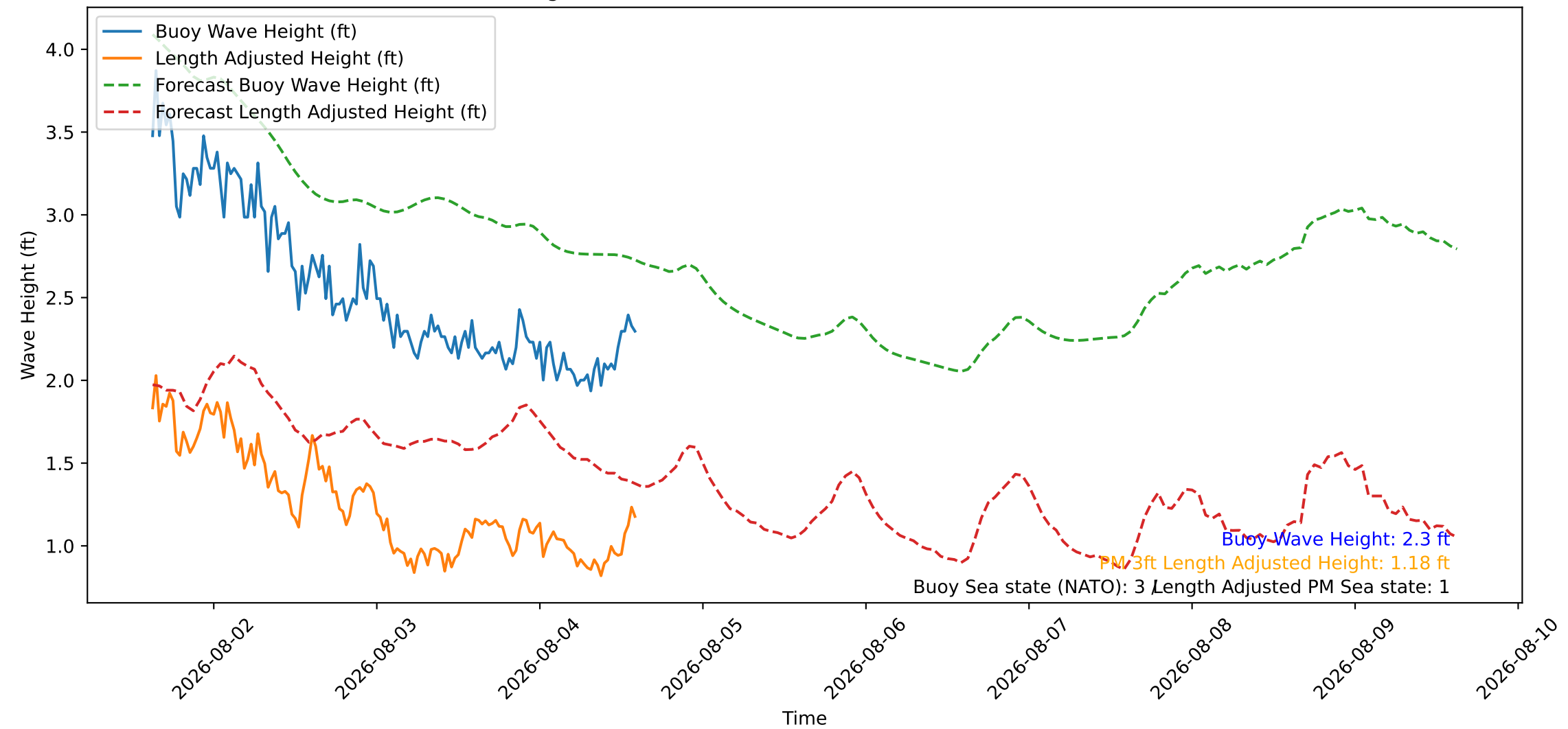
Wave Heights over Time for Green Beach at 2026-08-04 14:51:09
