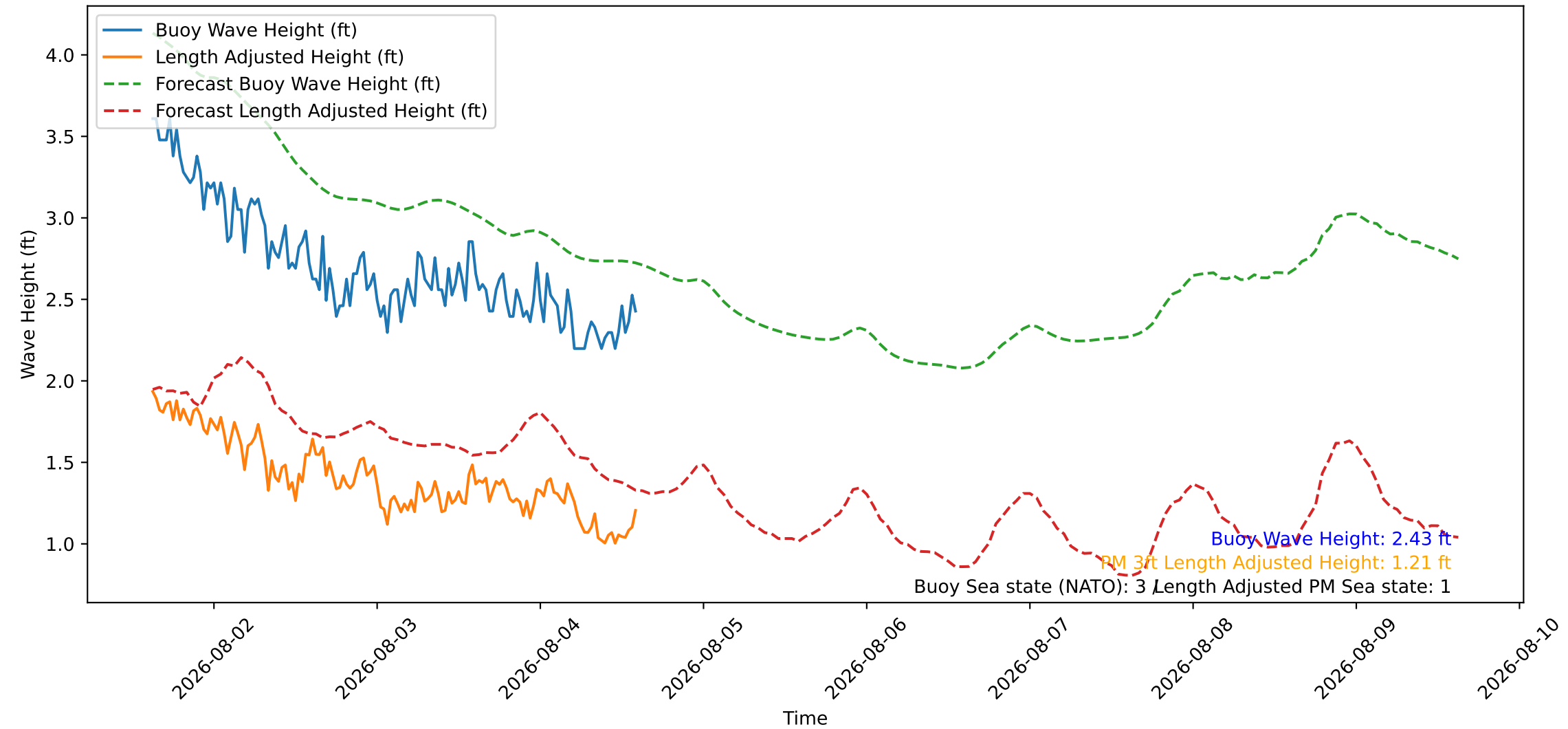
Wave Heights over Time for Oceanside Harbor at 2026-08-04 14:50:26
