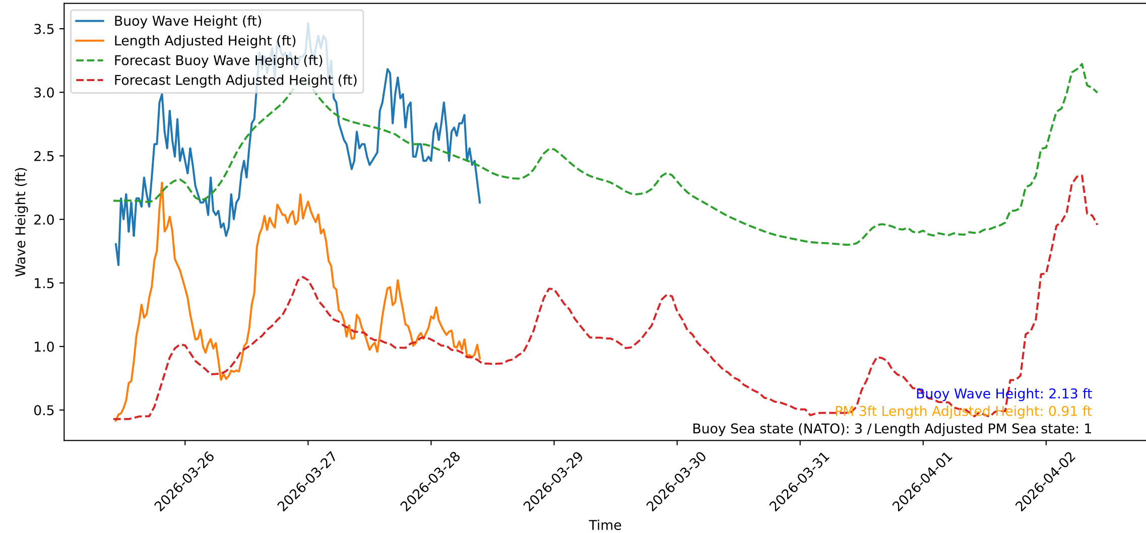
Wave Heights over Time for Green Beach at 2026-03-28 10:21:10
