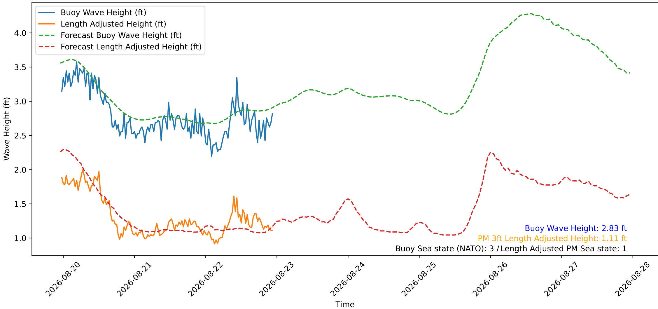
Wave Heights over Time for Oceanside Harbor at 2026-08-22 23:20:55
