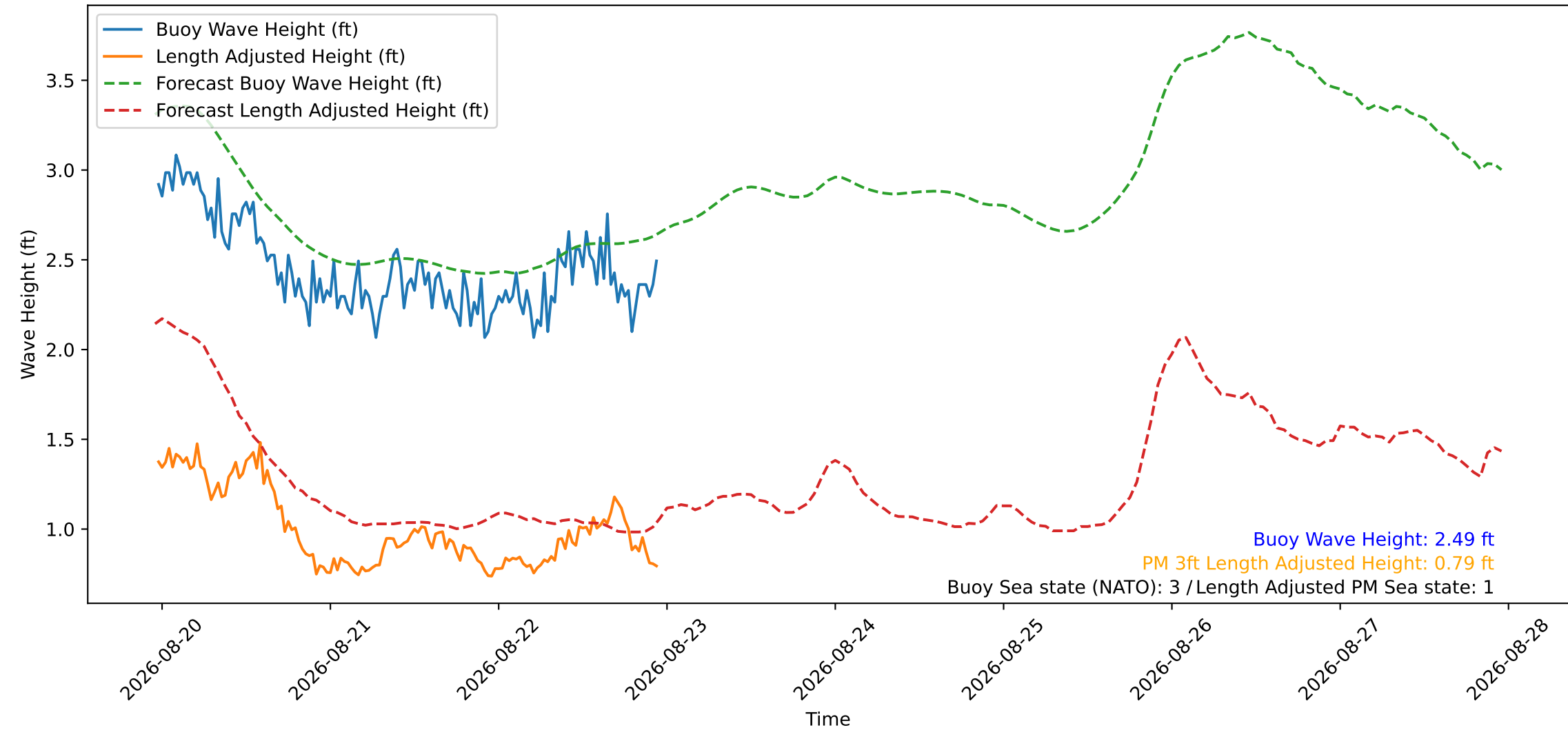
Wave Heights over Time for Red Beach at 2026-08-22 23:21:16
