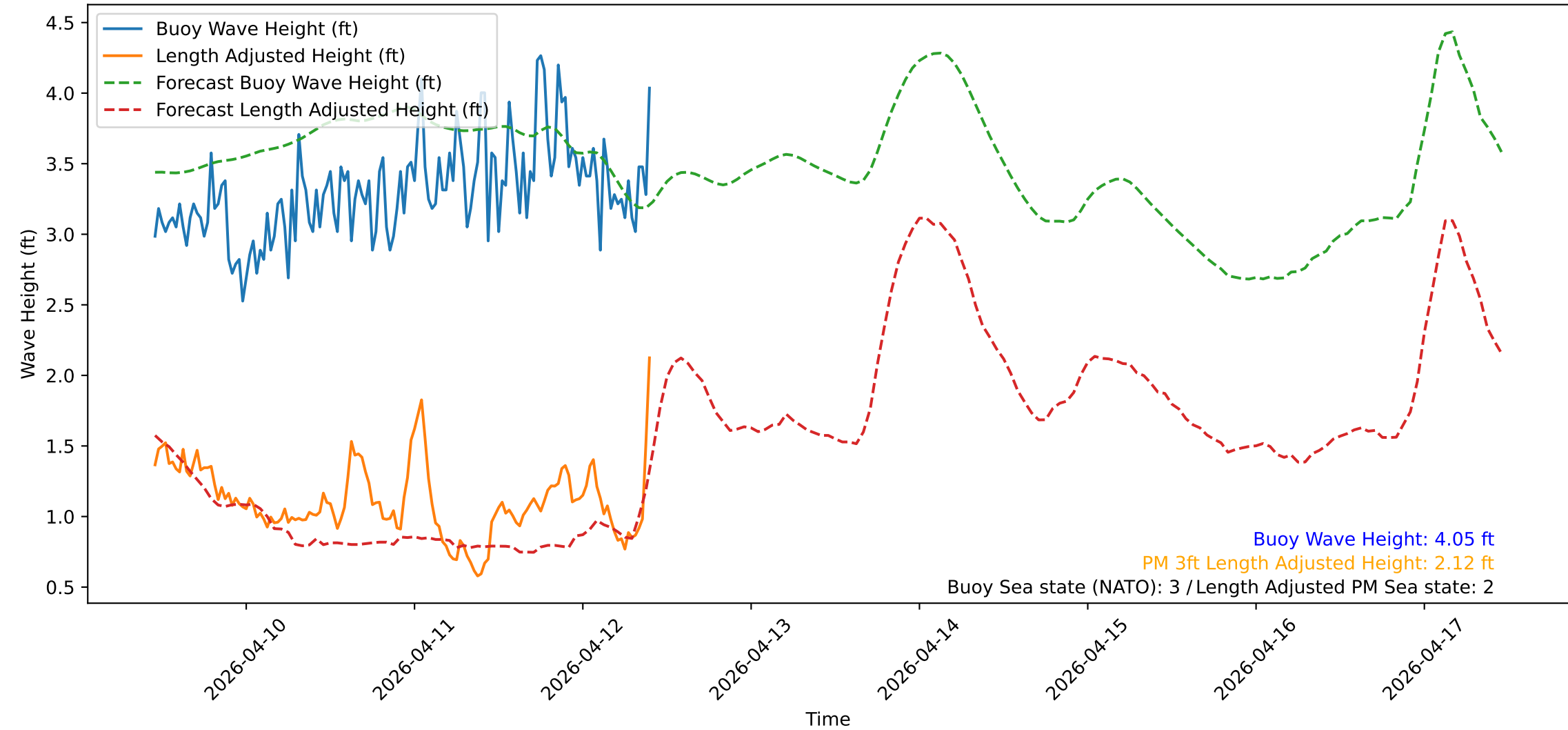
Wave Heights over Time for Red Beach at 2026-04-12 10:50:51
