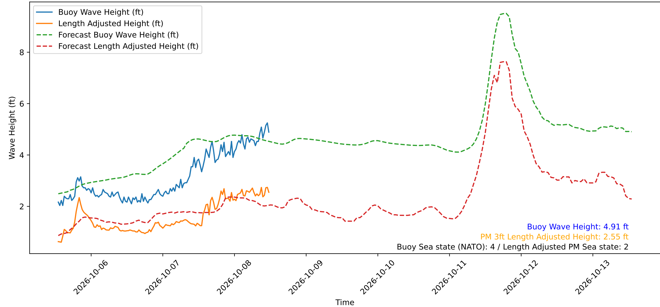
Wave Heights over Time for Green Beach at 2026-10-08 12:41:13
