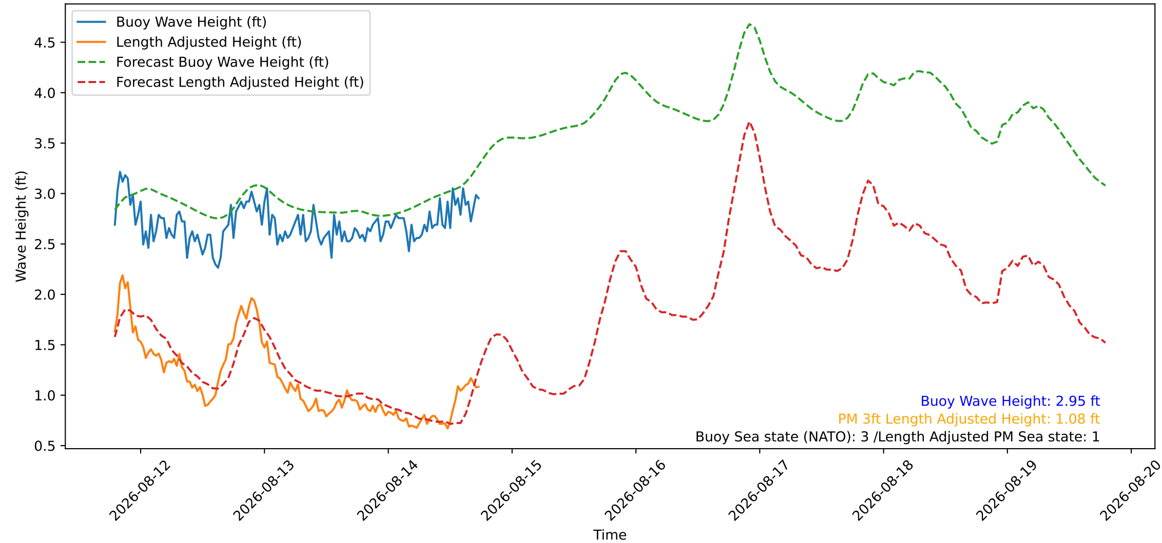
Wave Heights over Time for Green Beach at 2026-08-14 19:01:08
