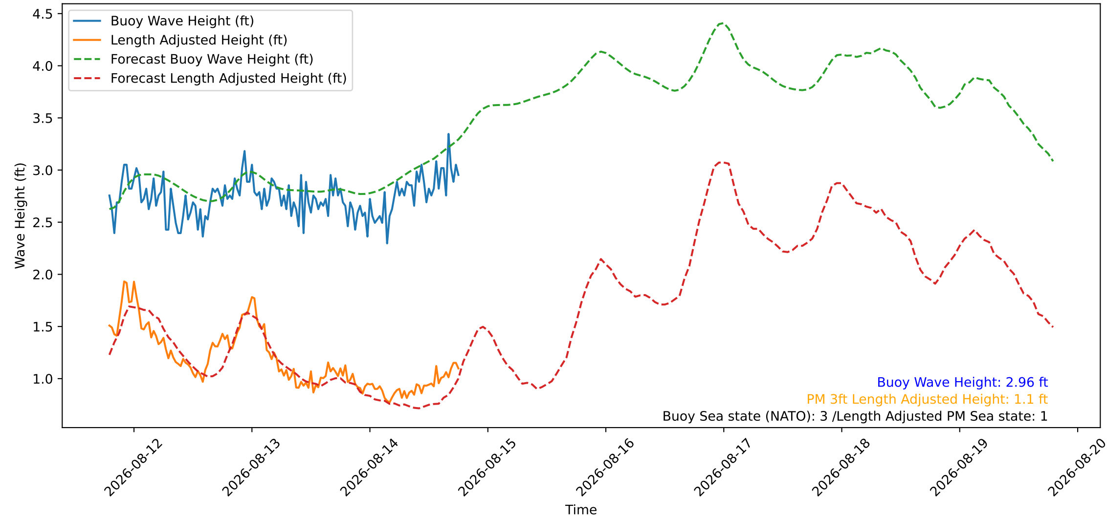
Wave Heights over Time for Oceanside Harbor at 2026-08-14 19:00:26
