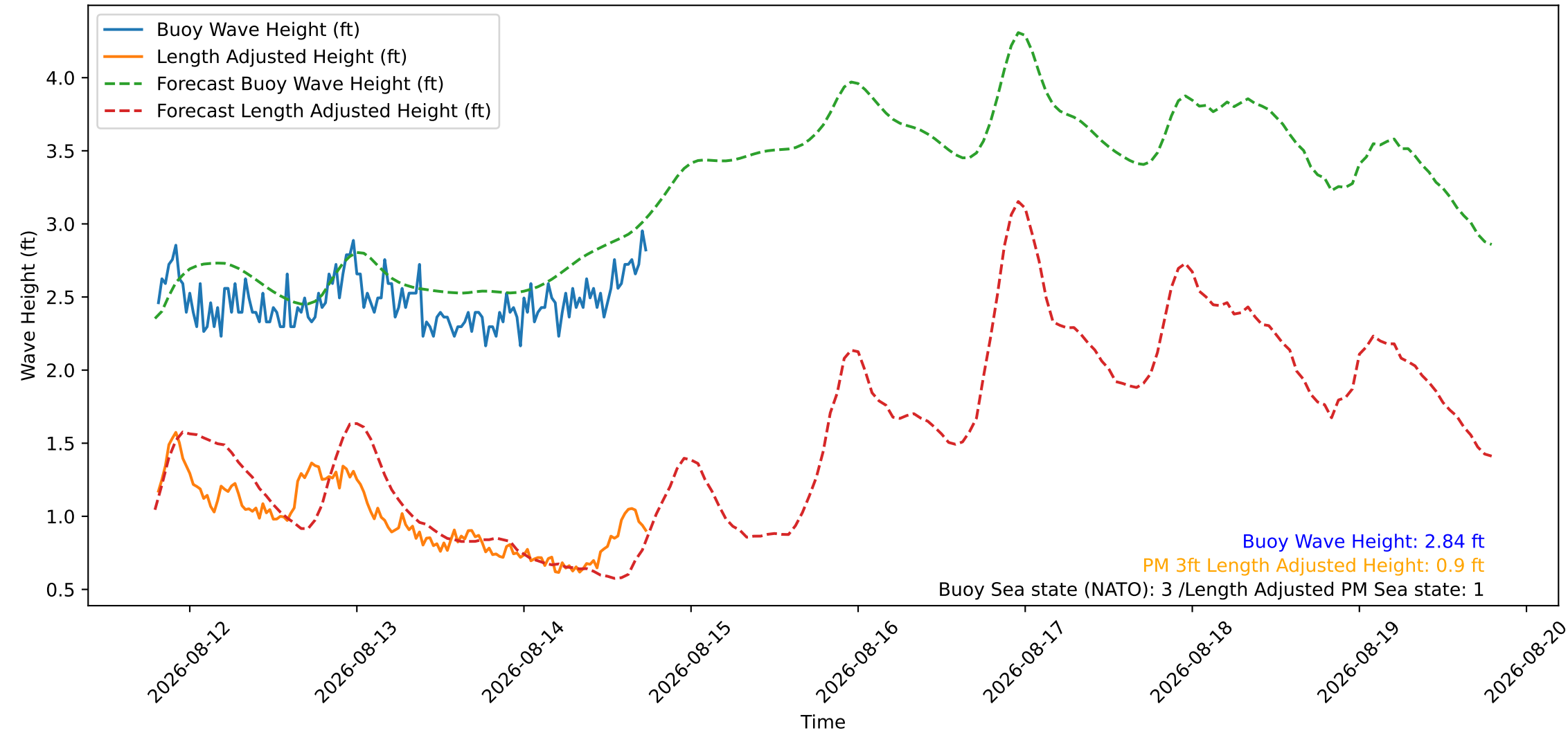
Wave Heights over Time for Red Beach at 2026-08-14 19:00:46
