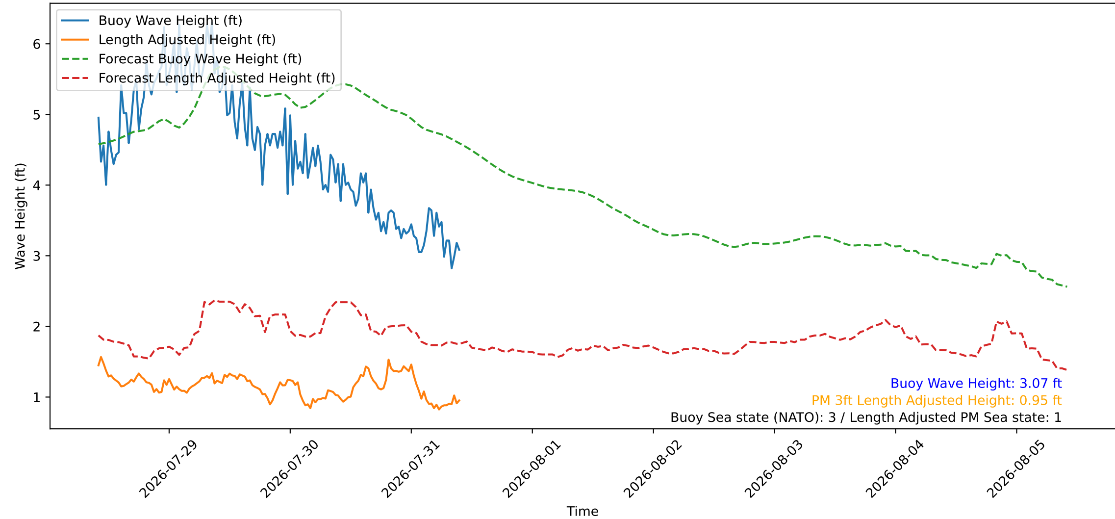
Wave Heights over Time for Green Beach at 2026-07-31 10:11:10
