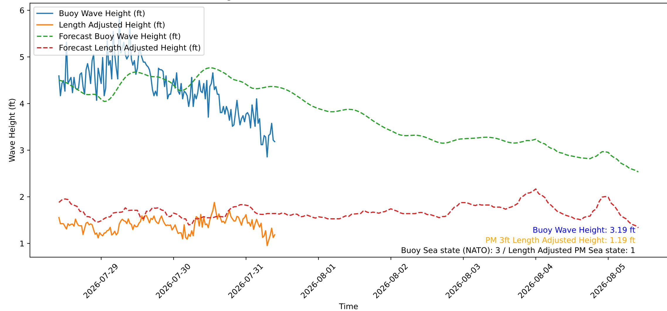
Wave Heights over Time for Oceanside Harbor at 2026-07-31 10:10:27
