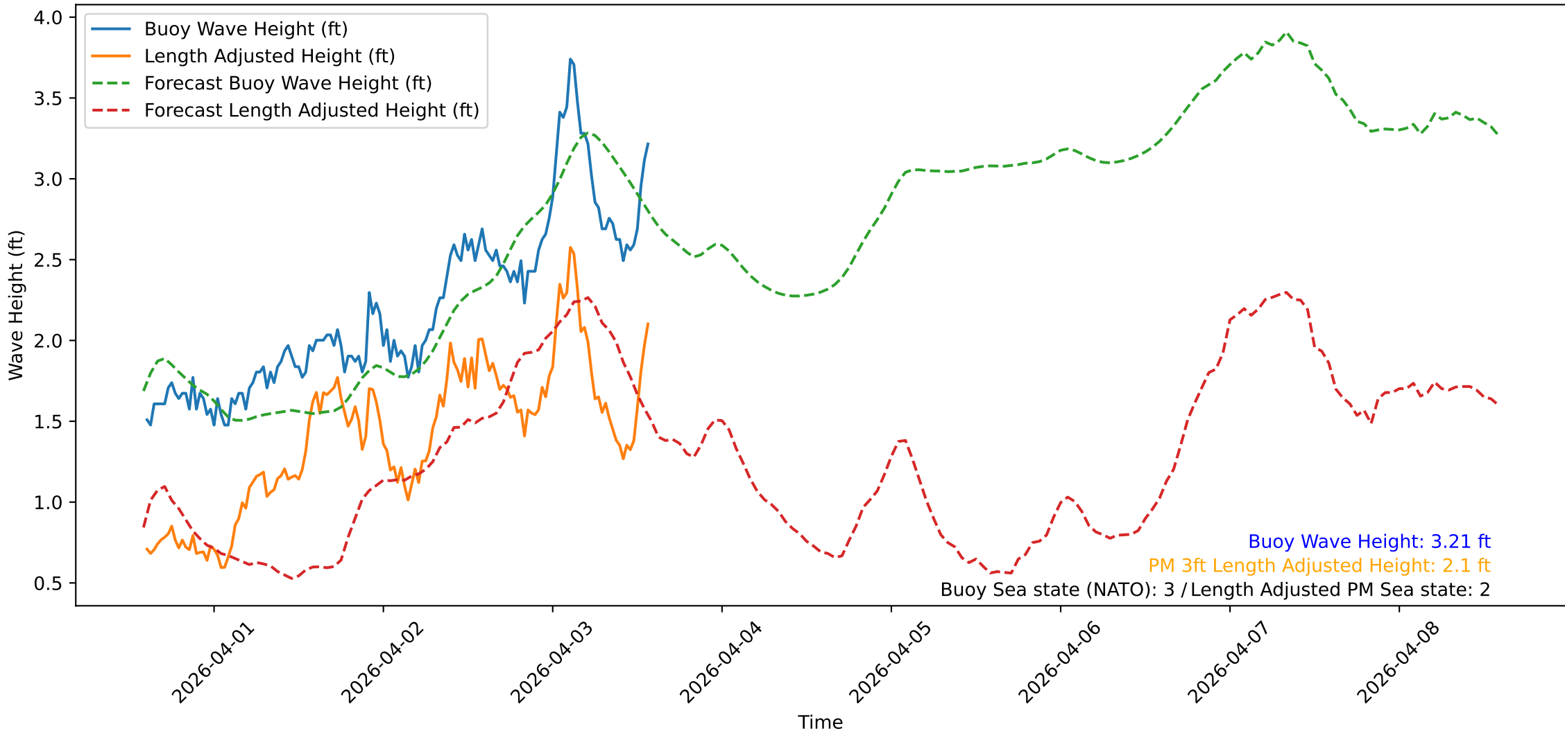
Wave Heights over Time for Red Beach at 2026-04-03 14:20:48
