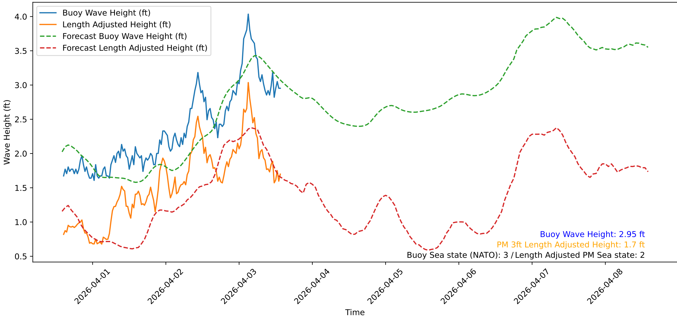
Wave Heights over Time for Oceanside Harbor at 2026-04-03 14:20:31
