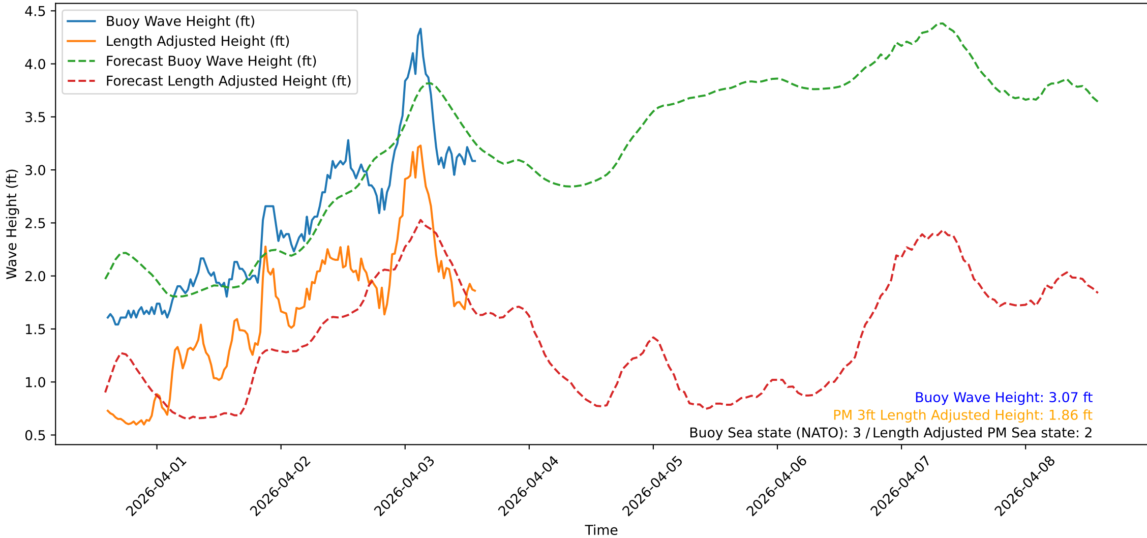
Wave Heights over Time for Green Beach at 2026-04-03 14:21:10
