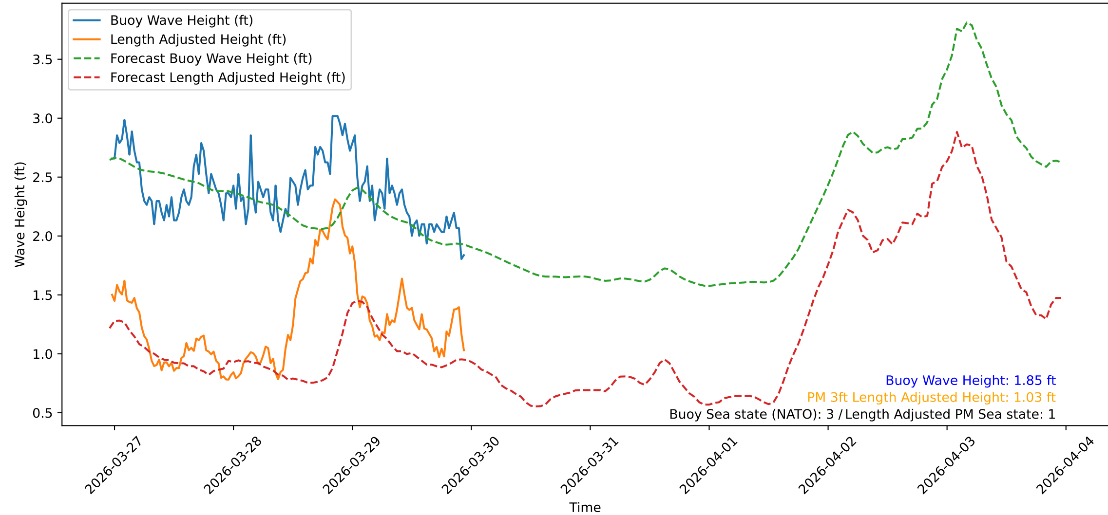
Wave Heights over Time for Red Beach at 2026-03-29 23:10:48
