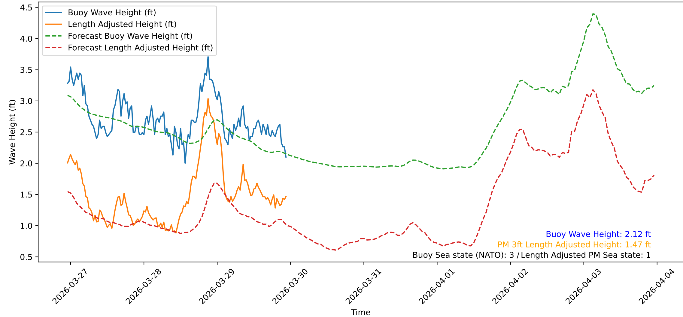
Wave Heights over Time for Green Beach at 2026-03-29 23:11:10
