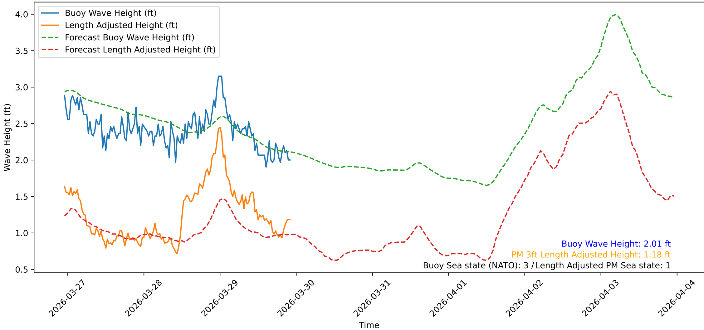
Wave Heights over Time for Oceanside Harbor at 2026-03-29 23:10:32
