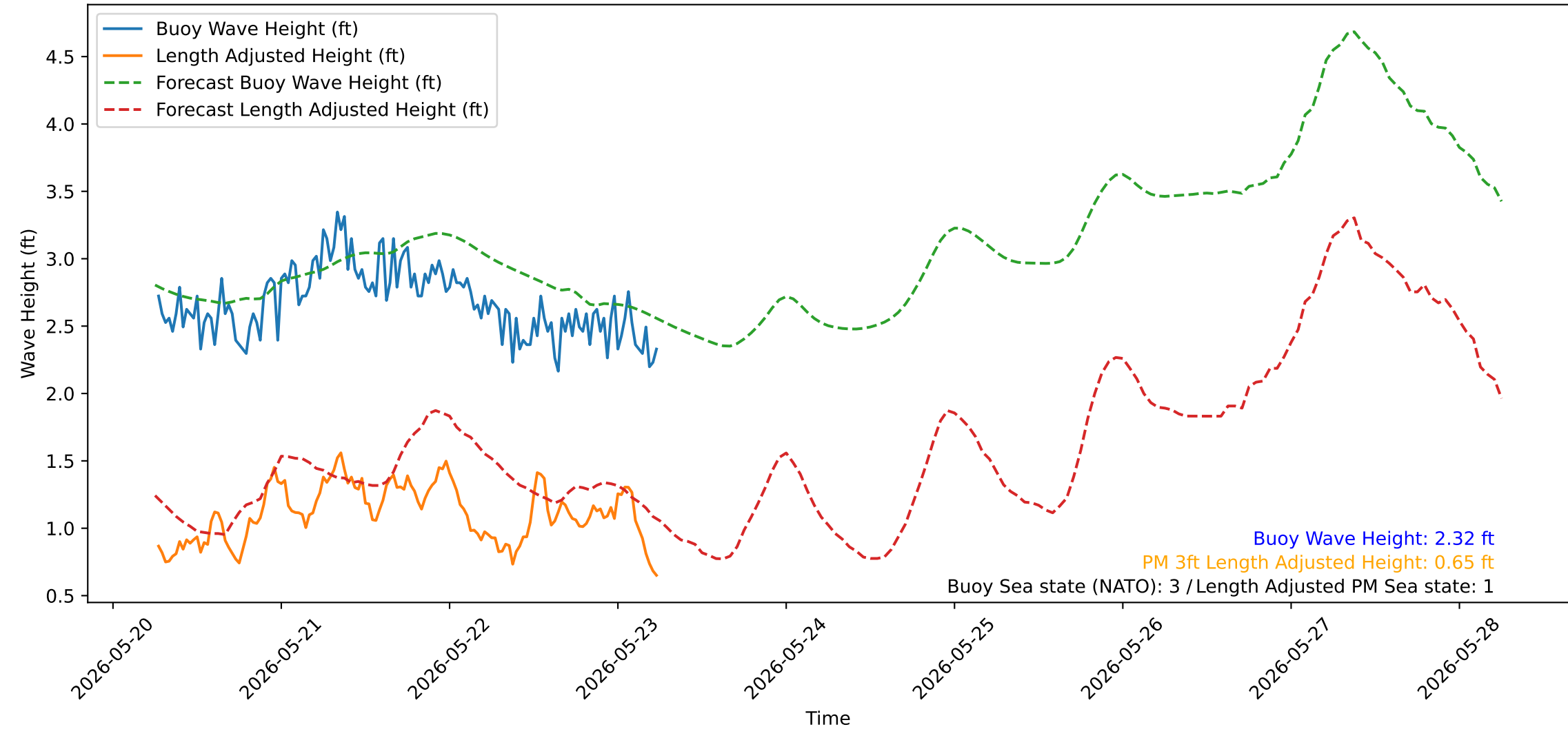
Wave Heights over Time for Red Beach at 2026-05-23 06:10:50
