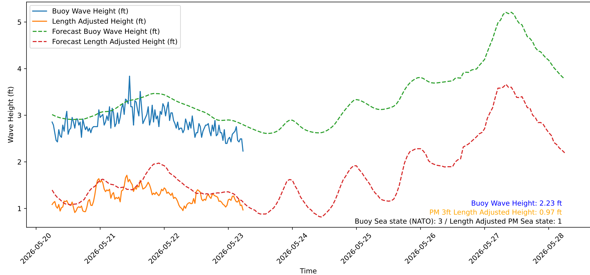
Wave Heights over Time for Oceanside Harbor at 2026-05-23 06:10:31
