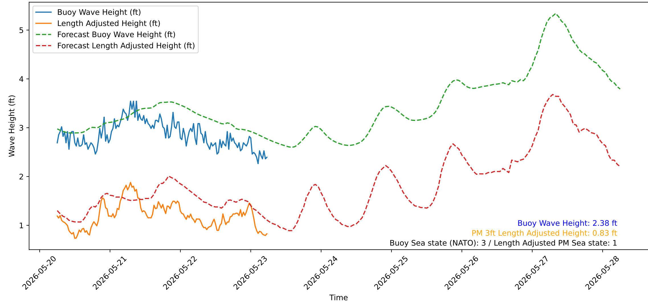
Wave Heights over Time for Green Beach at 2026-05-23 06:11:13
