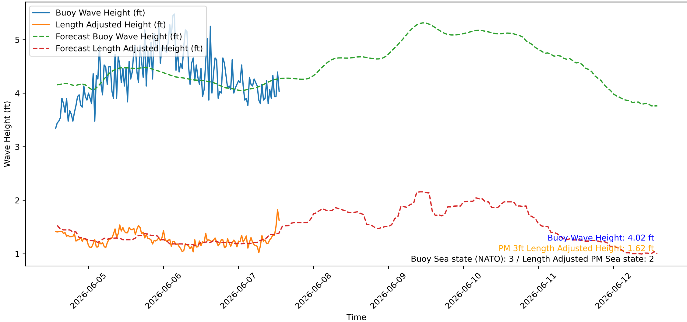
Wave Heights over Time for Oceanside Harbor at 2026-06-07 13:30:26
