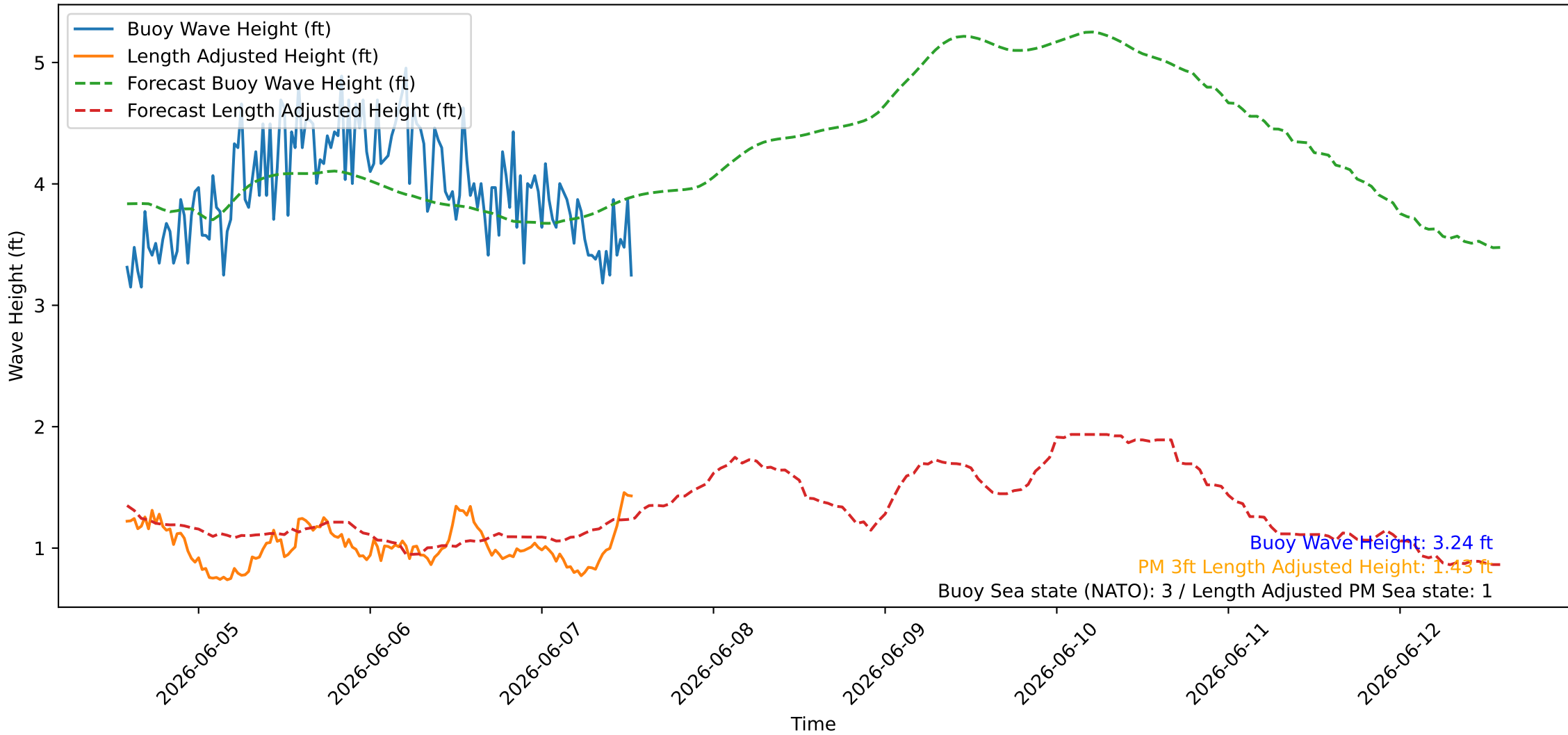
Wave Heights over Time for Red Beach at 2026-06-07 13:30:46
