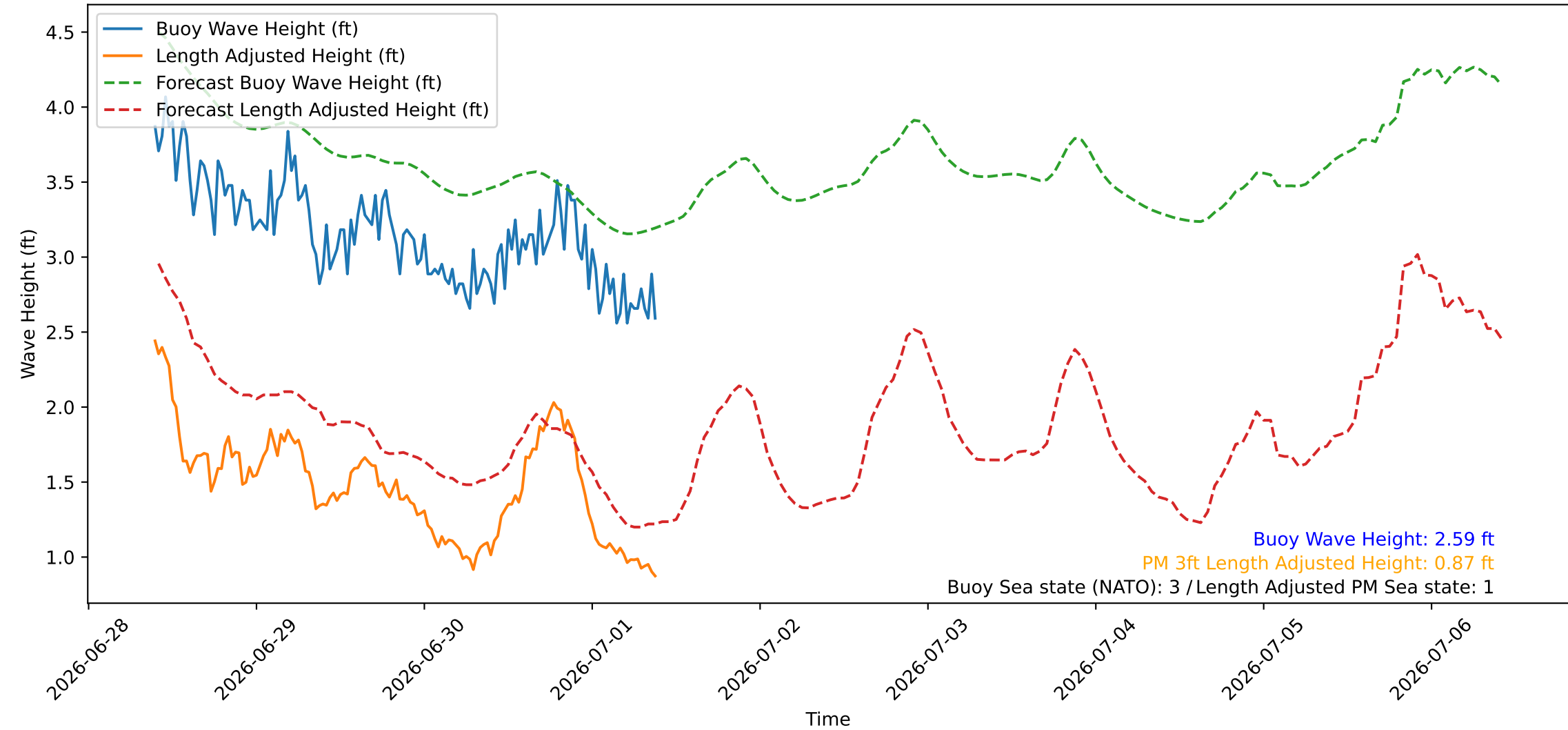
Wave Heights over Time for Green Beach at 2026-07-01 09:41:08
